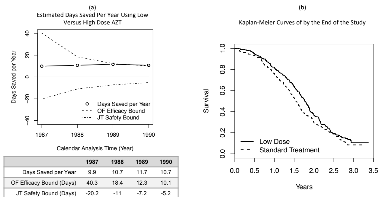
Figure 4. Figures in Example: (a) Estimated Days Saved Per Year Using Low Versus High Dose AZT; (b) Kaplan-Meier Curves of by the End of the Study
