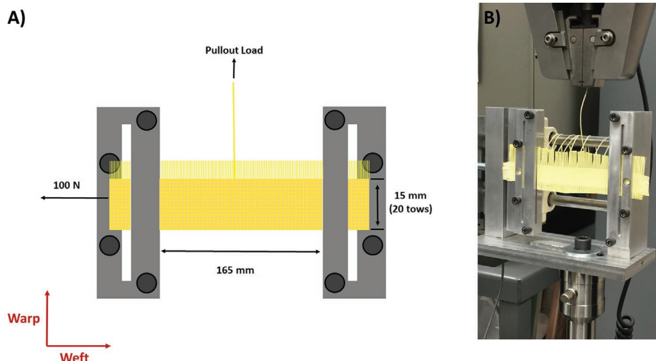
Figure 3. A) Schematic of experimental setup for tow pullout test. B) Treated aramid fabric sample for tow pullout.
