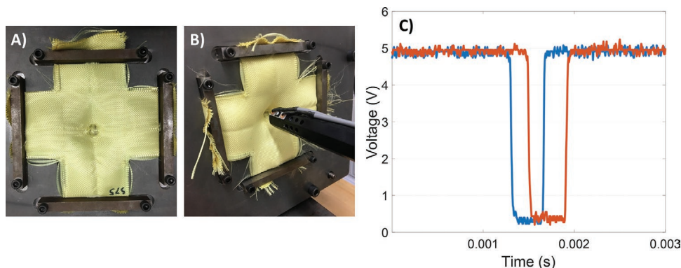
Figure 11. A) Cross-shaped, four-sided clamped aramid fabrics. B) Experimental setup using 0.25 in. distance between barrel and target. C) Photogates recorded signal as projectile exits the barrel.
