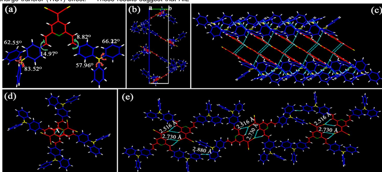
Fig. 2 Single crystal structure of TPA-DCM: (a) Molecular structure of TPA-DCM in crystal. (b) Crystal cell for TPA-DCM in b direction. (c) Molecular packing manner of TPA-DCM in c direction. (d) Intermolecular interactions of TPA-DCM, and (e).
