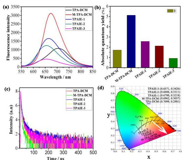
Fig. 5(a) The emission spectra of TPA-DCM, M-TPA-DCM and TPAIEs in solid state. (b) Absolute fluorescent quantum yield of TPA-DCM, M-TPA-DCM and TPAIEs in solid state. (c) The time-dependent fluorescence of TPA-DCM, M-TPA-DCM and TPAIEs. (d) CIE chromaticity diagram for TPA-DCM, M-TPA-DCM and TPAIEs
