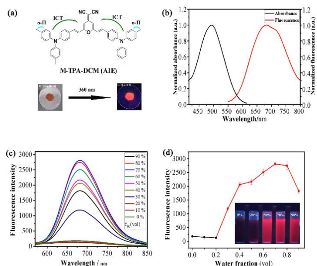
Fig. 1 (a) The molecular structure of M-TPA-DCM. (b) Normalized UV-Vis absorption and emission spectra of M-TPA-DCM in DMF solution. (c) Fluorescence emission spectra of M-TPA-DCM in water/DMF mixtures with various water fractions f_w . (d) Plot of maximum intensity of M-TPA-DCM versus water fraction in water/DMF mixed solvent. ( [M-TPA-DCM] = 10^{-5} M, \lambda_{ex} = 485 nm, speed: 2400 nm/min, slit: 5/5.)
