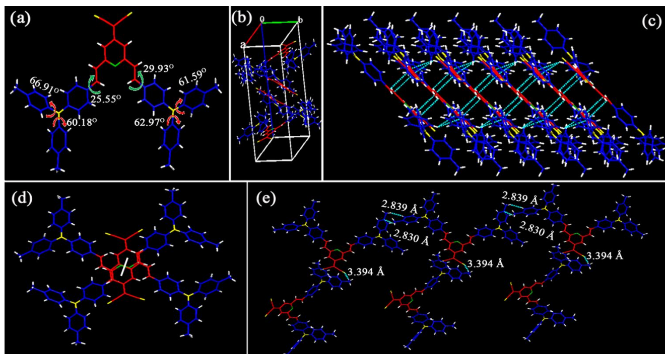
Fig. 3 Single crystal structure of M-TPA-DCM: (a) Molecular structure of M-TPA-DCM in crystal. (b) Crystal cell for M-TPA-DCM in b direction. (c) Molecular packing manner of M-TPA-DCM in c direction. (d) Intermolecular interactions of M-TPA-DCM and (e).
