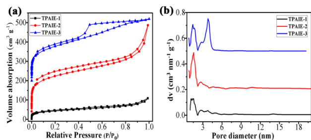
Fig. 4(a) Nitrogen adsorption-desorption isotherms of TPAIEs at 77 K. (b) The NL-DFT pore size distribution of TPAIEs
