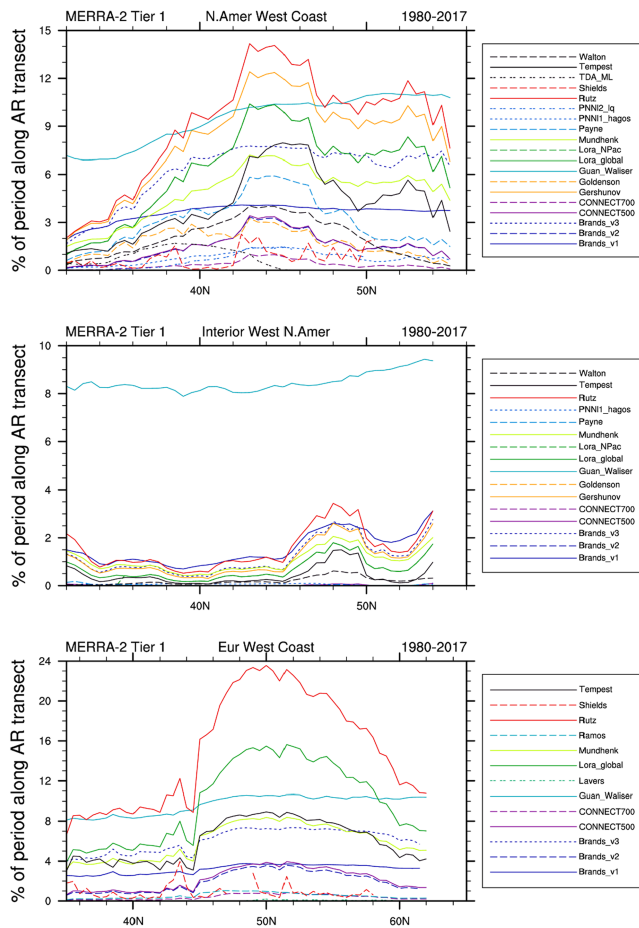
Figure 6. AR frequency of ARTMIP methods for selected transects (a) along the North American West Coast, (b) through interior western North America, and (c) along the European West Coast. Note that some methods are only available over certain regions.
