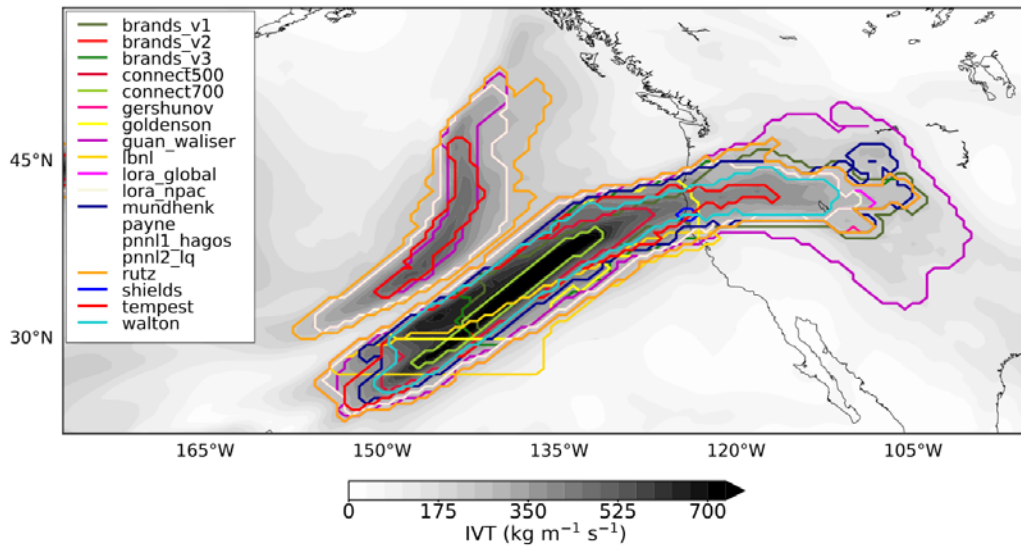
Fig. 2: Example of how AR identification and tracking methods differ over the northeastern Pacific, based on MERRA v2 data from 0000 UTC 15 February 2014. Gray shading represents IVT ( \text{kg m}^{-1} \text{s}^{-1} ), and colored contours represent the spatial regions designated as ARs by the various methods. Note that only algorithms available in this region are shown.
