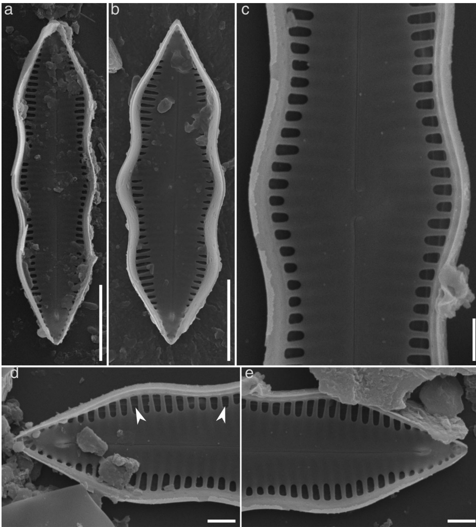
Fig. 6. K. triundulata gen. et sp. nov., SEM internal views. (a,b) Whole valve view, with axial plate evident as well as distinct helictoglossae at the poles. (c) Central area, showing proximal raphe ends strongly deflected in same direction. (d,e) Valve apices, with small, elongated helictoglossa. The axial plate extends at the center and narrows near the apices, note the siliceous slat system (arrowheads). Scale bars = 5 \mu m (a,b); 1 \mu m (c–e). Specimens from the type locality, India.
