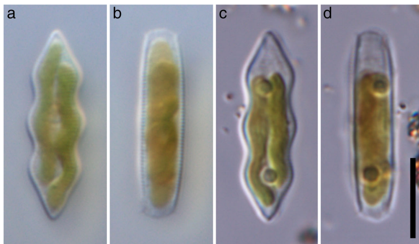
Fig. 1. Live cells with chloroplast structure of Kulikovskiyia triundulata gen. et sp. nov. (a,b) Girdle view and valve view of the same cell. (c,d) Girdle view and valve view of the same cell. (Scale bar represents 10 \mu m). [Color figure can be viewed at wileyonlinelibrary.com ]
