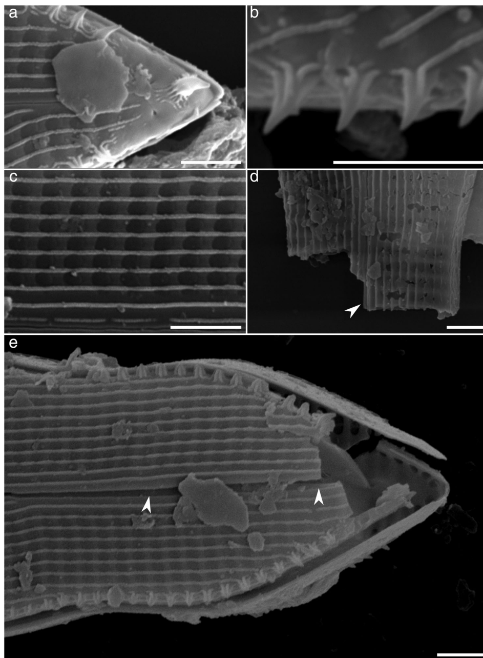
Fig. 5. SEM images of K. triundulata gen. et sp. nov. (a) Robust terminal spine with marginal spines. (b) Magnified view of marginal spines. (c) Parallel siliceous slats are evident with occluded striae. (d,e) External broken valves showing raphe fissure (arrow-head). (All scale bars represents 1 \mu m). Specimens from the type locality, India.
