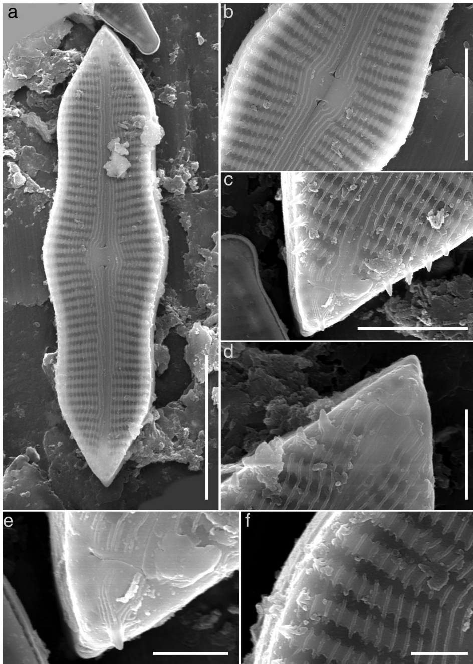
Fig. 8. Kulikovskiyia sp. from the Chinese material. SEM of the external part from one single frustule. (a) Whole valve view. (b) Close up view of the valve center with proximal raphe ends. (c,d) Distal raphe endings with apical and marginal spines. (e) Close up view of conical apical spine. (f) Close up view of marginal spines. (Scale bars: a = 10 \mu\text{m} ; b = 5 \mu\text{m} ; c = 3 \mu\text{m} ; d = 2 \mu\text{m} ; e, f = 1 \mu\text{m} ).
