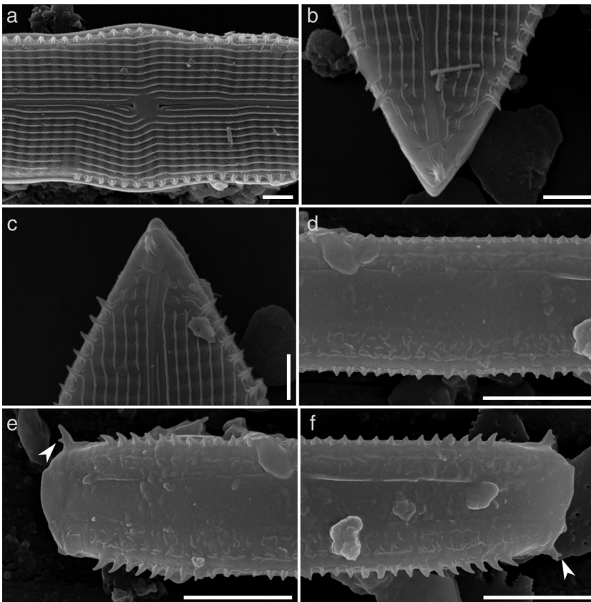
Fig. 3. SEM of K. triundulata gen. et sp. nov., external valve views. (a,b) Valve views showing peripheral and apical spines, siliceous slats and tri-undulate valve shape, arrowhead showing opposite orientation of conical spines. (c) External girdle views, apical spines with small side branch (arrowhead). (All scale bars represents 5 \mu m). Specimens from the type locality, India.
