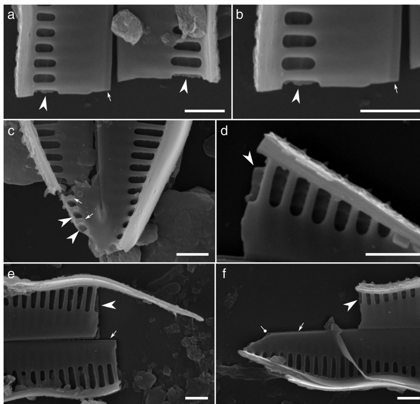
Fig. 7. K. triundulata gen. et sp. nov., SEM internal views of broken valves. (a,b) Showing broken chambered striae (arrowheads) and raphe fissure (arrow). (c) Apical portion showing open chambers (arrowheads) and internal strut (fibulae-like) structures (arrows). (d) One broken chambered stria (arrowhead) with siliceous slats bearing inner side of valve outer cover. (e) Broken apical part showing chambered stria (arrowhead) beneath the axial plate and raphe fissure (arrow). (f) Chambered stria (arrowhead), raphe fissure (arrow) and helictoglossa fissure (round pointer). (All scale bars represents 1 \mu m). Specimens from the type locality, India.
