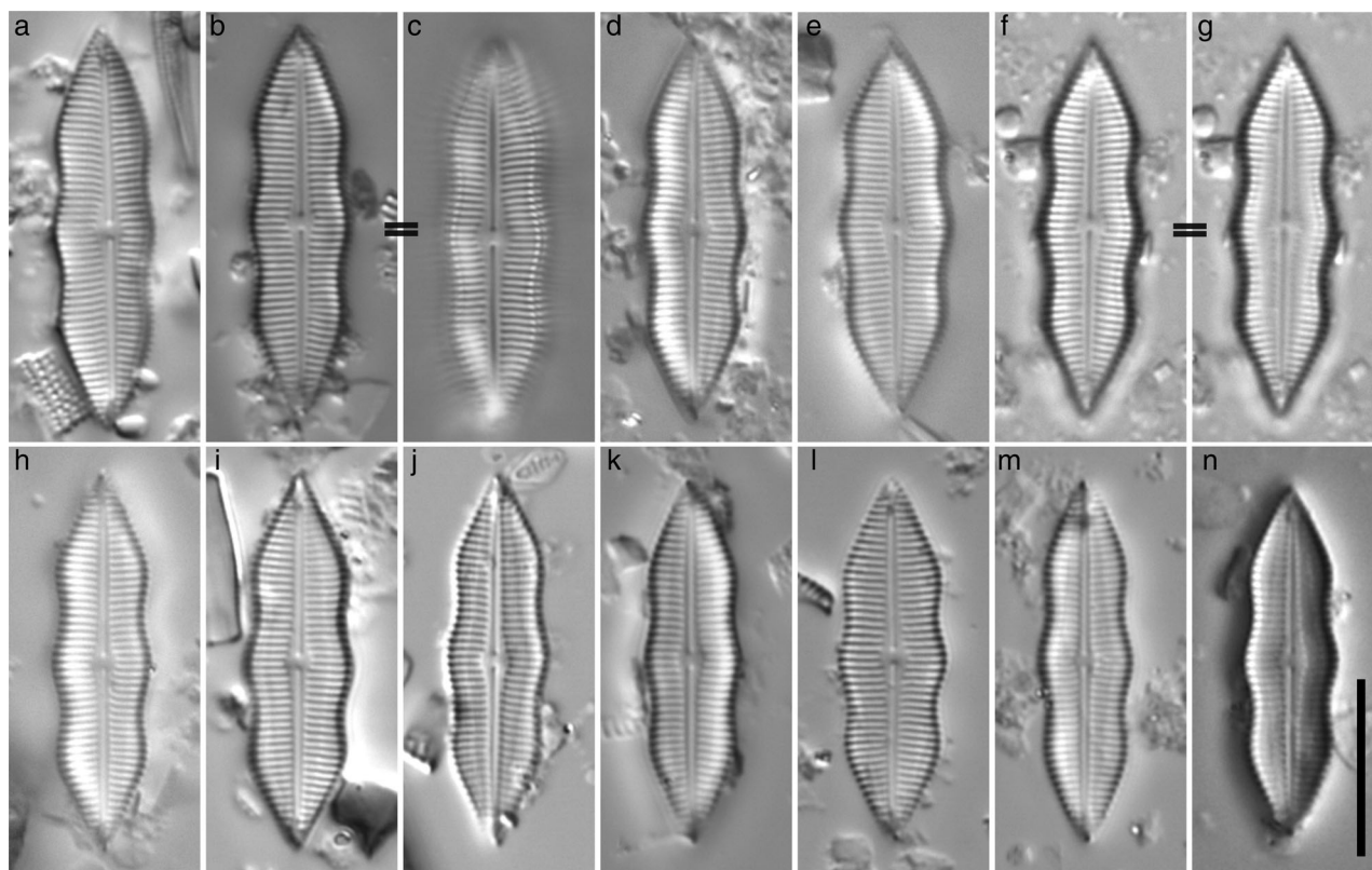
Fig. 2. Light microscopy of K. triundulata gen. et sp. nov., from the type population; valve views showing the size diminution series. Holotype depicted in b,c. (b,c) Frustules in valve view with different focal plain showing distinct raphe and central area of both valves. (f,g) Longitudinal lines due to the internal axial plate under different focus. (Scale bar represents 10 \mu m). Specimens from the type locality, India.
