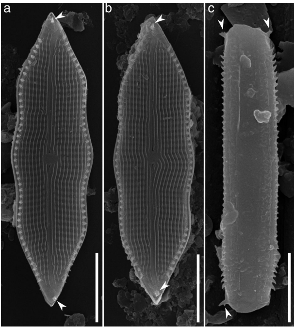
Fig. 3. SEM of K. triundulata gen. et sp. nov., external valve views. (a,b) Valve views showing peripheral and apical spines, siliceous slats and tri-undulate valve shape, arrowhead showing opposite orientation of conical spines. (c) External girdle views, apical spines with small side branch (arrowhead). (All scale bars represents 5 \mu m). Specimens from the type locality, India.
