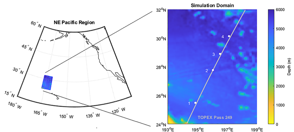
Figure 1. (left) The Northeast Pacific region showing a colored box at the location of the simulation domain. (right) A close-up of the simulation domain including the local bathymetry (color), the locations of the MMPs (white dots), and the trajectory of TOPEX/Poseidon satellite pass #249 (gray line).
