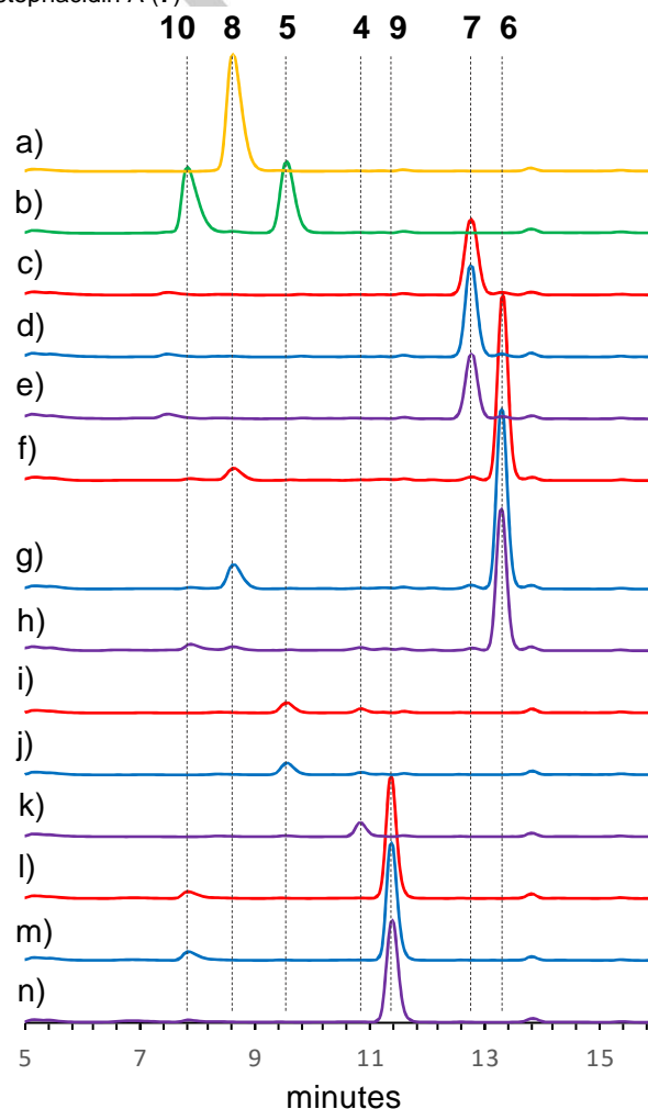
Figure 1. Biochemical activity assays with NotI and NotI'. (a) (+)-versicolamide B (8) standard. (b) (+)- and (-)-notoamide B (5 and 10) standards. (c) NotI' reaction with (-)-6- epi -stephacidin A (7). (d) NotI reaction with 7. (e) No enzyme control with 7. (f) NotI' reaction with (+)-6- epi -stephacidin A (6). (g) NotI reaction with 6. (h) No enzyme control with 6. (i) NotI' reaction with (-)-stephacidin A (4). (j) NotI reaction with 4. (k) No enzyme control with 4. (l) NotI' reaction with (+)-stephacidin A (9). (m) NotI reaction with 9. (n) No enzyme control with 9. No enzyme controls are shown in purple, reactions with NotI are shown in blue, and
