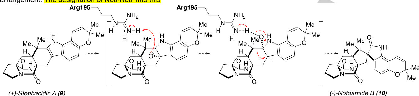
Scheme 3. Proposed mechanism for epoxidation and spirocyclization catalyzed by NotI and NotI'.
