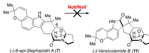
Scheme 1. Reactions catalyzed by NotI/NotI' in vitro and in the respective native fungal species.
