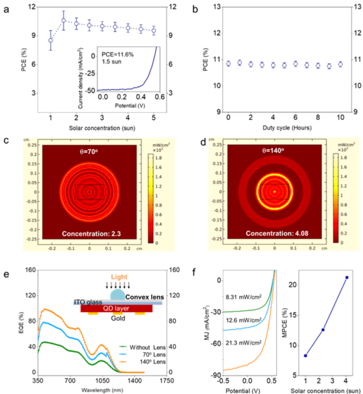
Figure 3 | QD CPV system and integrated polymer-lens CPV system characteristics. a, PCE performance of QDSCs under different solar concentrations. The inset displays the J-V curve of the as-prepared champion cell. b, Unencapsulated QDSC PCE stability performance under 3 Suns insolation for a continuous 10 hours exposure. c, d, Ray trajectories simulated with COMSOL Multiphysics emanating from a 70° and 140° contact angle micro-lens. e, EQE curves of the QD polymer-lens CPV system under 1.5G AM irradiance. Inset of (e) shows the structure of the QD CPV system. f, MJ-V, and MPCE as a function of the solar concentration ratio.
