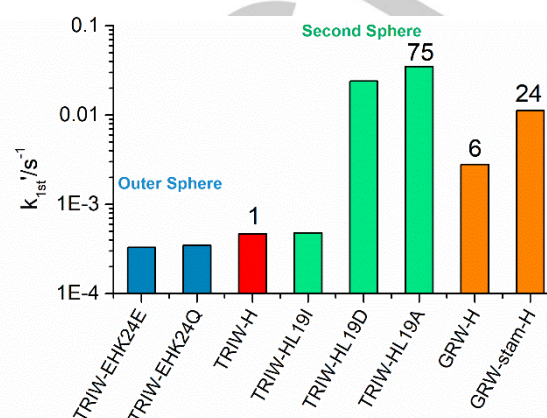
Figure 2. Pseudo-first order rate constants for Cu catalyzed NiR activity at pH 5.8 for the original construct TRI W-H (red) [9] , previously described modifications to the exterior (blue) [11] and interior (green) [12] compared to those determined for GRW -H and GRW 27stamAEL L33H (orange).
