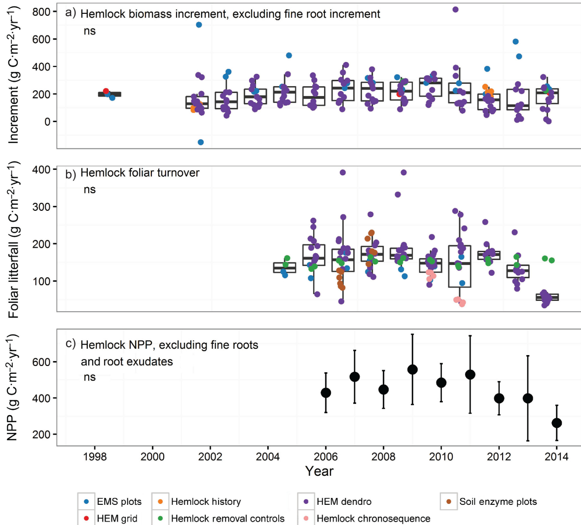
FIG. 6. Components of NPP at the Harvard Forest over time for hemlock-dominated plots: (a) biomass increment (above-ground and coarse roots); (b) foliar litter production; (c) NPP combining woody increment aboveground, coarse root increment, and total litter production. None of these showed a significant trend over time (noted as ns). Data for total litterfall began in 2005 for the hemlock plots, which is why panel c shows data only from 2006–2014. Box plot components in panels a and b are midline, median; box edges, first and third quartiles; and whiskers, 1.5 * interquartile range.
