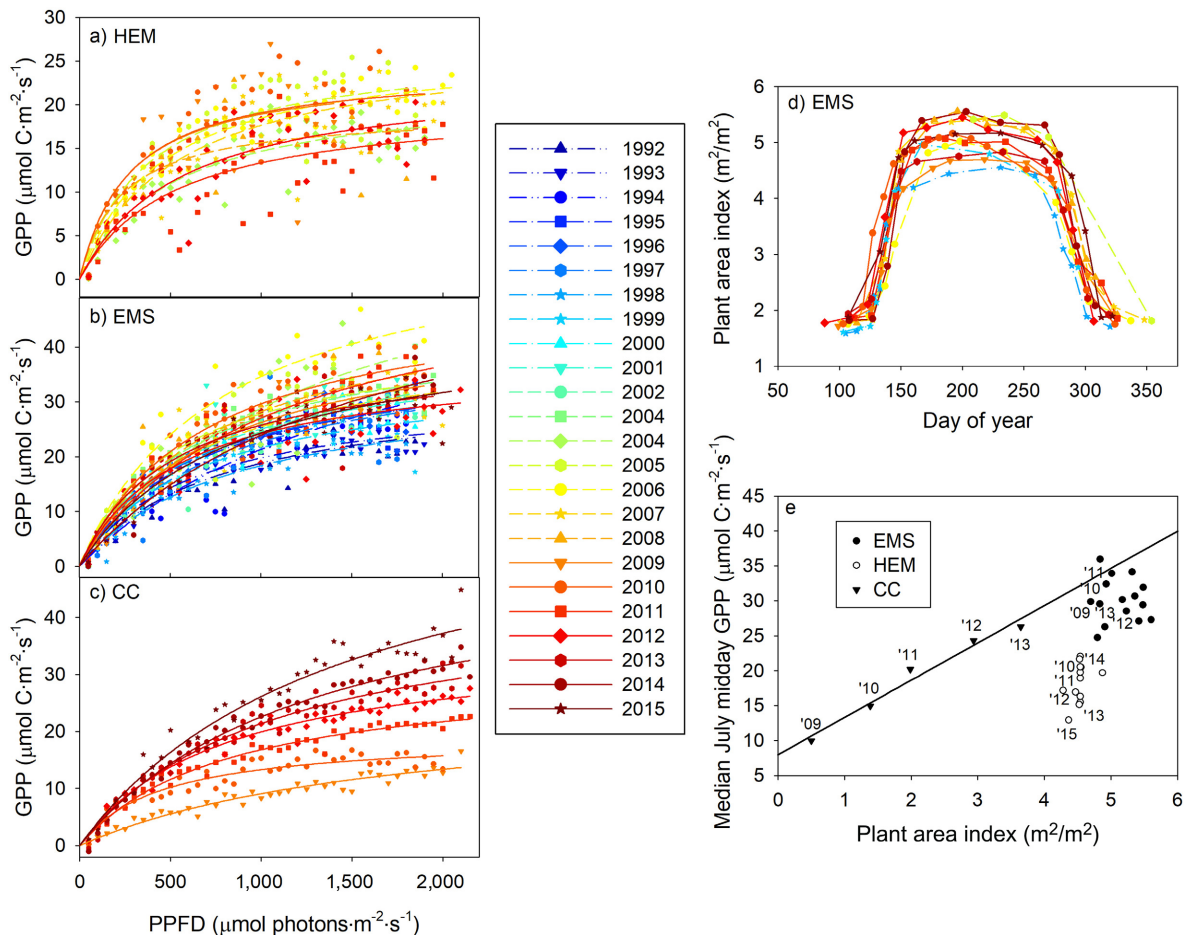
FIG. 8. Notable features of the eddy-covariance and plant-area index (PAI) data sets. July GPP as a function of photosynthetic photon flux density for the (a) hemlock (HEM), (b) EMS, and (c) clear-cut (CC) tower sites. The fitted lines model light use efficiency using Eq. 3. Data were averaged within 50 \mu\text{mol photon}\cdot\text{m}^{-2}\cdot\text{s}^{-1} bins of photosynthetic photon flux density (PPFD). (d) The seasonal time course of leaf area index (LAI) at the EMS site and (e) median July midday GPP as a function of plant area index. Data from the HEM site are restricted to the time before clear sign of hemlock woody adelgid (HWA)-associated decline (2005–2012). The black line in panel e is the regression between CC-tower PAI and GPP.
