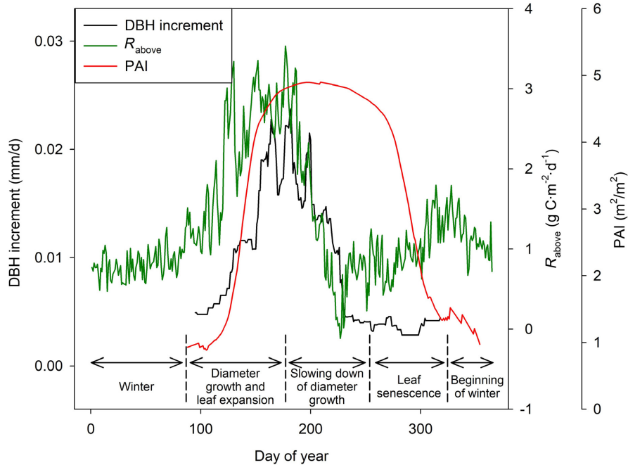
FIG. 11. Mean daily DBH increment, mean daily aboveground respiration ( R_{\text{above}} , and plant area index (PAI) at the EMS site for 1998–2003 and 2006. A total of 1,320 trees (>5 cm DBH) of 16 species were measured 6–19 times per year.
