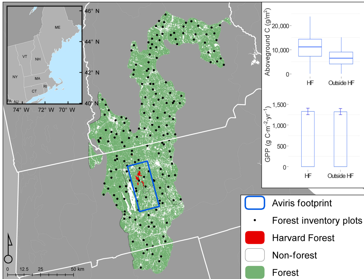
FIG. 2. Regional comparison of production and C stocks in biomass. Distribution of C in biomass in FIA plots (black dots) within EPA ecoregions 58g and 59b (green polygon) is lower than that at the Harvard Forest (red outline). GPP estimated from AVIRIS (blue box) does not differ between the Harvard Forest and full AVIRIS footprint.
