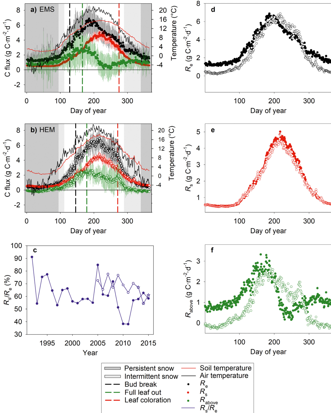
FIG. 10. Median daily fluxes of C at the (a) EMS and (b) HEM sites. The data in this figure were first published in Giasson et al. (2013) but were updated through the end of 2015. Ecosystem respiration is based on new data from the two eddy-covariance tower sites. No additional soil respiration data have been collected since Giasson et al. (2013) and the time series is extended based on an empirical model fit between flux and soil temperature data collected between 1992 and 2010 (see fig. A4 in Giasson et al. 2013). For the HEM site, data from the period during which hemlocks were declining (2013–2015) were not used. The shaded regions above and below the points reflect 1 SD of the average daily flux across the 24- and 8-yr records, respectively. Soil temperature was measured 20 cm below the soil surface at the EMS site and 10 cm below the surface at the HEM site. (c) The ratio of soil and total ecosystem respiration at the two sites. The median daily (d) ecosystem respiration, (e) soil respiration, and (f) aboveground respiration at the EMS and HEM sites. Open symbols represent the HEM site and closed symbols the EMS site. In panel c, star symbols indicate years during which hemlocks were in decline.
