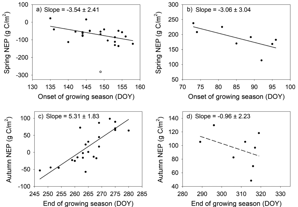
FIG. 13. Relationship between the date of the onset of the growing season and springtime NEP for the (a) EMS and (b) HEM sites. Also, the relationship between the date of the end of the growing season and autumn NEP for the (c) EMS and (d) HEM sites. The onset of the growing season is defined as the first day of the year when daily NEP was above a threshold of 30% of the mean maximum daily NEP. Similarly, the last day when NEP was above the threshold was considered to be the end of the growing season. Spring is defined as March–May and autumn is September–November. Regressions are statistically significant (EMS spring, \text{Adj-}r^2 = 0.27 , P = 0.006 ; EMS autumn, \text{Adj-}r^2 = 0.61 , P < 0.001 ; HEM spring, \text{Adj-}r^2 = 0.42 , P = 0.049 ) except in the autumn at the HEM site ( \text{Adj-}r^2 = 0.02 , P = 0.333 ). The 95% confidence interval of the slopes are indicated. Solid and dashed lines represent significant and insignificant relationships, respectively.
