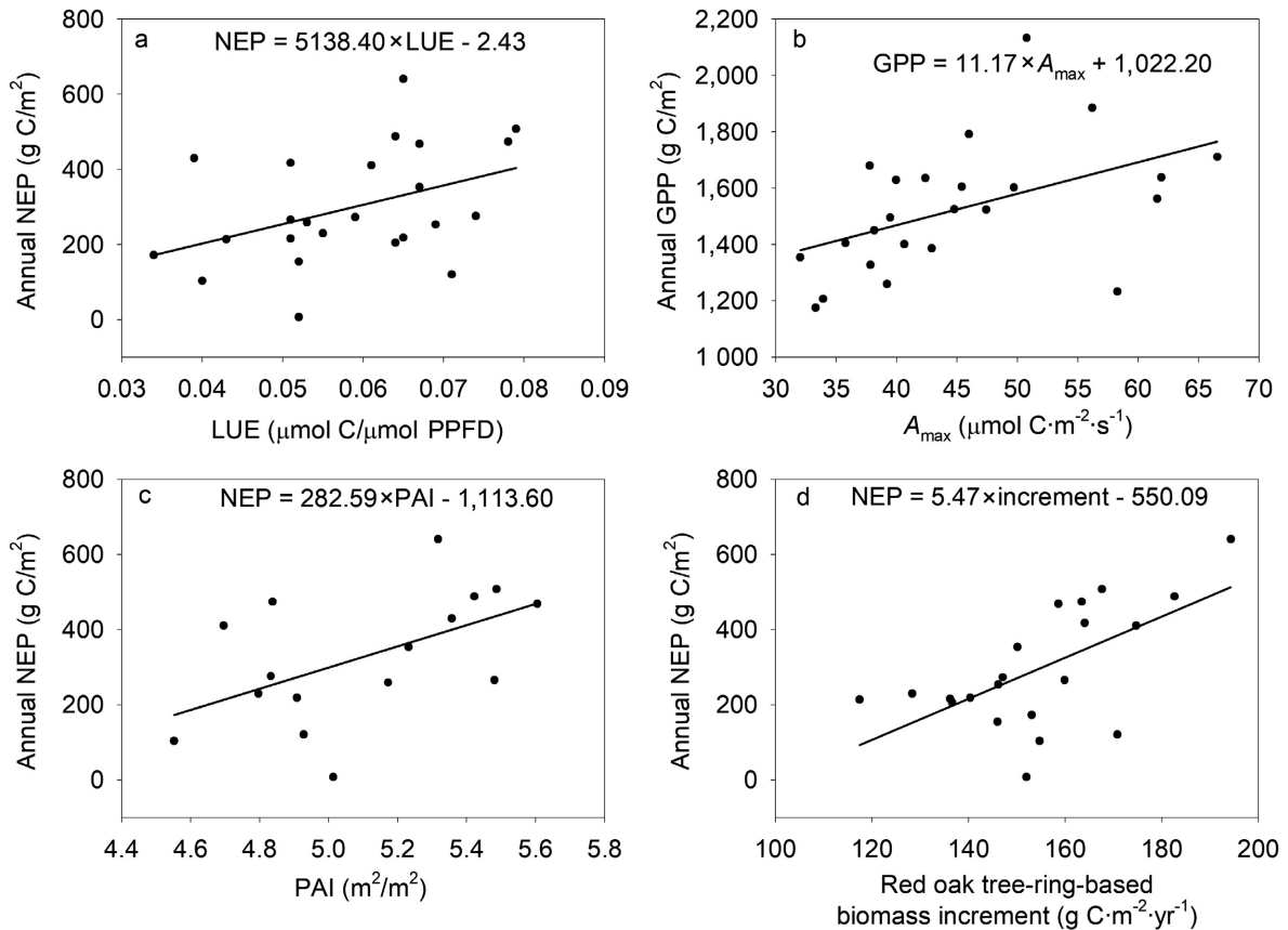
FIG. 9. Relationship between (a) NEP and light-use efficiency (LUE; Adj- r^2 = 0.13 , P = 0.045 ), (b) GPP and ecosystem photosynthetic capacity ( A_{max} ; Adj- r^2 = 0.20 , P = 0.018 ), (c) NEP and PAI (Adj- r^2 = 0.23 , P = 0.035 ), and (d) NEP and red oak tree-ring-based biomass increment (Adj- r^2 = 0.35 , P = 0.003 ) at the EMS site.
