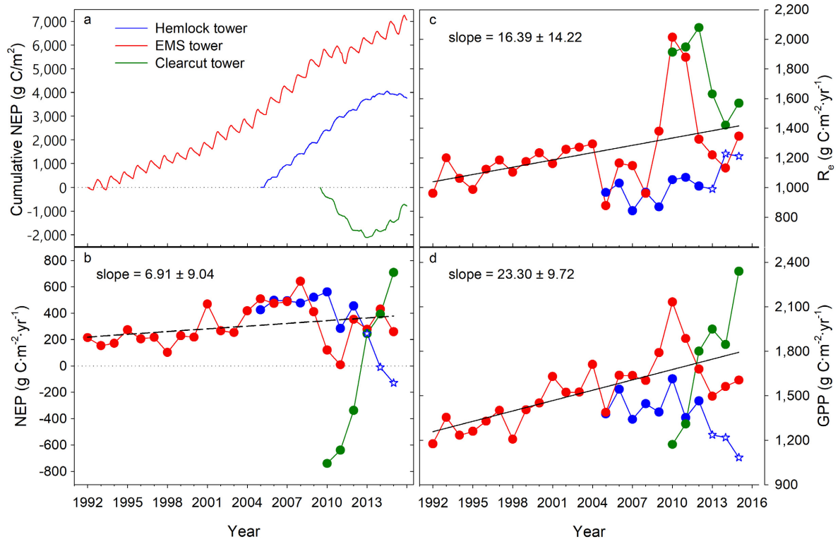
FIG. 7. (a) Cumulative and (b) annual net ecosystem production (NEP) and its component fluxes (c) total ecosystem respiration ( R_e ) and (d) gross primary production (GPP). Star symbols represent years during which hemlocks were in decline. The black lines in panels b–d represent the significant (solid) or nonsignificant (dashed) trends in increasing NEP, R_e , and GPP with time at the EMS site (NEP, \text{Adj-}r^2 = 0.06 , P = 0.127 ; R_e , \text{Adj-}r^2 = 0.17 , P = 0.026 ; GPP, \text{Adj-}r^2 = 0.51 , P < 0.001 ).
