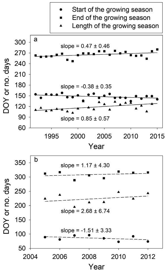
FIG. 12. Climate metrics at the Harvard Forest. Start and end dates of the growing season and the length of the growing season at the (a) EMS and (b) HEM eddy-covariance sites. All regressions for the EMS site are statistically significant ( \text{Adj-}r^2 = 0.15 , P = 0.0351 ; \text{Adj-}r^2 = 0.13 , P = 0.0459 ; \text{Adj-}r^2 = 0.27 , P = 0.0052 for the start, end, and length of the growing season, respectively). No regression was statistically significant at the HEM site ( \text{Adj-}r^2 = 0.03 , P = 0.310 ; \text{Adj-}r^2 = -0.09 , P = 0.531 ; \text{Adj-}r^2 = -0.01 , P = 0.368 for the start, end, and length of the growing season, respectively). The 95% confidence interval of the slopes are indicated. Solid lines show statistically significant relationships and dashed lines show insignificant ones. DOY, day of year.
