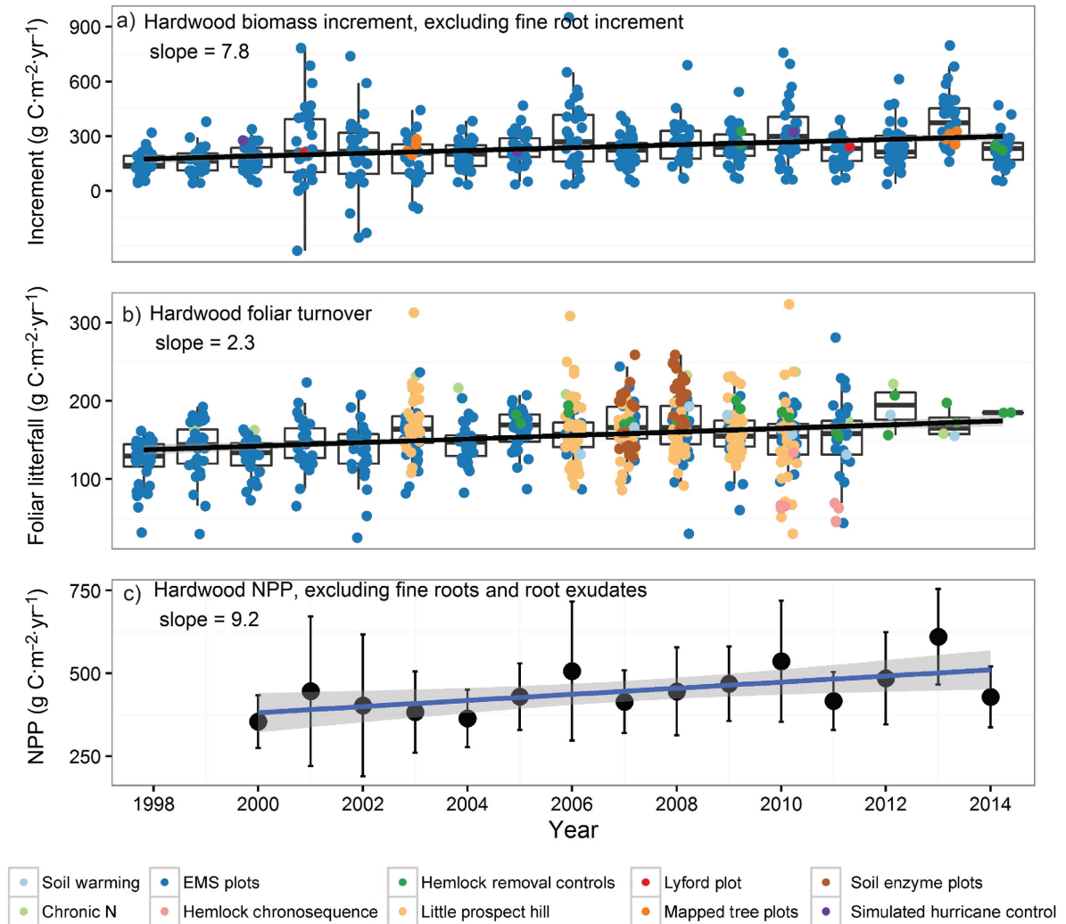
Fig. 5. Components of net primary production (NPP) at the Harvard Forest over time for hardwood-dominated plots: (a) biomass increment (aboveground and coarse roots), SE of slope = 1.22, P < 0.001 , \text{Adj-}r^2 = 0.07 ; (b) foliar litter production, SE of slope = 0.37, P < 0.001 , \text{Adj-}r^2 = 0.05 ; (c) NPP combining woody increment aboveground, coarse root increment, and total litter production, SE of slope = 3.3, P = 0.016 , \text{Adj-}r^2 = 0.32 . Data for total litterfall began in 1999 for the hardwood plots, which is why panel c shows data only from 2000–2014. Box plot components in panels a and b are midline, median; box edges, first and third quartiles; and whiskers, 1.5 * interquartile range.
