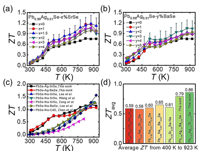
Figure 6. The Figure of merit, ZT , as a function of temperature for \text{Pb}_{0.99}\text{Ag}_{0.01}\text{Se}-x\% \text{ SrSe} (a) and \text{Pb}_{0.99}\text{Ag}_{0.01}\text{Se}-y\% \text{ BaSe} (b); Comparison of ZT values for p-type PbSe-based materials in this study with previously explored p-type PbSe thermoelectric materials (c) [5a,b,11] and comparison of ZT_{\text{avg}} values for a temperature gradient of 400 K to 923 K for top performing p-type PbSe-based materials (d). [5a,b,18]
