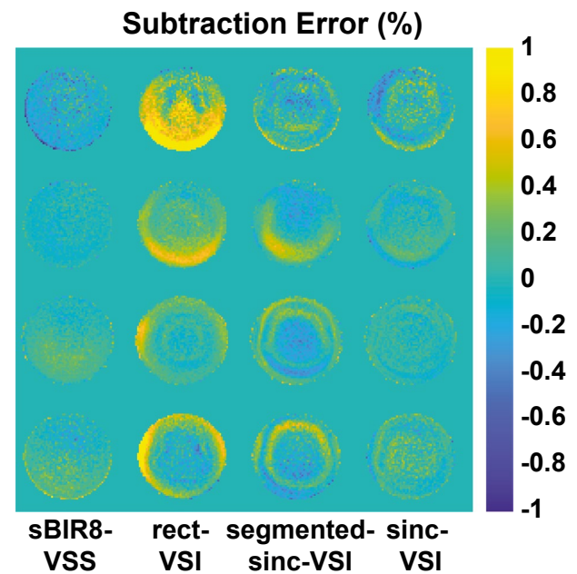
FIGURE 6 The subtraction error maps obtained from phantom scans, demonstrating EC sensitivity of the pulses. The velocity sensitive gradient pulses were applied in the S/I direction and the maps were normalized to the reference spin density image. The sBIR8-VSS and the sinc-VSI pulses showed comparable and low errors, whereas the rect-VSI and segmented-sinc-VSI had stronger sensitivity to EC effects with a spatially varying pattern. S/I, superoinferior
