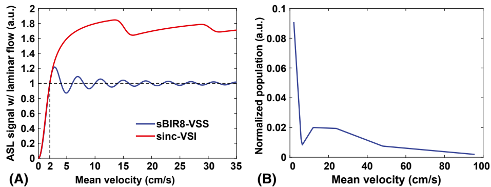
FIGURE 2 (A) The \text{Sig}_{\text{ASL}}\text{-}V_{\text{mean}} profiles for the VSS and VSI labeling after convolving with a laminar flow distribution, showing the definition of the cutoff velocity (eg, 2 cm/s); (B) the arterial blood population distribution obtained experimentally. Linear interpolation was used to estimate the population over the range of 2-96 cm/s of mean velocity. Note the well-matched cutoff profiles between VSS and VSI pulses. \text{Sig}_{\text{ASL}} , ASL signal; V_{\text{mean}} , mean velocity
