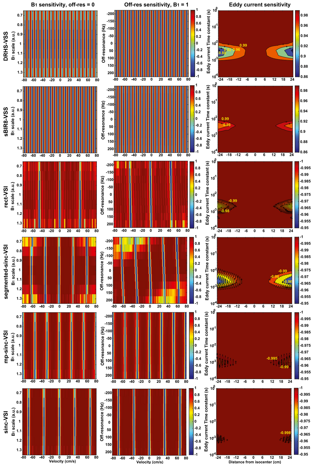
FIGURE 4 The simulation results showing the performance of the VS labeling pulses: (A) magnetization versus mean velocity response under the labeling condition showing the sensitivity to B_1 variation (ranging from 0.7 to 1.3 of the nominal value) without off-resonance; (B) magnetization versus mean velocity response under the labeling condition showing the sensitivity to B_0 variation (ranging from -200 Hz to 200 Hz) when B_1 = 1 ; and (C) magnetization of the static tissue ( V = 0 ) under the label condition showing EC sensitivity of the VSS and VSI pulses to EC components with different time constants (ranging from 0.1 ms to 1000 ms) at different distance to the iso-center of the magnet, where the magnetization under the control condition can be referred to the center line at distance = 0 . Please note the different color scales for VSS and VSI pulses. The sBIR8-VSS pulse demonstrated strong immunity to B_1 and B_0 variation and EC effects, whereas the sinc-VSI pulse had the highest robustness among the VSI pulses. Note that the response in panels A and B was generated before taking laminar flow effects into account. EC, eddy current
