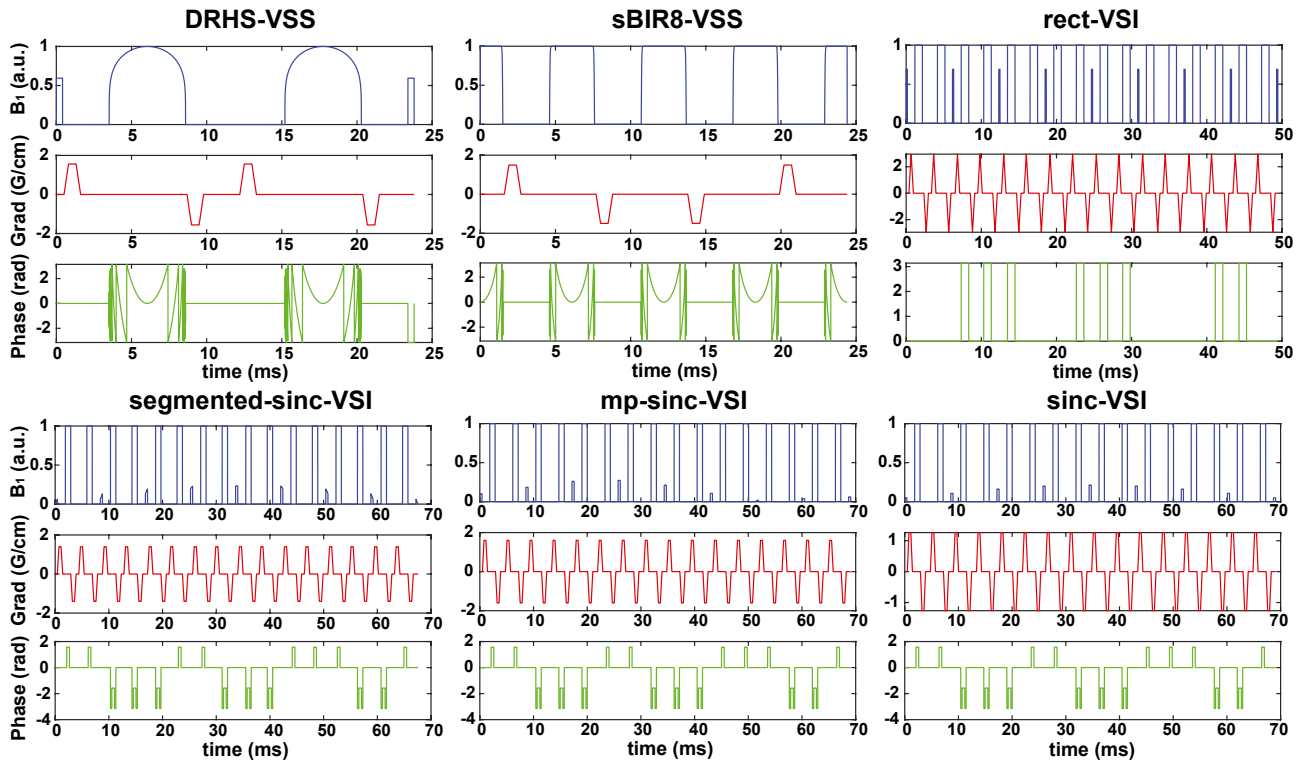
FIGURE 1 The pulse diagrams of DRHS-VSS pulse, sBIR8-VSS pulse, rect-VSI, segmented-sinc-VSI, mp-sinc-VSI, and the modified sinc-VSI. DRHS, double-refocused hyperbolic secant; mp-sinc-VSI, maximum-phased sinc modulation on the amplitude of the small flip-angle pulses; rect-VSI, original VSI pulse using hard RF of same small flip angle; sBIR8, symmetric 8-segment B_1 -insensitive rotation; segmented-sinc-VSI, modified VSI pulse with a regular sinc-shaped inversion pulse of 9 segments; VSI, velocity-selective inversion; VSS, velocity-selective saturation
