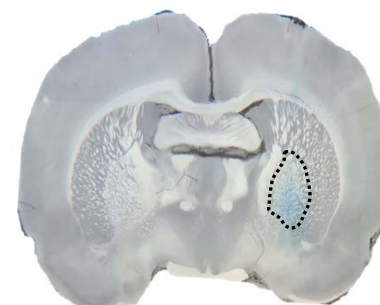
Bregma -1.00 mm
