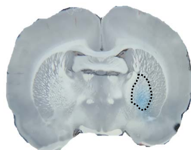
Bregma -0.90 mm
