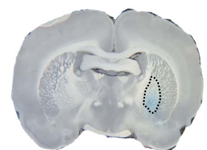
Bregma -1.1 mm
