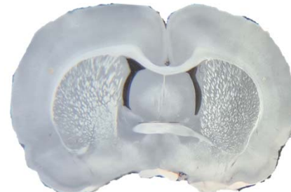
Bregma -0.20 mm
