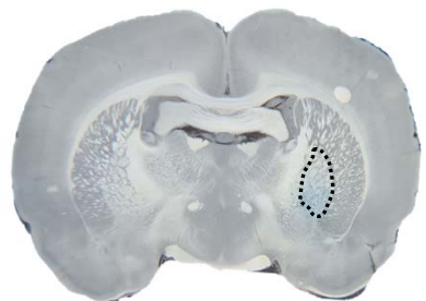
Bregma -1.30 mm
