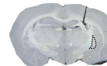
Bregma -1.80mm
