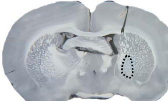
Bregma -0.50mm
