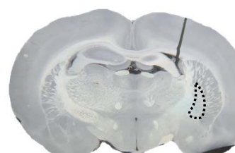
Bregma -1.60mm
