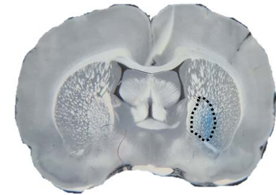
Bregma -0.60 mm
