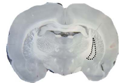
Bregma -1.80 mm
