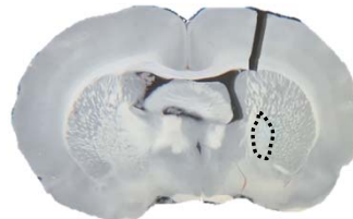
Bregma -0.30mm
