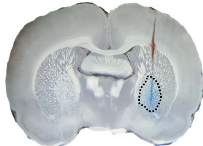
Bregma -0.80 mm
