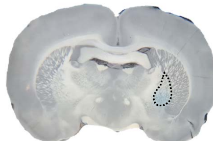
Bregma -1.50 mm
