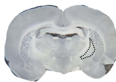
Bregma -1.70 mm
