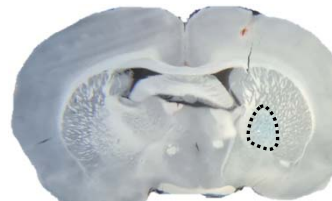
Bregma -0.70mm
