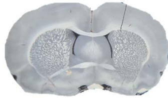
Bregma 0.20mm
