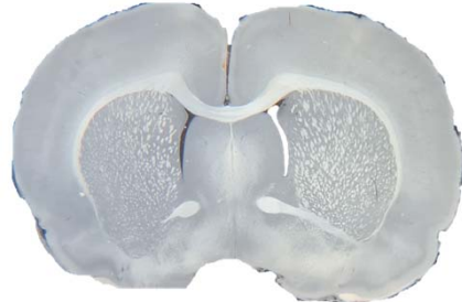
Bregma 0.30 mm
