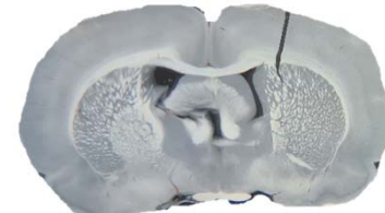
Bregma -0.20mm
