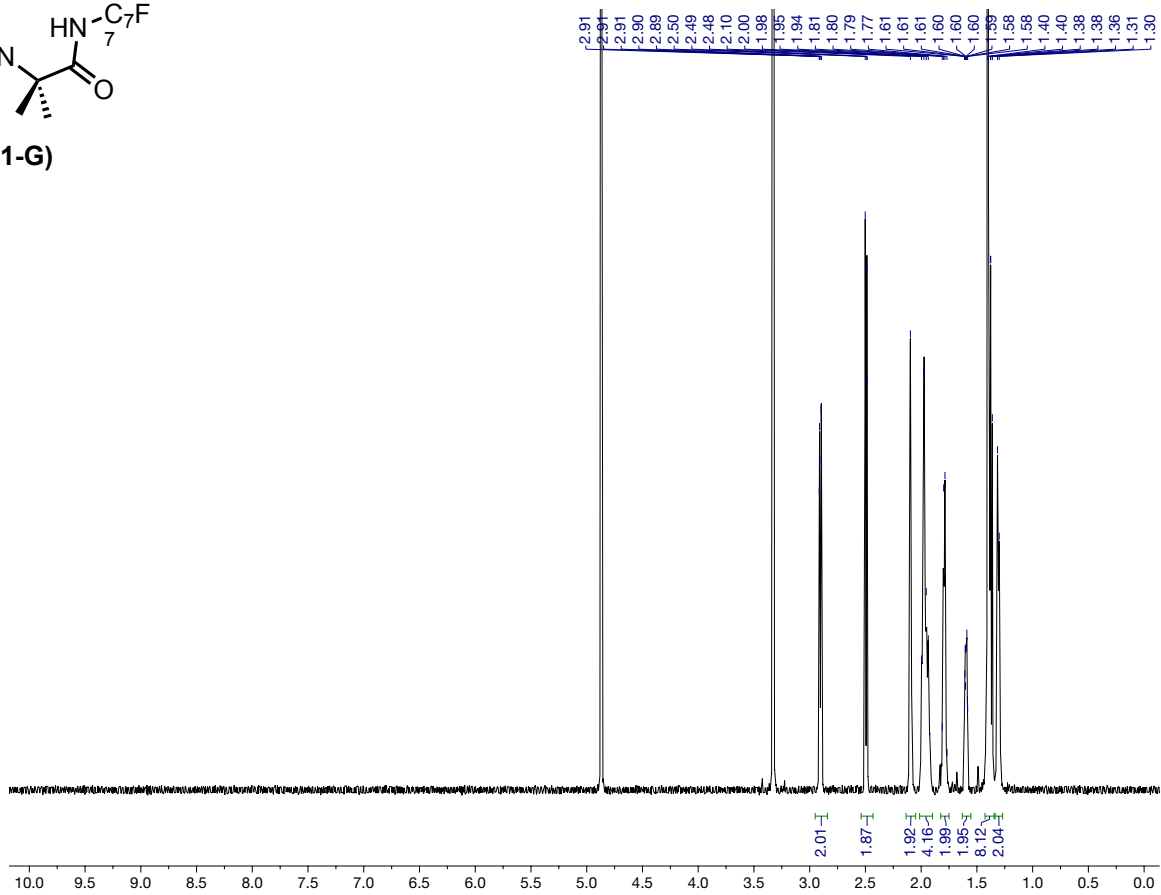
1 H NMR Spectrum in CD 3 OD
