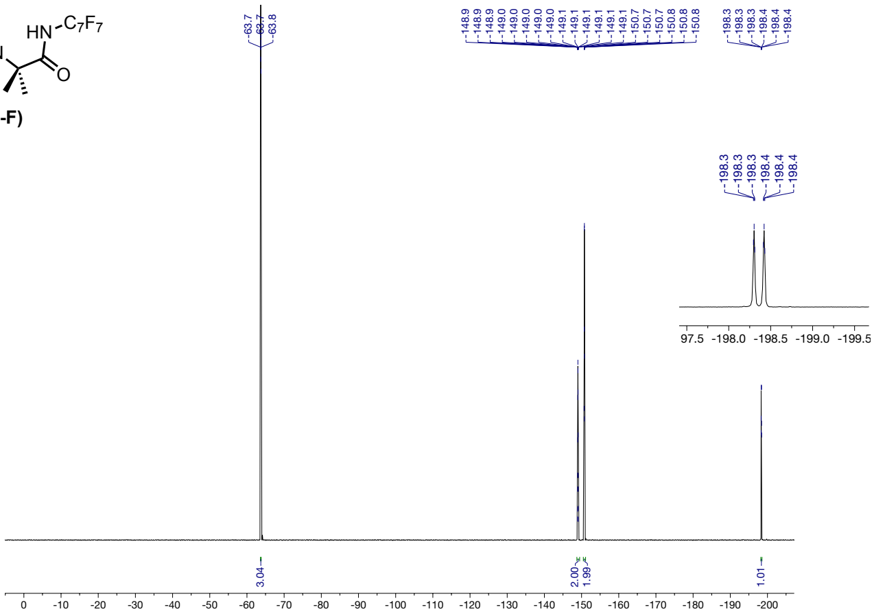
^{19}\text{F} NMR Spectrum in \text{CDCl}_3
