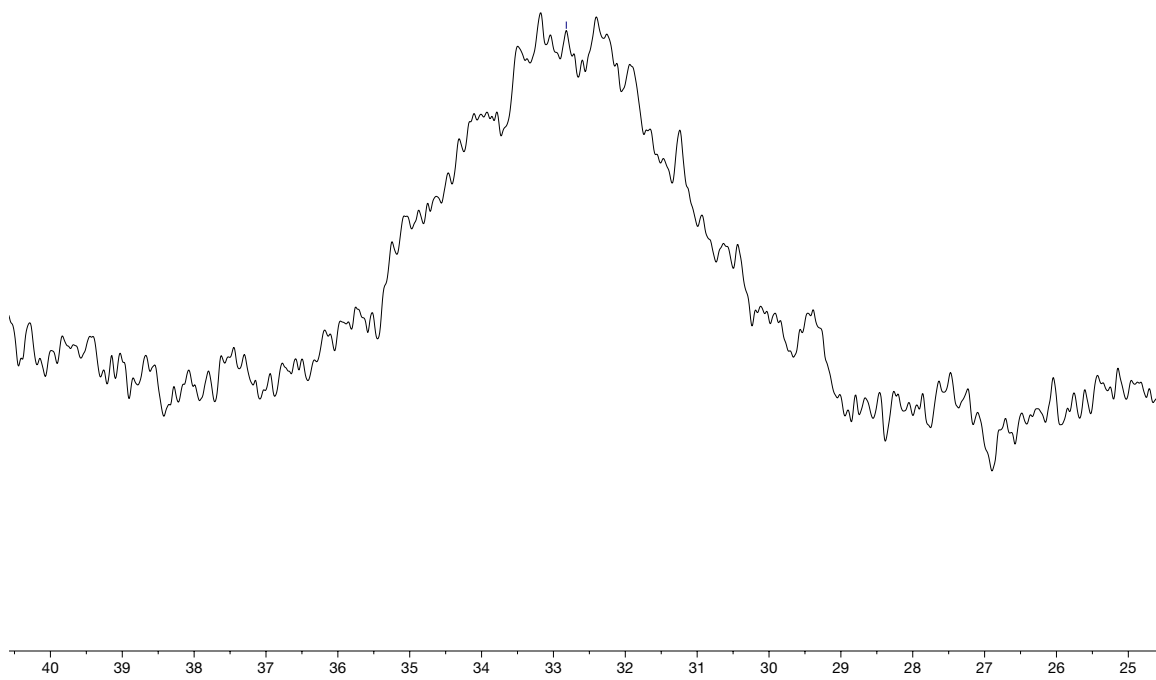
11 B NMR Spectrum in CDCl 3
