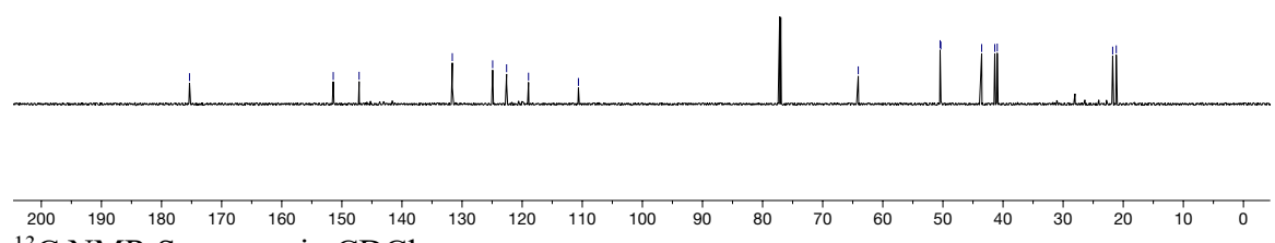
13 C NMR Spectrum in CDCl 3
