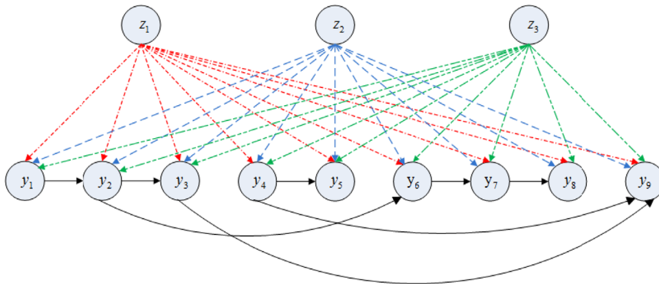
FIGURE 1 Part A presents four examples of directed mixed graphs. The graph in A(b) is cyclic, while all others are acyclic. An arrowed solid line indicates a directed edge and a dashed line denotes an undirected (or bidirected) edge. Part B presents an acyclic directed mixed graph that contains a DAG with the directed edges (arrowed solid lines) among nine observed variables y_1, \dots, y_9 and a set of undirected edges induced by three common latent factors z_1, z_2, and z_3 . This figure appears in color in the electronic version of this article, and any mention of color refers to that version
