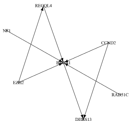
FIGURE 4 Subnetworks for master regulator genes (CCND2 and RUNX1) and master offspring genes (BRCA1 and LMO2), respectively. This figure appears in color in the electronic version of this article, and any mention of color refers to that version
