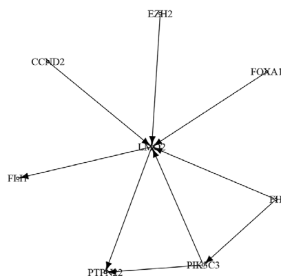
FIGURE 4 Subnetworks for master regulator genes (CCND2 and RUNX1) and master offspring genes (BRCA1 and LMO2), respectively. This figure appears in color in the electronic version of this article, and any mention of color refers to that version
