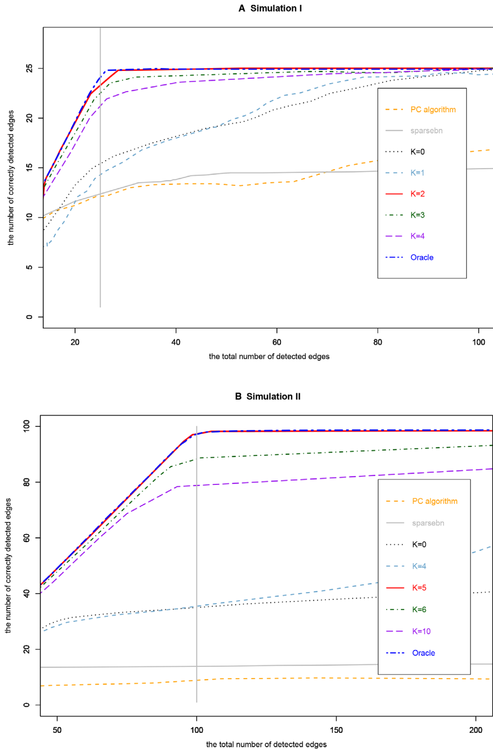
FIGURE 2 Summary results from two DAGs designed in the simulation studies. The x-axis is the total number of detected edges, and the y-axis is the average number of correctly identified edges over 50 replicates. The vertical (gray) line corresponds to the number of true edges. Panel A displays the results from the first small DAG simulation design with P = 50 , M = 25 , K = 2 , N = 25 as well as the estimated K_{ER} = 2 . Panel B shows the results of the second large DAG simulation design with P = 200 , M = 100 , K = 5 , N = 100 as well as the estimated K_{ER} = 5 . This figure appears in color in the electronic version of this article, and any mention of color refers to that version
