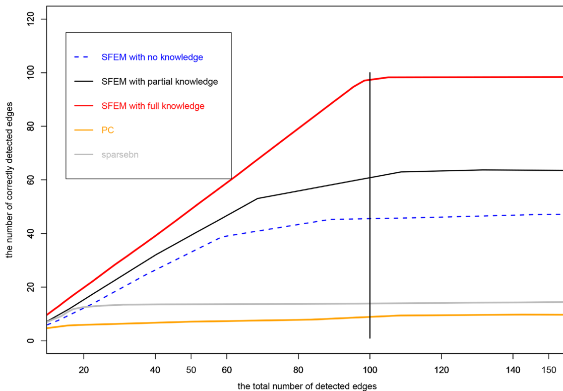
FIGURE 3 Summary results based on the large DAG simulation design with P = 200 , M = 100 , K = 5 , N = 100 as well as the estimated K_{ER} = 5 . The x -axis is the total number of detected edges, and the y -axis is the number of correctly identified edges averaged over 50 replicates. The vertical (black) line corresponds to the number of true edges. This figure appears in color in the electronic version of this article, and any mention of color refers to that version
