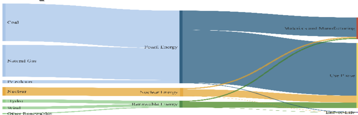
Figure 3. Life cycle primary energy flows for BEVs operating on 2019 U.S. average electric grid. The width of flow is directly proportional to total life cycle energy. Data are adapted from the GREET model (Argonne National Laboratory, 2018). Unlike fossil and nuclear sources (shown in blue and orange respectively), renewable energy sources (shown in green) inherently enhance automotive circularity. Underlying data used to create this figure can be found in the Supporting Information S1.
