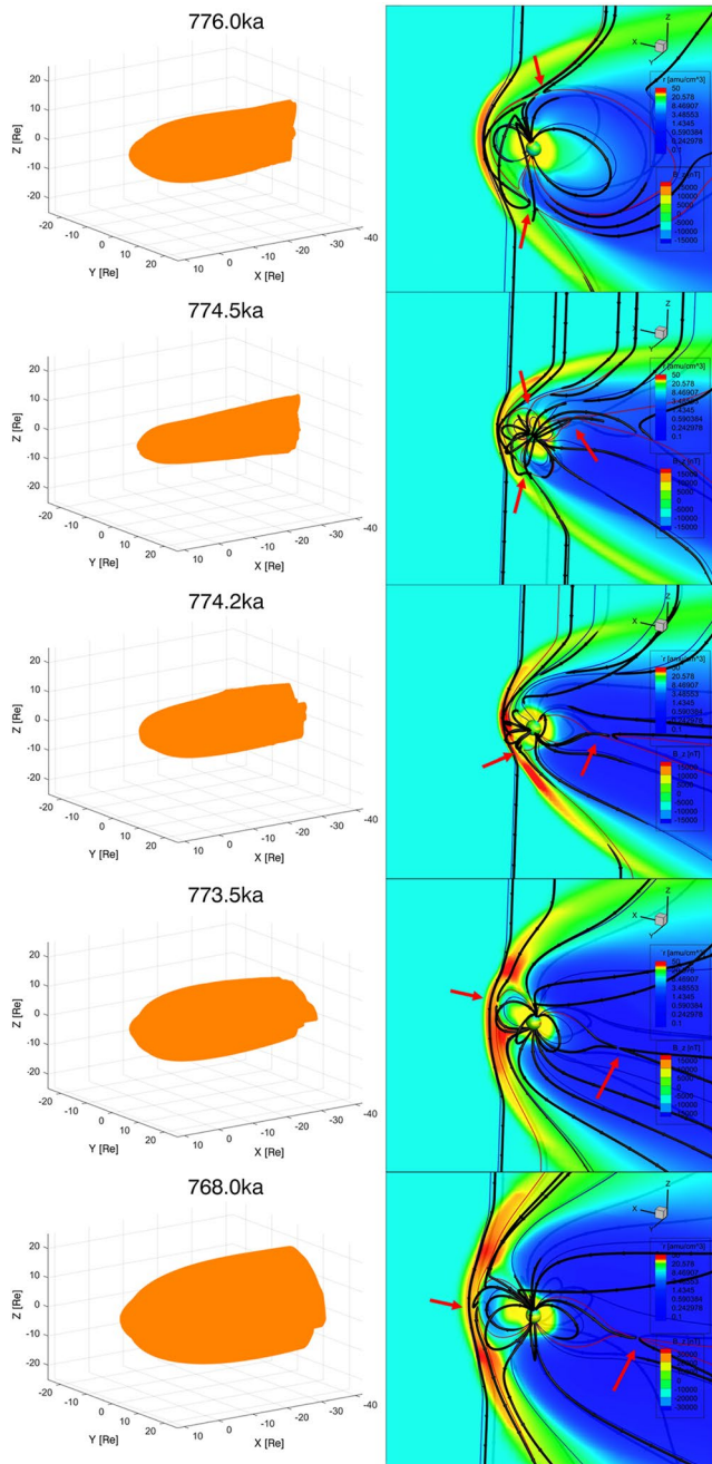
Figure 2. The left column displays the 3D view of the magnetopause surface at different phases during the Matuyama-Brunhes reversal; the right column shows the magnetic field lines in the magnetosphere. The red lines represent magnetic field lines being reconnected, projected into the Y = 0 plane. Color in the magnetosphere represents plasma density in \text{amu}/\text{cm}^3 . Color on the Earth surface is the magnitude of the geomagnetic field.
