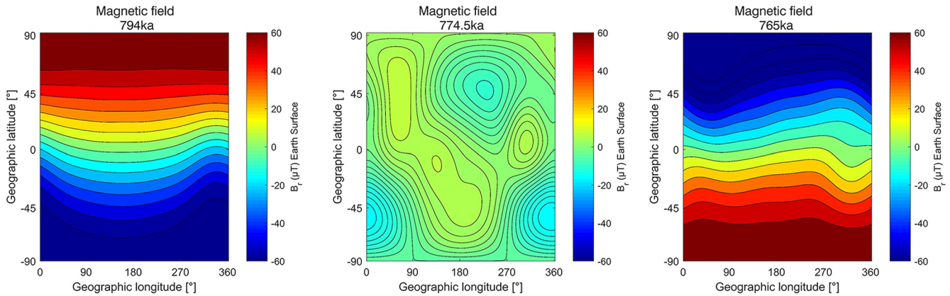
Figure 1. The global geomagnetic field distribution during the Matuyama-Brunhes reversal period using the data-reconstructed model “IMMAB4” (Leonhardt & Fabian, 2007). The X-axis and Y-axis represent geographic longitude and latitude, respectively.
