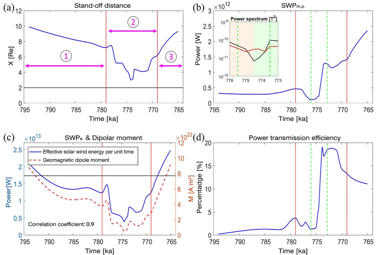
Figure 3. The temporal evolution of (a) the stand-off distance of subsolar point (in unit of Re), (b) total solar wind power gain through the magnetopause surface ( SWP_{m.p.} , in unit of Watt), (c) the effective solar wind power ( SWP_e , in unit of Watt), the geomagnetic dipole moment (red line, in unit of A m^2 ), and the present value of the geomagnetic dipole moment in 2020 (black line, in unit of A m^2 ), and (d) the ratio between SWP_{m.p.} and SWP_e , which represents the solar wind energy input efficiency. We divide the entire Matuyama-Brunhes reversal process into three phases with the vertical red lines: pre-reversal phase before 779 ka, reversal phase (779 ka–769 ka), and post-reversal phase after 769 ka. The small figure in (b) is the geomagnetic power spectrum of different components. The black and red lines represent the dipole component and the quadrupole component, respectively. The light red and green regions represent before and after the polarity reversal of the dipole component.
