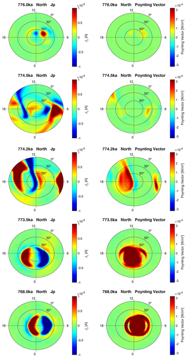
Figure 4. In the northern hemisphere, both projected field-aligned currents J_{||} (left) and Poynting flux (right) are from 776 ka to 768 ka in chronological order. The Red represents downward Poynting flux, the blue represents upward Poynting flux. The black circles are latitudes mapped to the altitude of the 2.5 Re.
