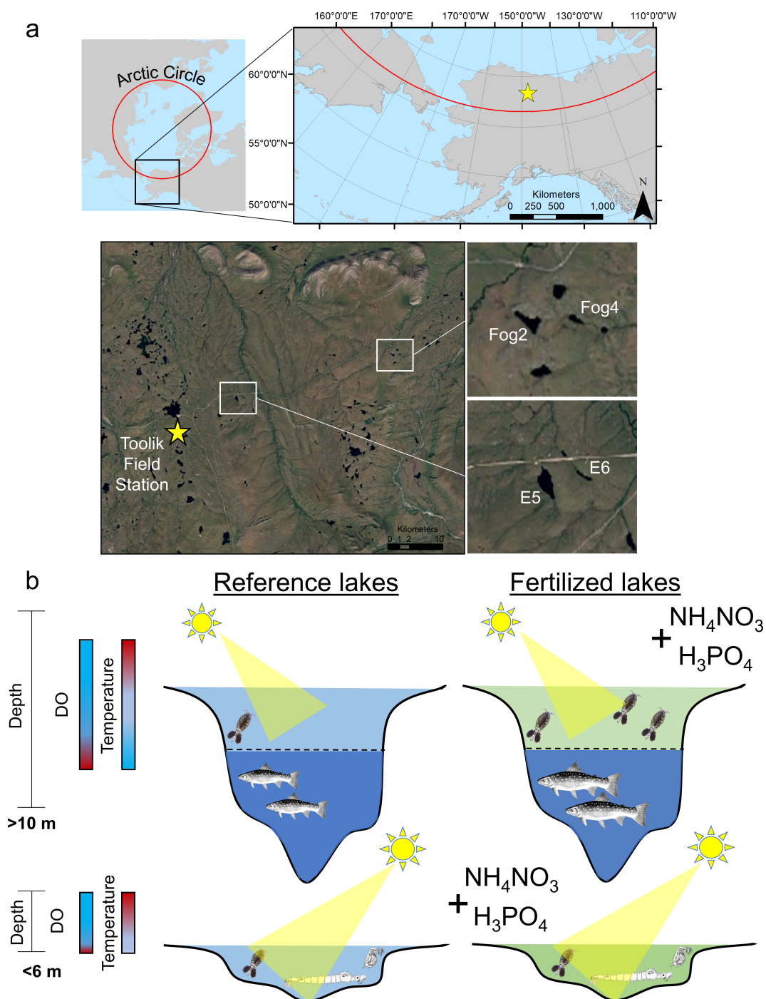
Fig. 1. (a) Location of Toolik Field Station (star) located on the North Slope of the Brooks Mountain Range, Alaska. The four lakes included in the experiment are labeled: E5 = fertilized deep lake with fish, E6 = fertilized shallow lake without fish, Fog 2 = reference deep lake with fish, Fog 4 = reference shallow lake without fish. (b) Conceptual diagram representing the two pairs of deep and shallow lakes. We manipulated one lake of each pair by fertilizing it with N and P, while keeping the other lake as a reference. Deep lakes typically stratify (dashed horizontal line) in the summer and contain fish. Sunlight reaches the bottom of the shallow lakes and these lakes are well mixed by wind. Zooplanktons are more numerous in the shallow lakes where fish are absent. We expected nutrient additions would stimulate primary producers (green shading), and zooplankton would increase in response. In the fertilized deep lake we expected fish condition would increase with food availability.
