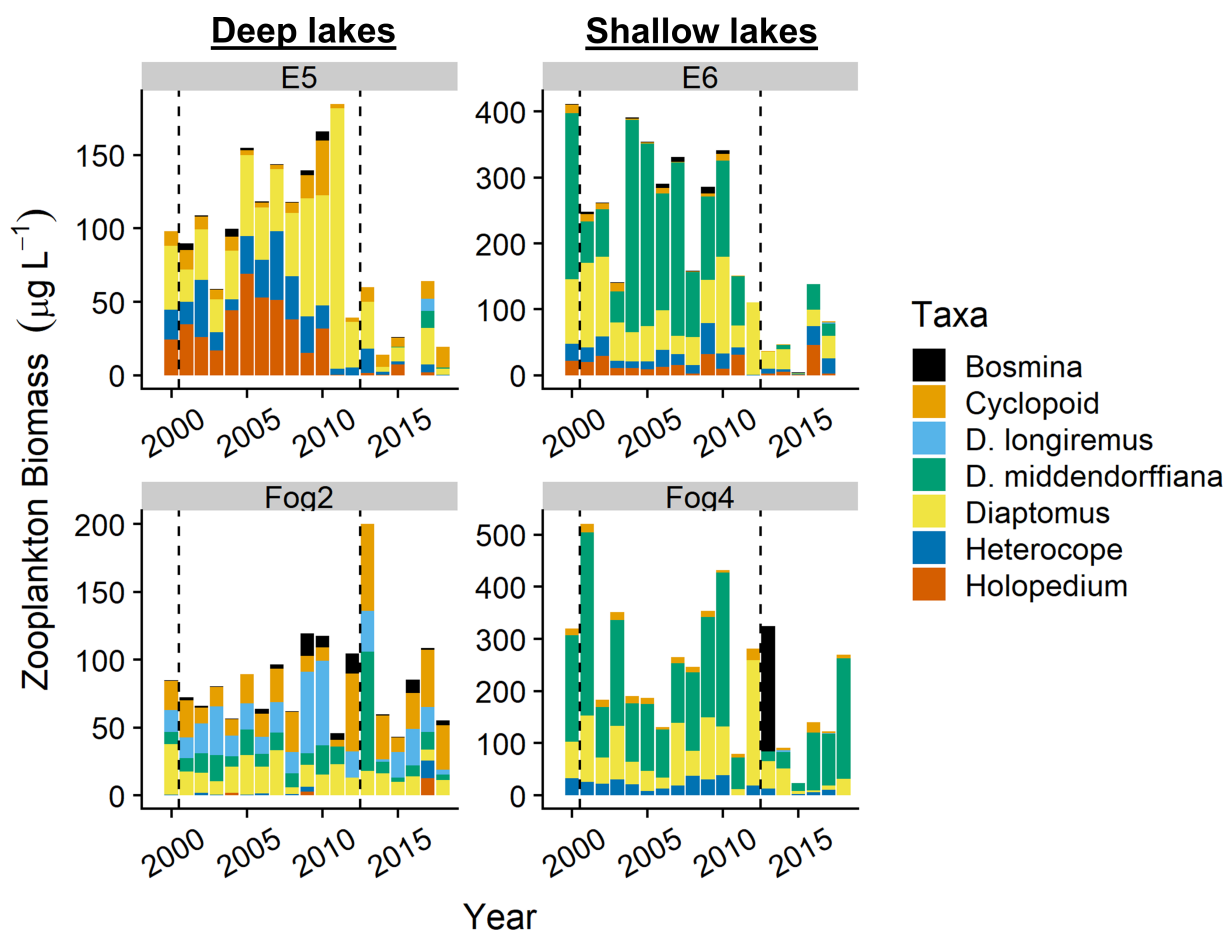
Fig. 4. Zooplankton biomass composition in each of the four study lakes. Dashed vertical lines represent the start and end of fertilization in E5 and E6. Major taxa are shown in the legend. We observed a natural thermokarst event in lake Fog4 from 2002 to 2004.
