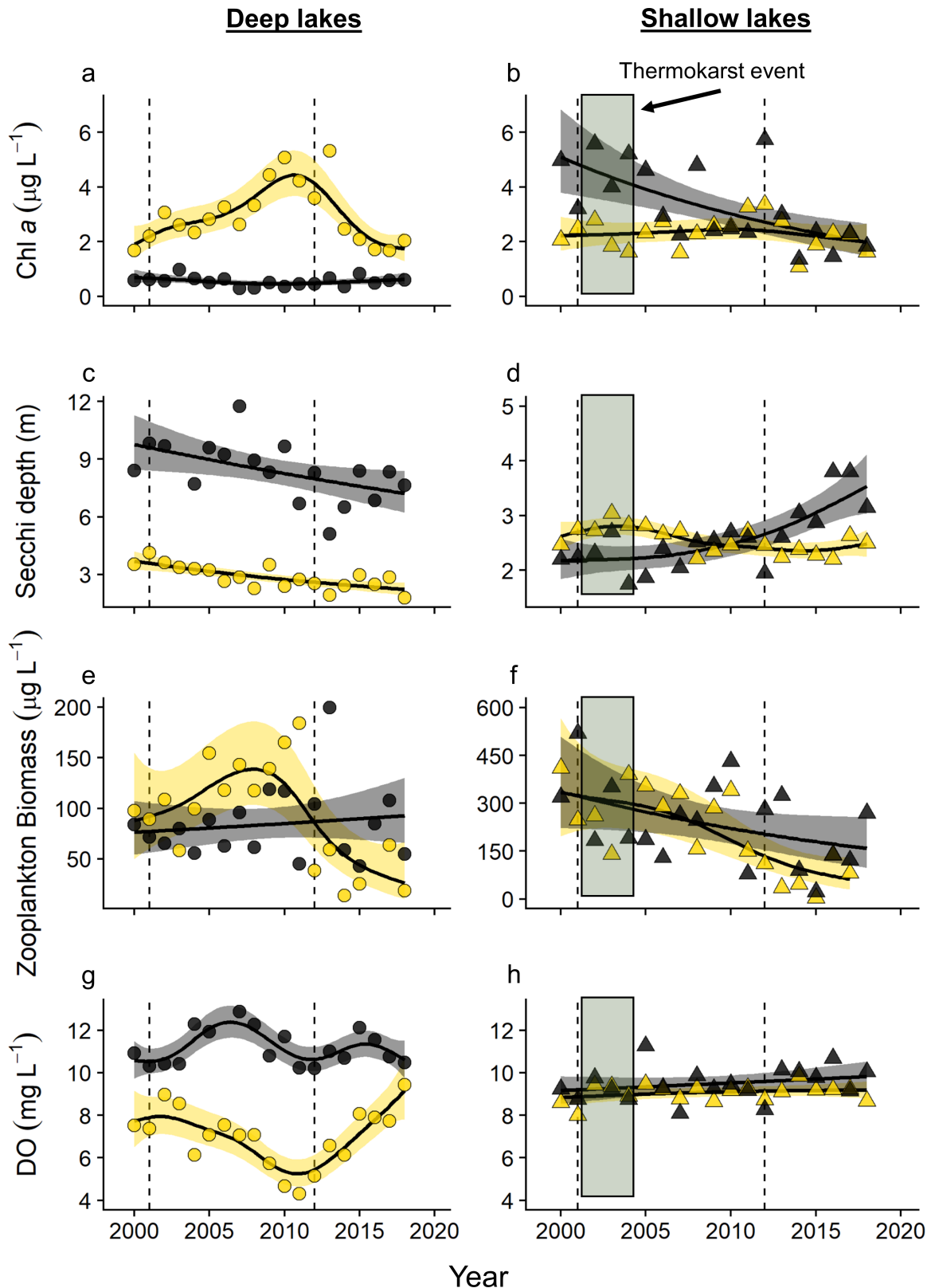
Fig. 2. Epilimnetic chlorophyll a (panels a,b ), water transparency (measured as Secchi depth) (panels c,d ), zooplankton biomass (panels e,f ), and hypolimnetic dissolved oxygen measured at 8 m (panel g ) and 2 m (panel h ). Deep lakes are on the left (circles) and shallow lakes are on the right (triangles). Fertilized lakes are shown in yellow symbols, and reference lakes are in black symbols. The dashed vertical lines indicate the start and end of the fertilization treatment, and the shaded boxes in the right panels represent a natural thermokarst event we observed in the shallow, reference lake. Trend Lines are smoothing splines with 95% confidence interval shading from generalized additive models. Some y-axis scales differ among panels. Note chlorophyll a from 2000 to 2003 represents total values uncorrected for phaeophytin.
