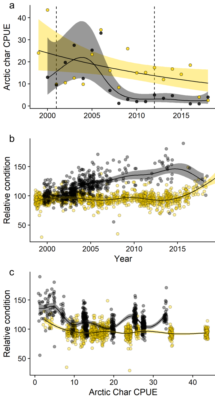
Fig. 5. (a) Fish catch per unit effort (CPUE) over time in the fertilized deep lake (yellow) and reference lake (black). The dashed vertical lines indicate the start and end of the fertilization. (b) Fish relative condition increased on average over time in the reference deep lake, and remained relatively constant in the fertilized deep lake. (c) Fish relative condition increased in both lakes once CPUE was <10. Lines are smoothing splines with 95% confidence intervals from generalized additive models. Output from generalized additive models is presented in Table 4.
