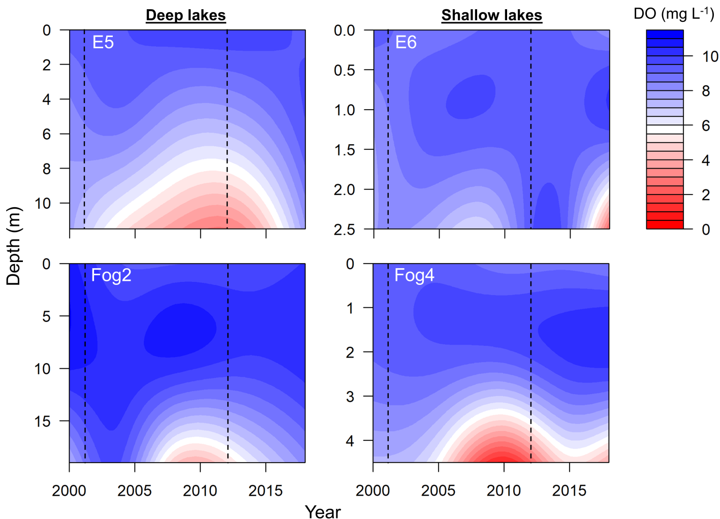
Fig. 3. Filled contour plots of dissolved oxygen concentration ( \text{mg L}^{-1} ) from profiles measured in deep (E5, Fog2) and shallow (E6, Fog4) lakes in July over time. The dashed vertical lines indicate the start and end of the fertilization treatment. A natural thermokarst event was observed in lake Fog4 from 2002 to 2004. Y-axes scales differ among panels.
