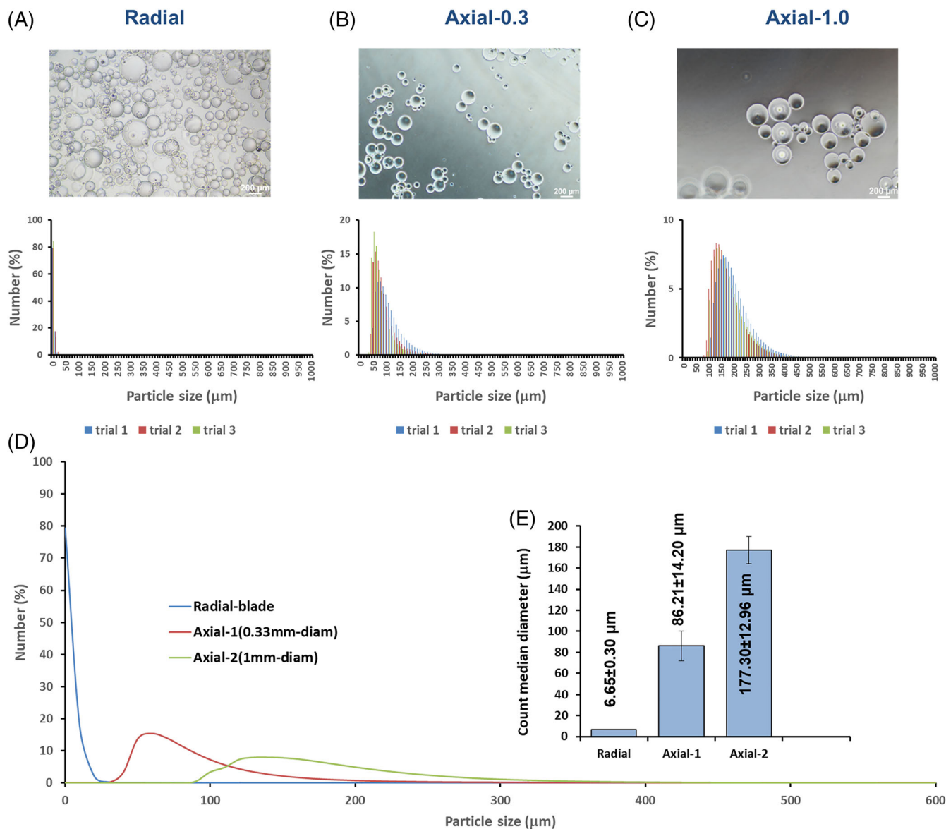
FIGURE 3 Effect of impeller geometry on microparticle size using a stirring rate of 500 rpm. Upper panels show brightfield optical microscopy and batch-to-batch size distribution of microparticles formed by (A) radial-blade, (B) 0.33 mm diameter axial-blade, and (C) 1.0 mm diameter axial-blade impeller geometries. Aggregate data are presented as (D) representative size distributions, and (E) median \pm SD for each impeller geometry
