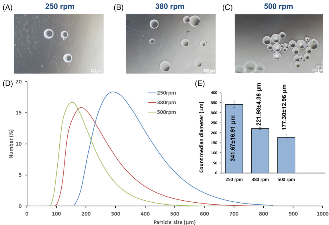
FIGURE 4 Effect of stirring rate on gelatin microparticle size using the Axial-1.0 impeller geometry. Upper panels show brightfield optical microscopy of microparticles formed at (A) 250 rpm, (B) 380 rpm, and (C) 500 rpm stirring rates. Aggregate data are presented as d) representative size distributions, and e) median ± SD for each stirring rate
