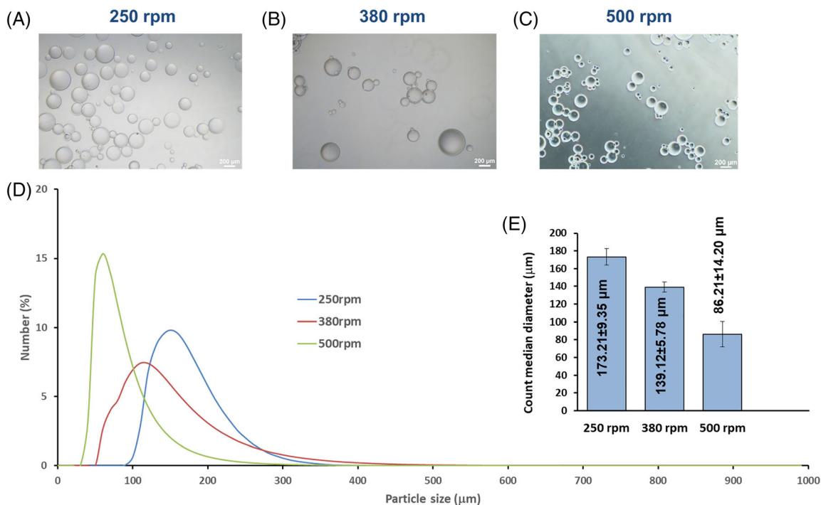
FIGURE 5 Effect of stirring rate on gelatin microparticle size using the Axial-0.3 impeller geometry. Upper panels show brightfield optical microscopy of microparticles formed at (A) 250 rpm, (B) 380 rpm, and (C) 500 rpm stirring rates. Aggregate data are presented as (D) representative size distributions, and (E) median ± SD for each stirring rate
