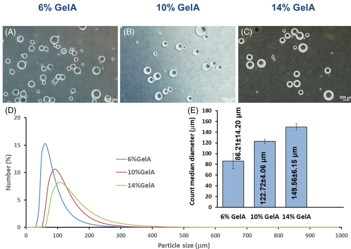
FIGURE 6 Effect of gelatin concentration on gelatin microparticle size using the Axial-0.3 impeller at 500 rpm. Upper panels show brightfield optical microscopy of microparticles formed at (A) 6.0% wt/vol, (B) 10.0% wt/vol, and (C) 14.0% wt/vol gelatin. Aggregate data are presented as (D) representative size distributions, and (E) median \pm SD for each gelatin concentration
