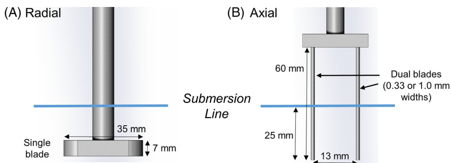
FIGURE 2 Comparative schematics of (A) radial-bladed impeller and (B) dual axial-bladed impellers. The axial-bladed impeller geometries used in this study differed only in blade cross-sectional dimensions, either 0.33 mm (Axial-0.3) or 1.0 mm (Axial-1.0)
