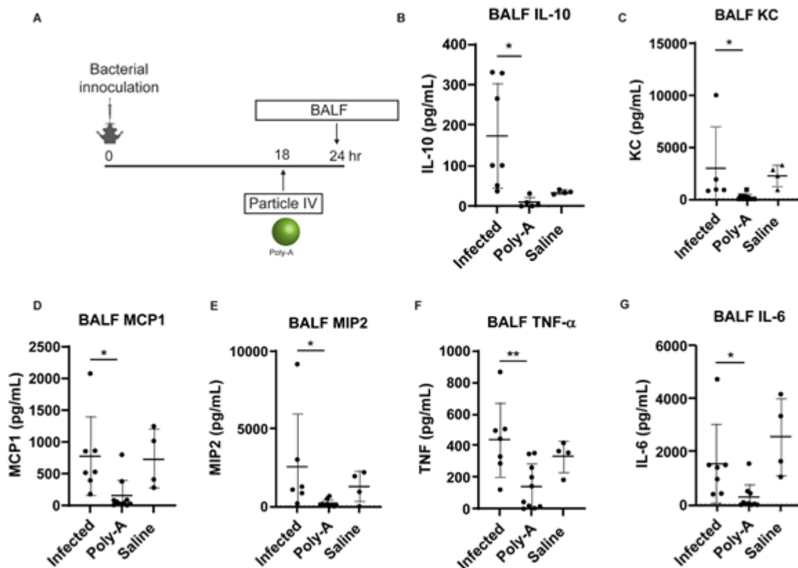
Figure 3. Cytokine and Protein Content in BALF of P. aeruginosa infected mice after 18-hour Poly-A injection, as measured by ELISA. (A) Schematic of Poly-A particle treatment and BALF protein sampling relative to the timing of bacterial infection. The concentration of (B) IL-10, (C) KC, (D) MCP1, (E) MIP2, (F) TNF- \alpha , and (G) IL-6 in the BALF of P. aeruginosa infected mice. Mice were injected with either 2 \times 10^8 Poly-A particles or saline at 18 hours post-infection, and samples were collected 24 hours post-infection. Statistical analysis was performed using GraphPad Prism Software using One-Way ANOVA with Fisher's LSD test with a 95% confidence interval. Asterisks indicate p values of: * = p < 0.05 , ** = p < 0.01 . N \geq 5 for all assays unless otherwise stated.
