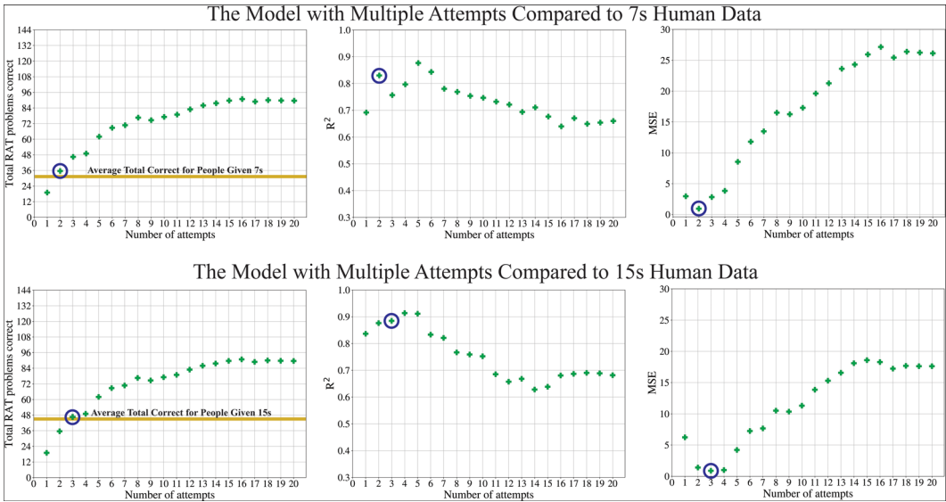
Fig. 3. The model with HBC using 1–20 attempts on the RAT presented in terms of the total number of problems correct, R^2 , and MSE for 7-s (top) and 15-s (bottom) human data.
