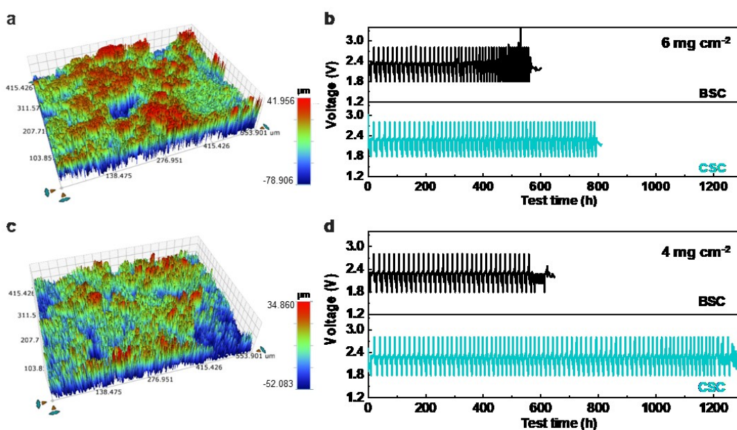
Figure 6 Optical profilometric images of CSC at S loading of 6 \text{ mg cm}^{-2} (a) and 4 \text{ mg cm}^{-2} (c). Discharge and charge profiles of the BSC and CSC at S loading of 6 \text{ mg cm}^{-2} (b) and 4 \text{ mg cm}^{-2} (d) in E/S = 4 \text{ mL g}^{-1} .
