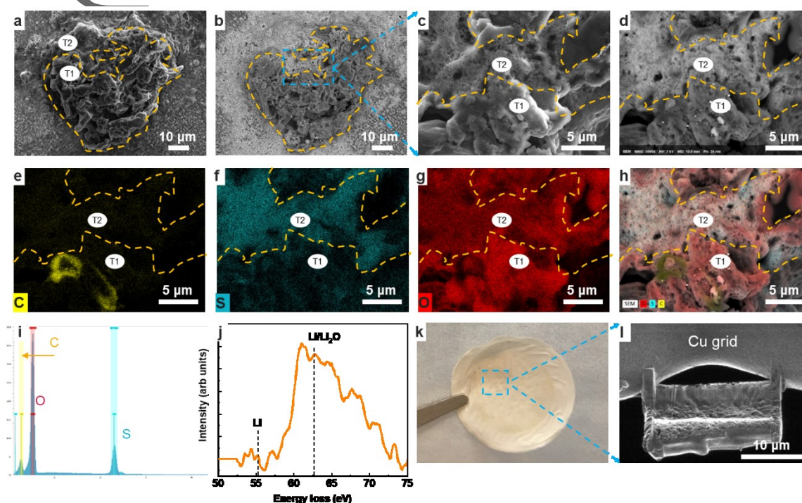
Figure 2 SEM, BSE, EDX, and EELS images of the particles on the separator surface facing cathode (coin cell in Figure 1a after charge failure). SEM (a) and BSE (b) images of T1 and T2. (c) and (d) magnified SEM and BSE images of the blue rectangular in Figure 2b. (e-h) EDX mapping of (c): red-O, blue -S, yellow-carbon, and their combination (h). (i) EDX spectrum of (c). (j) EELS image of the Li K-edge on T1. (k) Digital photograph of the used separator with the top side facing S cathode. (l) SEM/focused ion beam (FIB) cross-section image of particles on separator for EELS.
