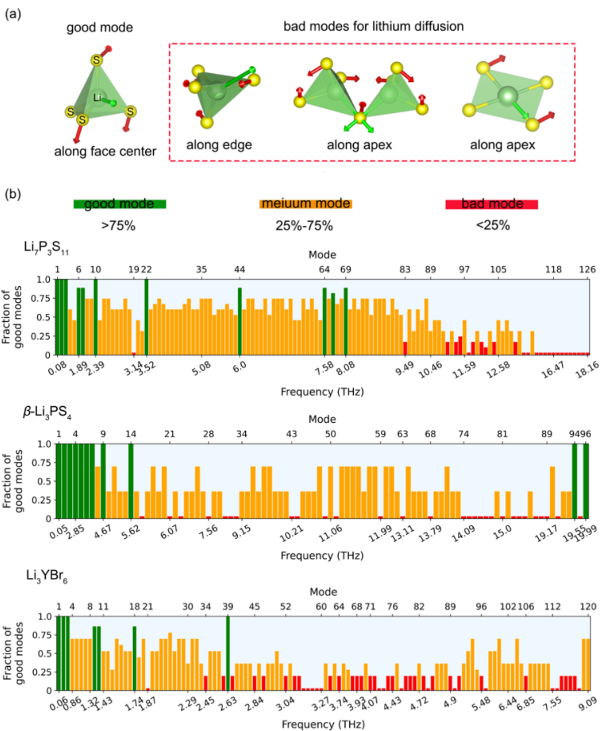
Figure 3. Vibrational modes for Li ion diffusion. (a) Schematic diagrams of the good and bad vibrational mode for lithium ion diffusion in \beta\text{-Li}_3\text{PS}_4 , (b) the frequency distributions of the good,
