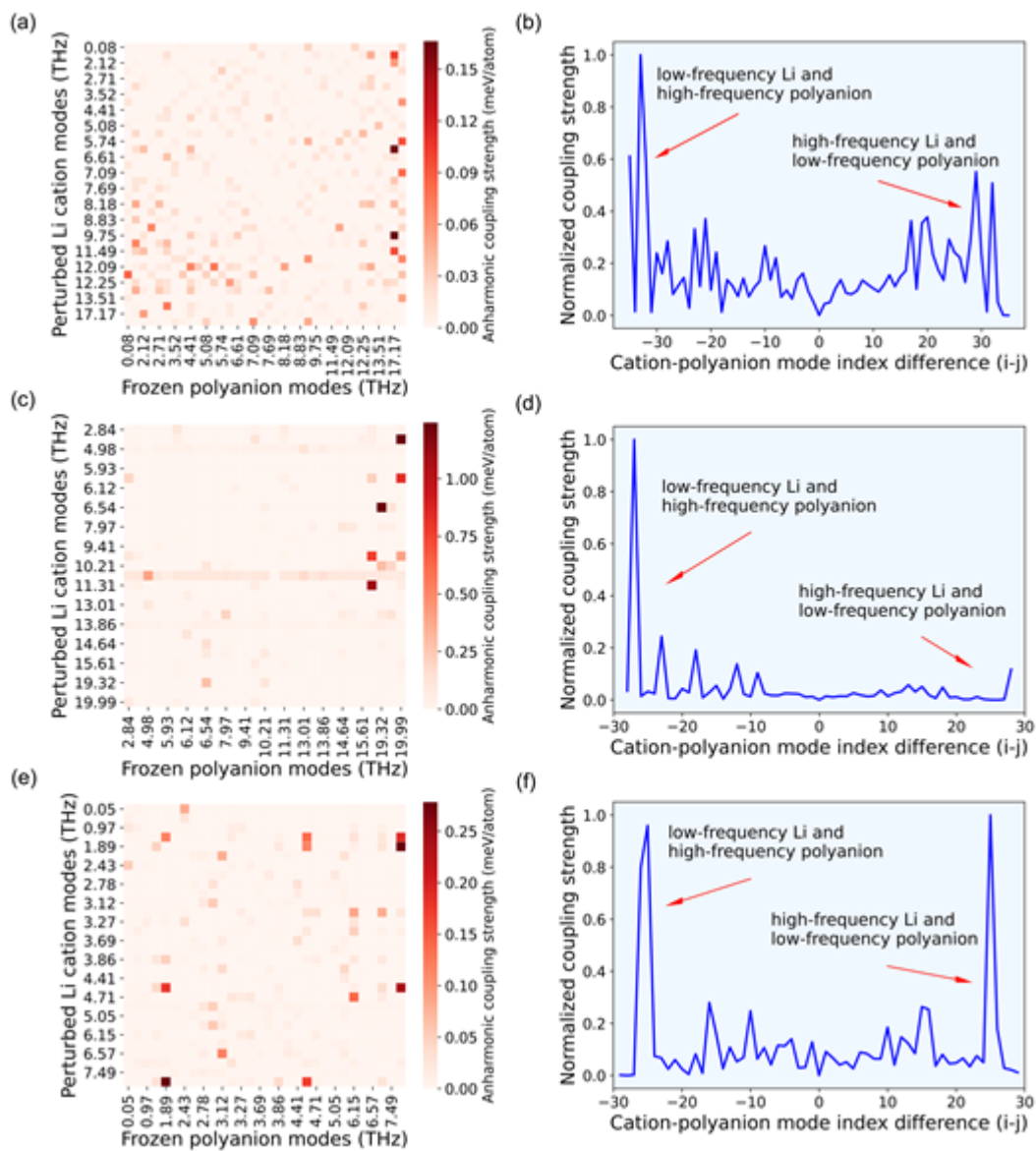
Figure 4. Interactions between phonon mode anharmonic coupling. Anharmonic cation-polyanion phonon mode coupling for (a) \text{Li}_7\text{P}_3\text{S}_{11} , (c) \beta\text{-Li}_3\text{PS}_4 and (e) \text{Li}_3\text{YBr}_6 , respectively. Normalized coupling strengths of these pairs of cation-polyanion modes with the same mode index difference ( i-j , i and j are the index for cation and polyanion modes, respectively) for (b) \text{Li}_7\text{P}_3\text{S}_{11} , (d) \beta\text{-Li}_3\text{PS}_4 and (f) \text{Li}_3\text{YBr}_6 , respectively. The frequency increases with the increase of mode number. The large normalized coupling strength of the pair of cation-polyanion modes with a large positive i-j means the strong coupling interaction between the low-frequency Li modes and the high-frequency polyanion modes;
