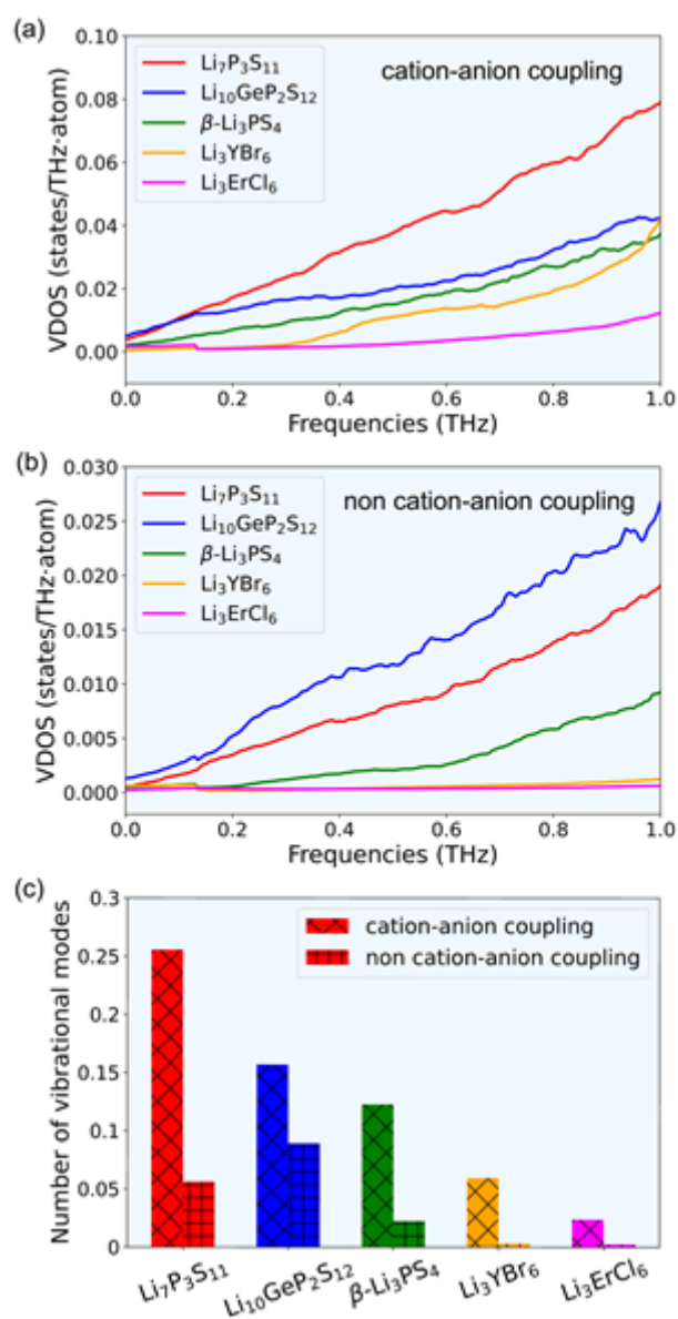
Figure 2. (a-b) Low-frequency (< 1 THz) Li VDOS of five lithium superionic conductors with and without cation-anion coupling; (c) the mode number integrated from the low-frequency (< 1 THz) Li VDOS with and without cation-anion coupling, respectively.
