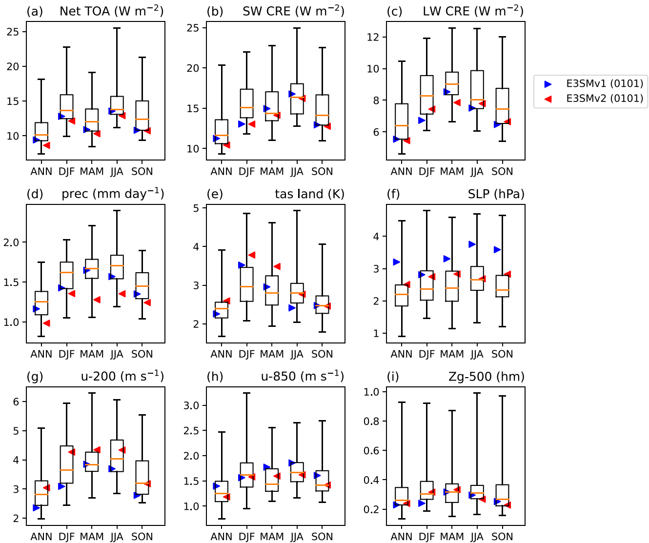
Figure 7. Comparison of RMSEs (1985–2014) of an ensemble of 52 CMIP6 models (first historical members r111p1f1) with the first historical members of E3SMv1 (blue triangles) and E3SMv2 (red triangles). Box and whiskers show 25th, median, 75th percentile, minimum, and maximum RMSE for the CMIP6 ensemble. Spatial RMSE against observations are computed for annual and seasonal averages with the E3SM Diagnostics package (C. Zhang et al., 2022). Fields shown include TOA net radiation (a), TOA SW and LW cloud radiative effects (b, c), precipitation (d), surface air temperature over land (e), sea-level pressure (f), 200 and 850 hPa zonal wind (g, h), and 500 hPa geopotential height (i). TOA, top-of-atmosphere; SW, shortwave; CRE, cloud radiative effects; LW, longwave; DJF, December–February; MAM, March–April; JJA, June–August; SON, September–November; RMSE, root-mean-square error. The mean climatology of the reference observational and reanalysis data sets are derived from: CERES-EBAF Ed4.1 (Loeb et al., 2018; 2001–2014) for (a–c), GPCP2.3 (Adler et al., 2018; 1985–2014) for (d) and ERA5 (Hersbach et al., 2020; 1985–2014) for (e–h). Due to data availability, not all models are included for every variable. Complete data is available in Table S1.
