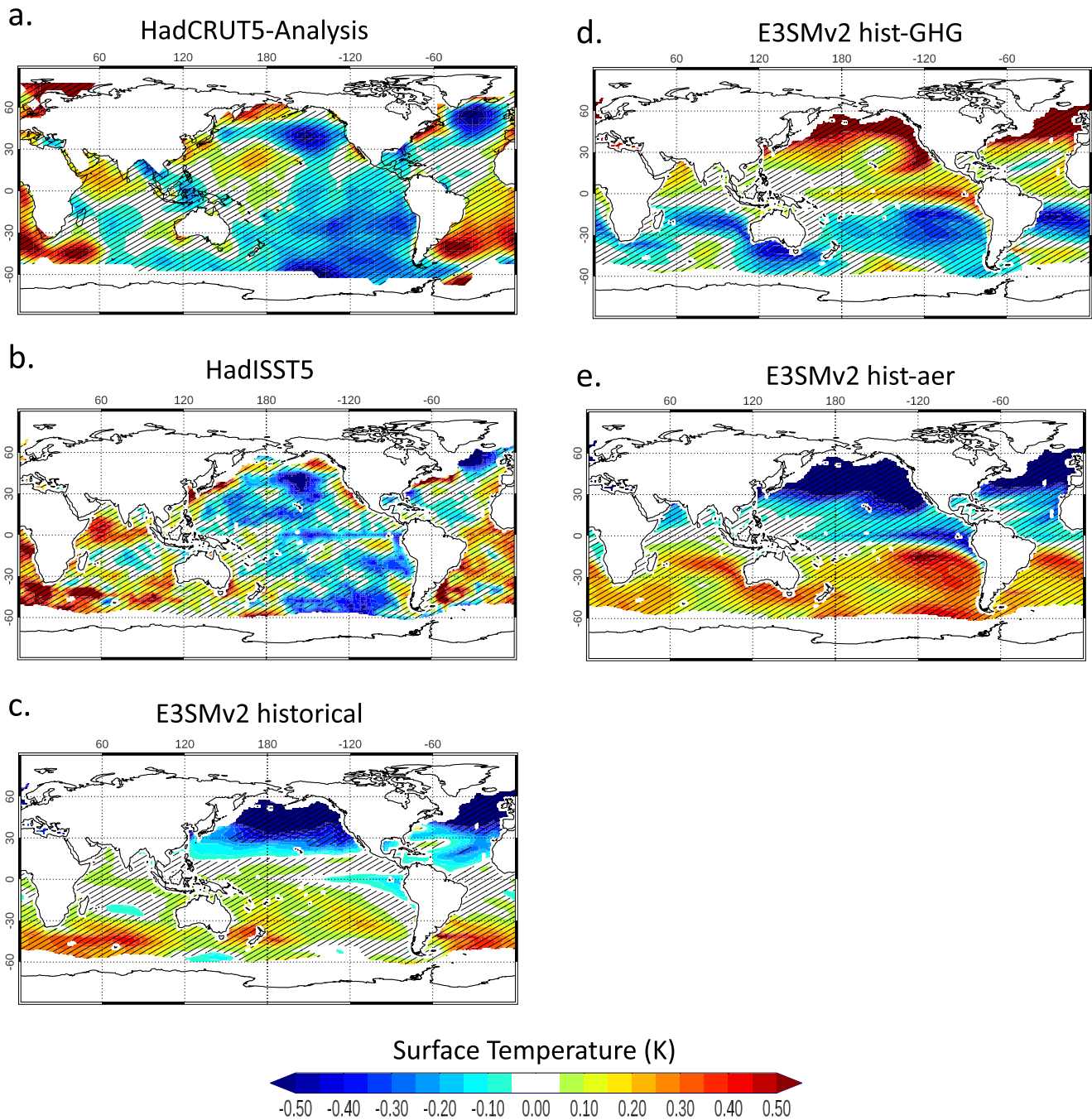
Figure 24. Difference in SST between 1980–2014 and 1870–1904 relative to the tropical mean change between the two periods for (a) HadCRUT5 data, (b) HadISST data, (c) E3SMv2 historical ensemble, (d) E3SMv2 hist-GHG ensemble, and (e) hist-aer ensemble. Hatched areas indicate regions where the difference is statistically significant at the 95% confidence level based on a two-tailed Student's t test.
