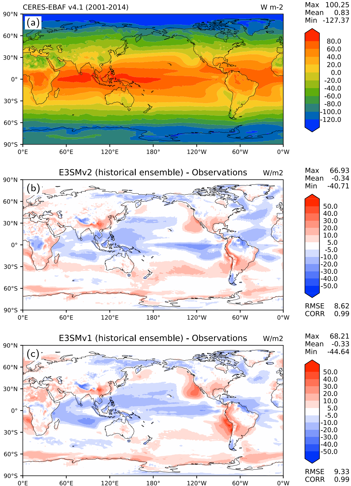
Figure 8. Annual net top-of-atmosphere (TOA) radiative flux ( W\ m^{-2} ): (a) CERES-EBAF Ed4.1 observational estimate (2001–2014), (b) model bias from the 5-member ensemble of E3SMv2 historical coupled simulations (2001–2014), and (c) model bias from the 5-member ensemble of E3SMv1 historical coupled simulations (2001–2014). RMSE, root-mean-square error; CORR, linear correlation coefficient between observation and model.
