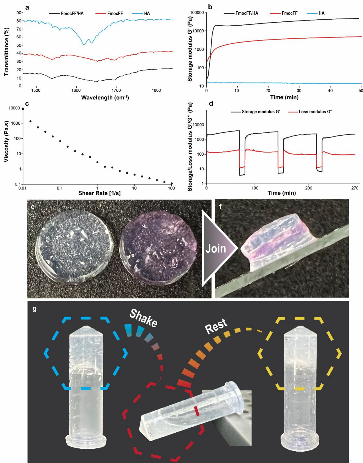
Figure 2. Rheological and FTIR analyses of FmocFF/HA composite hydrogel. (a) FTIR spectra of FmocFF/HA, FmocFF and HA. (b) In situ time sweep oscillation measurements of the FmocFF, HA, and the composite FmocFF/HA hydrogel. (c) Viscosity versus shear rate of the FmocFF/HA composite hydrogel. (d) Time sweep when alternate step strain switched from 0.1% to 100%. (e, f) Digital images demonstrating the self-healing properties of separate layers of the composite hydrogel. (g) Inverted test-tube showing the self-healing property of the hydrogel after mechanical breaking.
