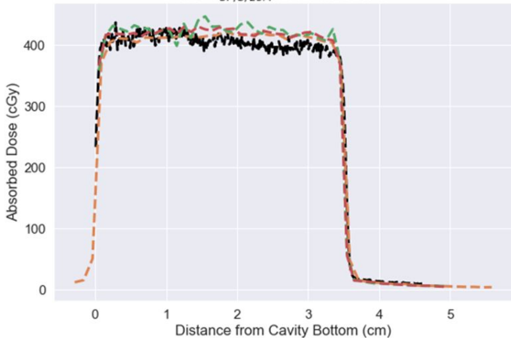
Lu177 SF, S, 25.4 #3 Horizontal Profile
