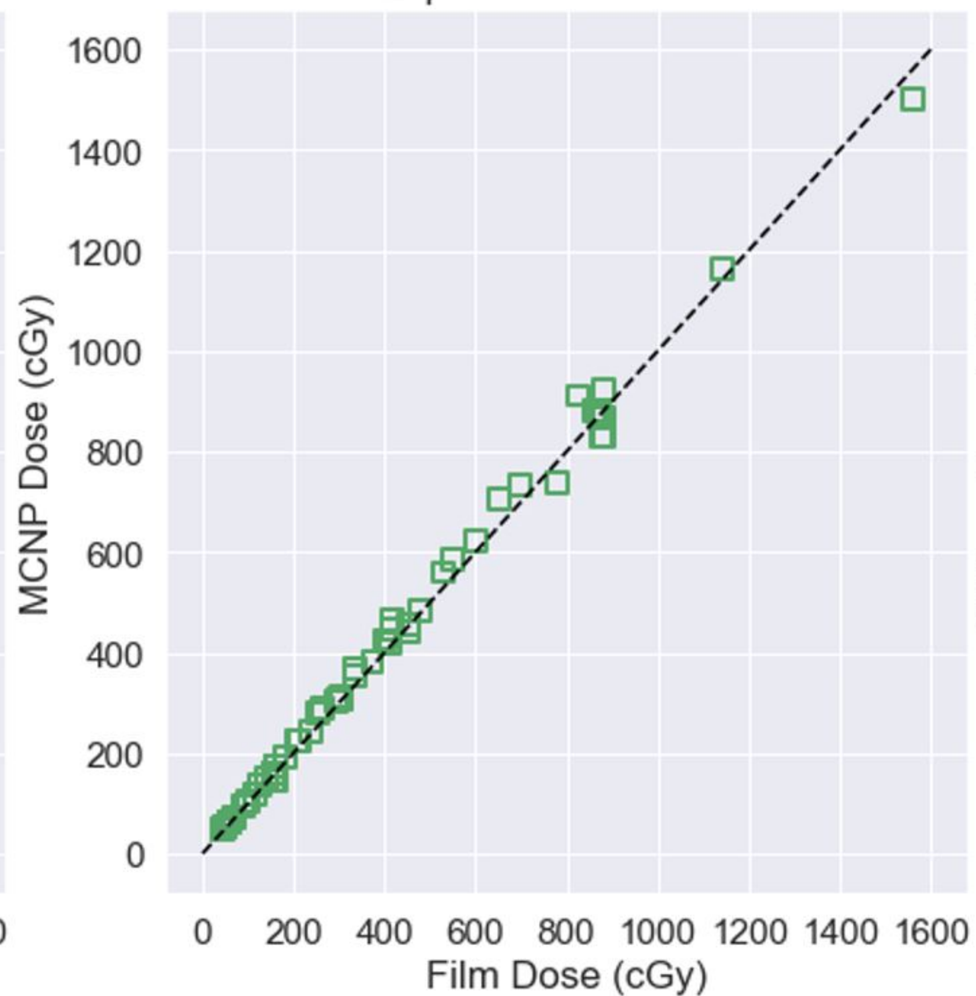
Experiment vs MCNP
