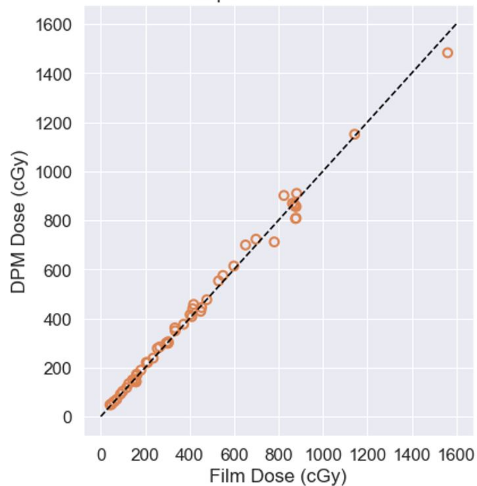
Experiment vs DPM
