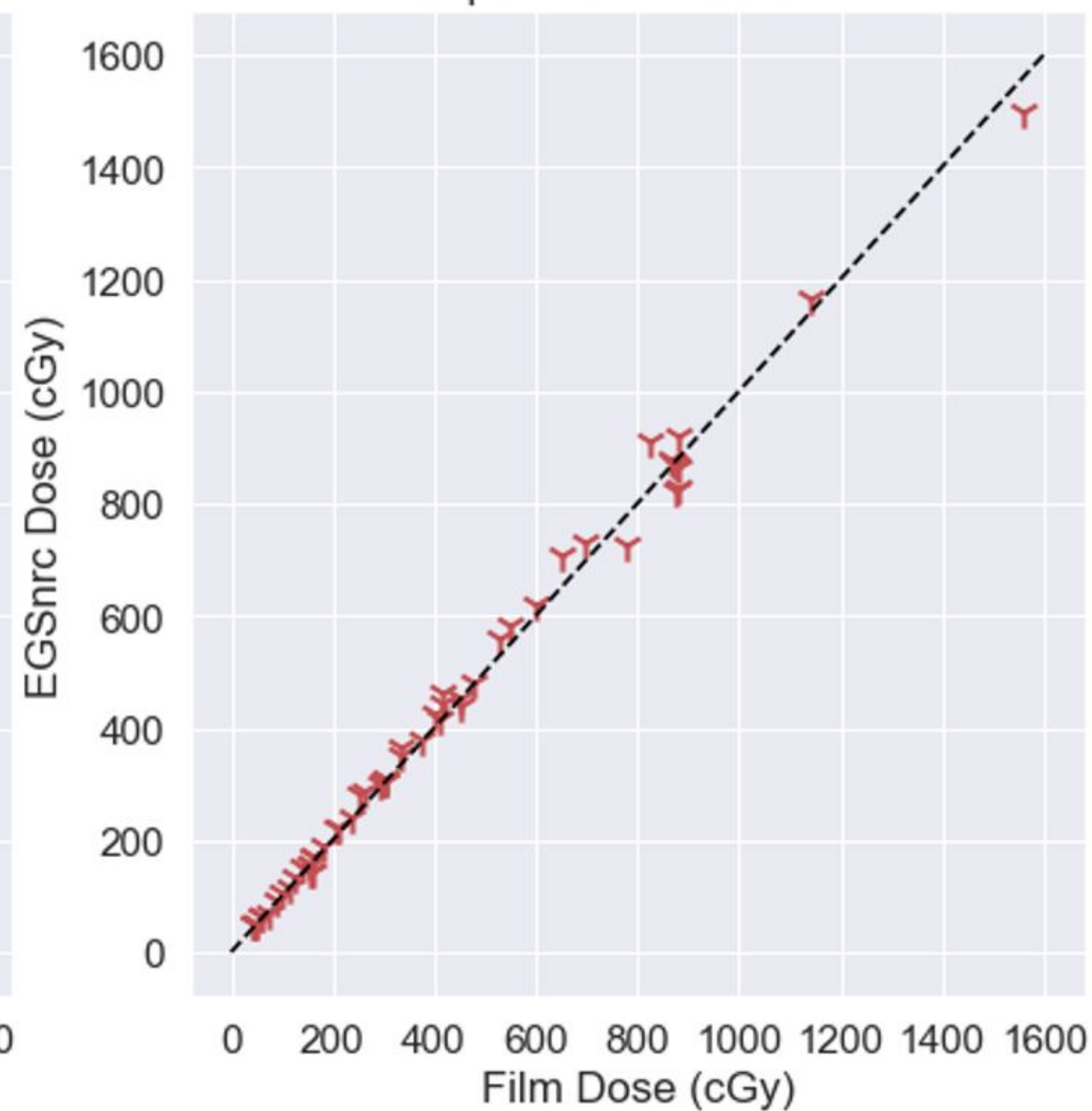
Experiment vs EGSnrc
