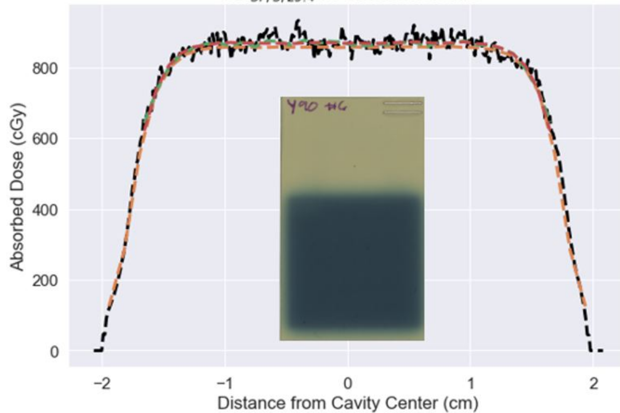
Y90 SF, S, 25.4 #3 Horizontal Profile
