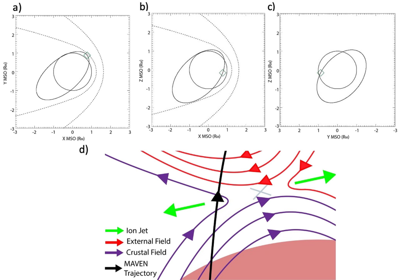
Figure 5. Mars Atmosphere and Volatile EvolutionN (MAVEN) orbit as viewed from the Z_{\text{MSO}} plane (a), Y_{\text{MSO}} plane (b), and X_{\text{MSO}} (c) plane. The green diamond in panels (a–c) represent the location of the current sheet. The dashed lines in panels (a–c) show the nominal locations of the bowshock and magnetic pileup boundary from Trotignon et al. (2006). Schematic of reconnection region and ion jet outflow with colored arrows representing the ion jet (green), crustal magnetic field orientation (purple), external field orientation (red), and the trajectory of the spacecraft (black) (d).
