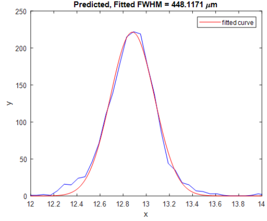
(b) X cross-section of events in pixel (7,3) predicted by a narrow neural net trained on data from all inner 9\times 9 pixels. The measured position resolution in X is 422\ \mu\text{m} after deconvolving the response of the collimator, a \sim 25\ \mu\text{m} improvement over the traditional techniques.
