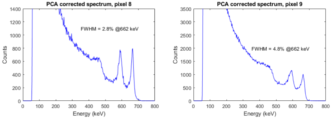
Figure 5.35: PCA-corrected spectra from pixels 8 and 9 of UNC-1. Resolutions are 2.8% and 4.8% at 662 keV, an improvement over the standard drift time corrections of Figure 5.18.
