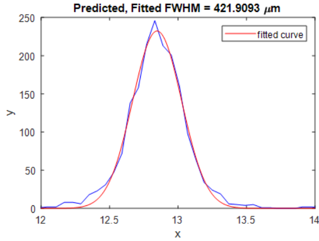
(c) X cross-section of events in pixel (7,3) predicted by a narrow neural net trained on data from this particular pixel. The measured position resolution in X is 395\ \mu\text{m} after deconvolving the response of the collimator, a \sim 50\ \mu\text{m} improvement over the traditional techniques.
