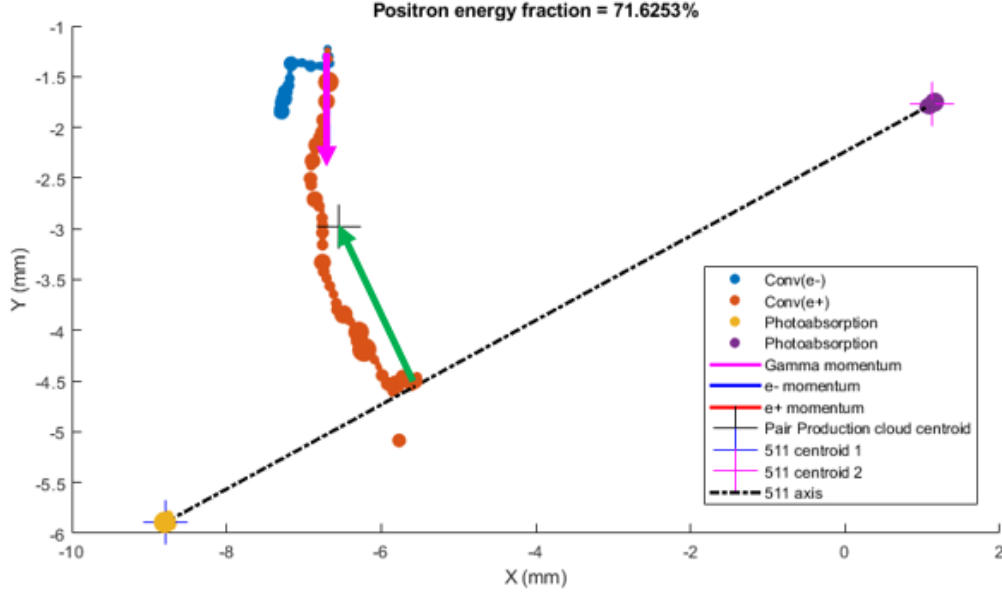
Figure 4.8: Simulated charge cloud detail for a pair production event in which the positron had 72% of the total available kinetic energy.
