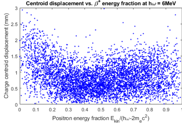
Figure 4.11: Charge cloud displacement from 511 axis vs. positron energy fraction for simulated pair production events from a 6 MeV photon beam.
