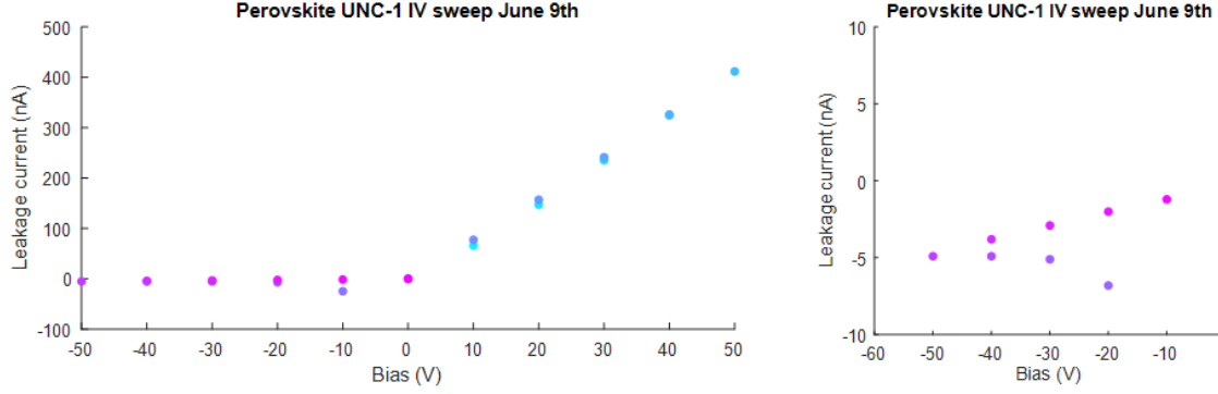
Figure 5.16: I-V scan of the solution grown perovskite samples of Figure 5.15. (Left) entire range, (right) reverse bias region. Bias was applied to the planar Au contact. The sweep tracked from 0V to +50V, back down to 0V and -50V, then returned to 0V (blue to purple to pink in the figure).
