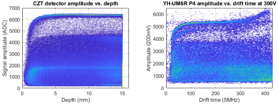
(a) Typical plot of pixel signal amplitude vs. depth for a CZT detector exposed to ^{137}\text{Cs} . (b) Plot of pixel signal amplitude vs. drift time for YH-UM6R, the furnace grown \text{CsPbBr}_3 detector from Figure 5.9, exposed to ^{137}\text{Cs} .
