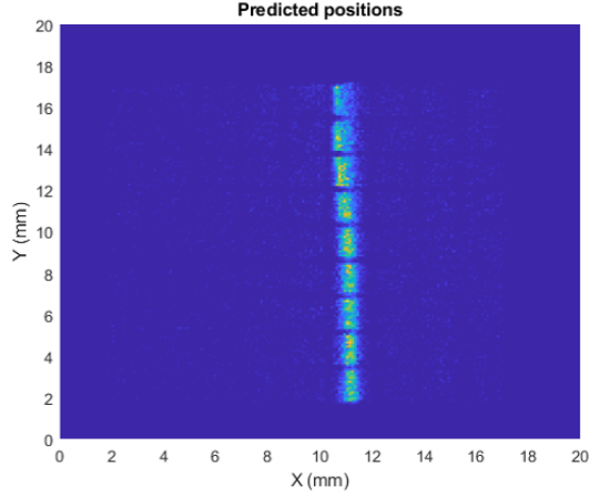
(a) Distribution of subpixel XY positions for irradiation with a 100\ \mu\text{m} slit collimator, predicted using a narrow neural net trained on aggregate data from all inner 9\times 9 pixels.
