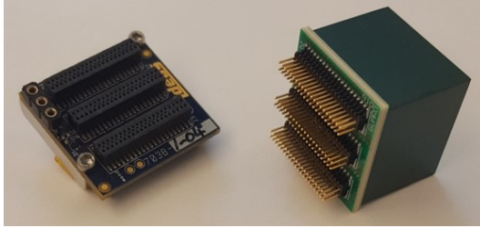
(a) VAD_UMv2.2 ASIC (left) and standard attach CZT detector module (right).
