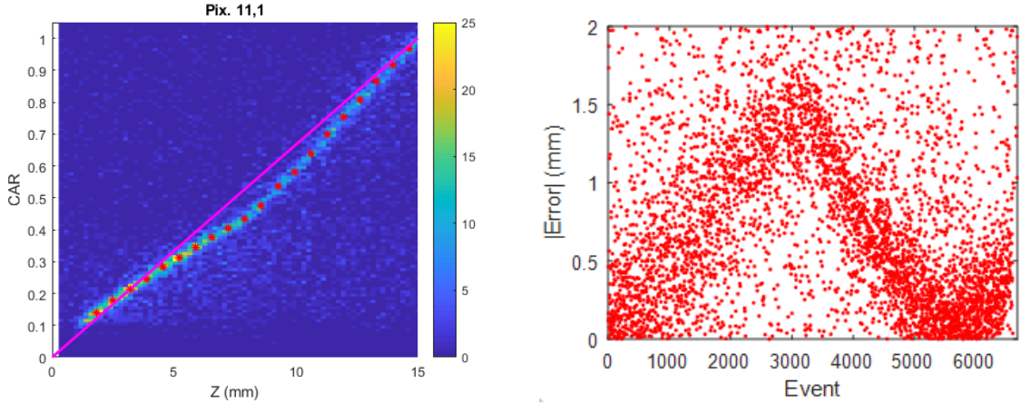
(a) Calculated position from cathode/anode ratio vs. true collimator position for a corner pixel, (11,1). There is significant deviation in the middle, mostly due to the nonideal weighting potential. (b) Absolute error between calculated and measured Z coordinates above the corner pixel (11,1).
