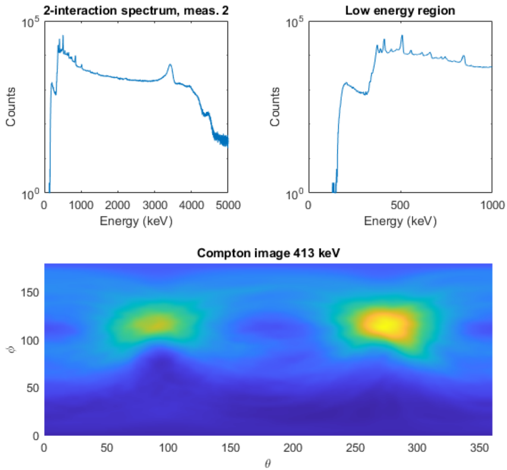
Figure 4.19: 2-interaction spectrum for experiment 2 and Compton image of the 413 keV peak.
