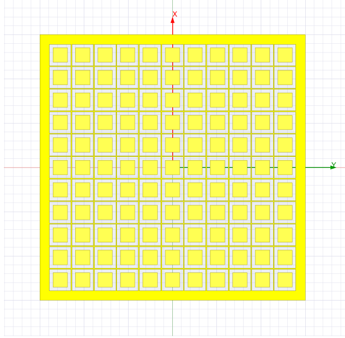
Figure 3.5: Pixel pattern with inter-pixel grid, used by older generation CZT detectors.
