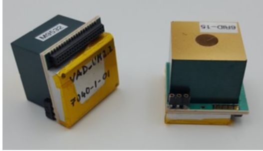
(b) Direct attach module with VAD_UMv2.2 ASIC and CZT crystal bonded to the same substrate board.
