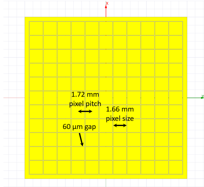
Figure 3.4: Fine detail of the pixel pattern used with the CZT detectors in this work. The pitch between pixels is 1.72 mm, while the pixel size is 1.66 x 1.66 mm 2 . The resulting gap is 60 \mu m wide.
