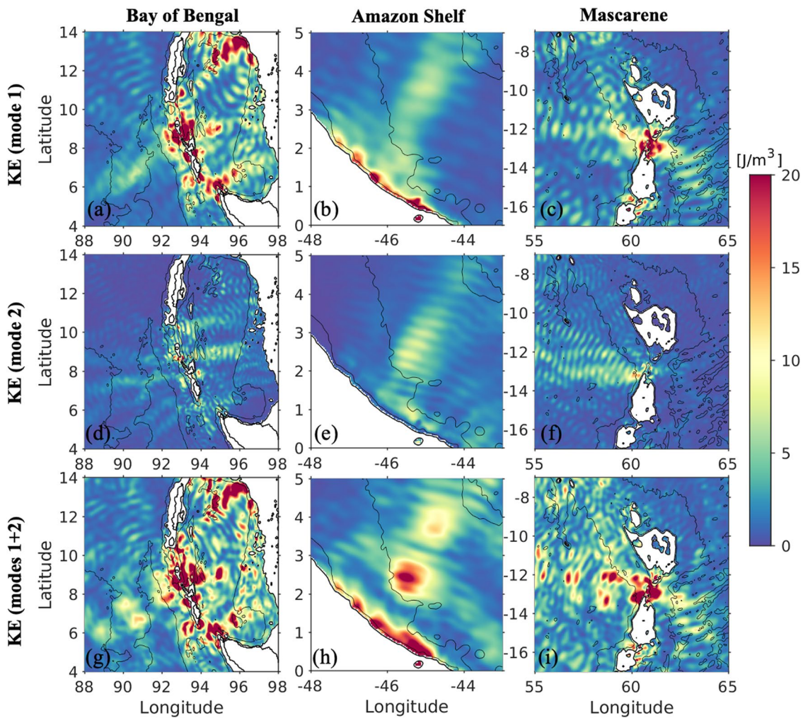
Figure 11. Time-mean surface kinetic energy ( J/m^3 ) for mode 1 at (a) the Bay of Bengal and Andaman Sea, (b) the Amazon Shelf, and (c) the Mascarene Ridge, (d–f) for mode 2 and (g–i) the sum of modes 1 and 2 for the same three areas. The contour lines mark the 0, 250, 1,000, and 3,500 m sea-floor depths.
