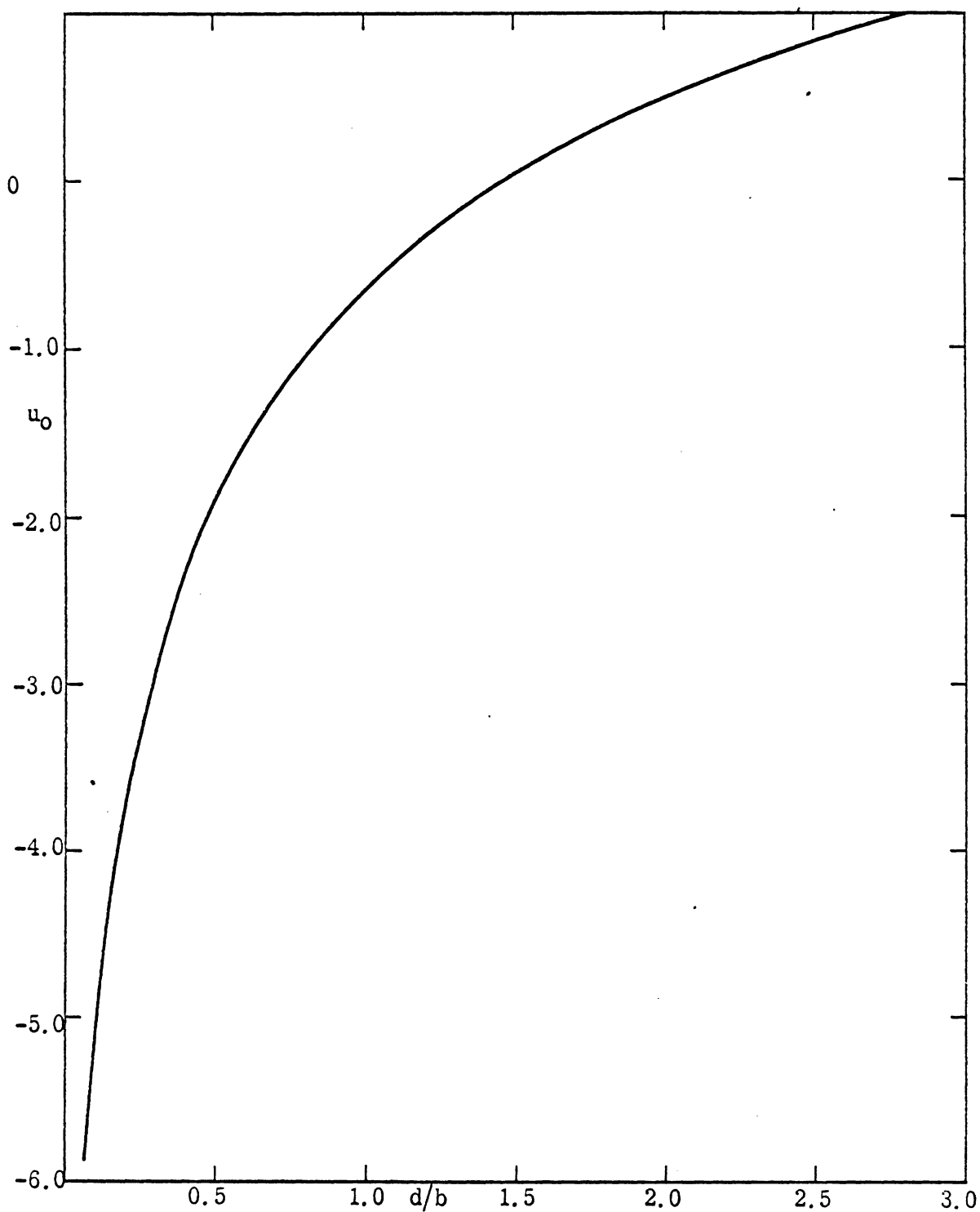
FIG. 2-2: Variation of the Ground Proximity Factor u_0 as a Function of d/b , where d/b is the normalized ground proximity distance.
