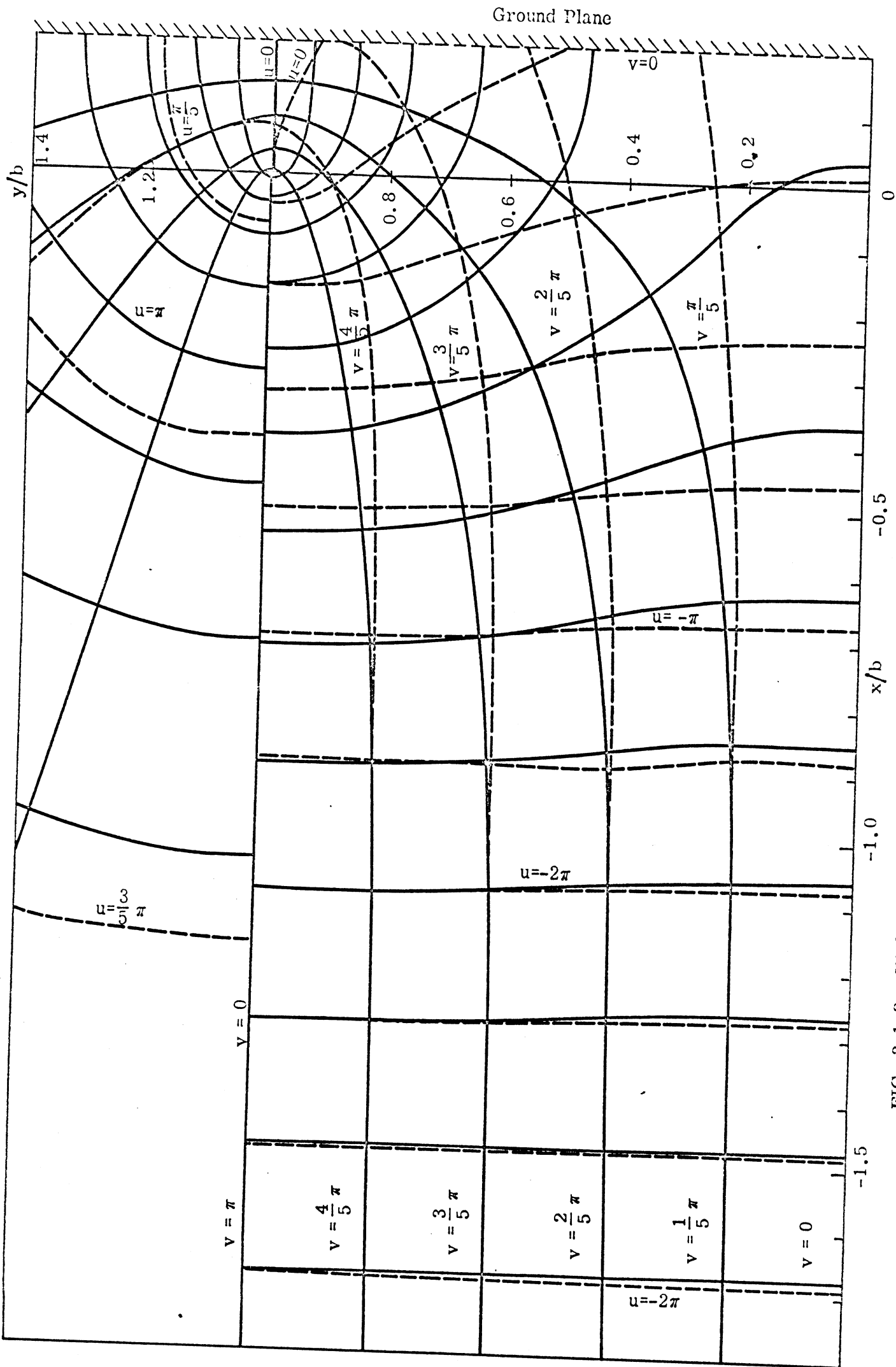
FIG. 3-1-2. Field Lines, d/b = 0.2 .
