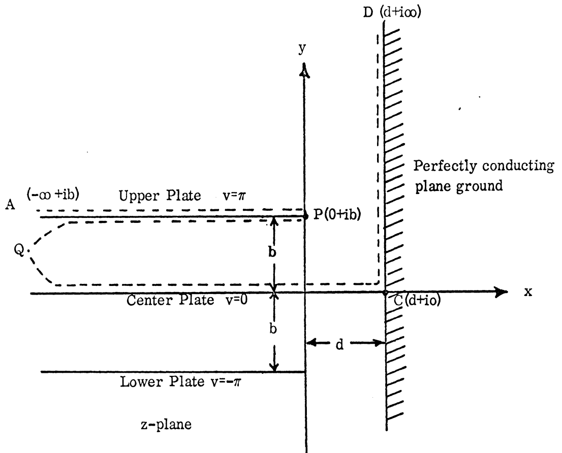
FIG. A-1: A semi-infinite parallel plate transmission line system in the z -plane in the presence of the perfectly conducting ground.
