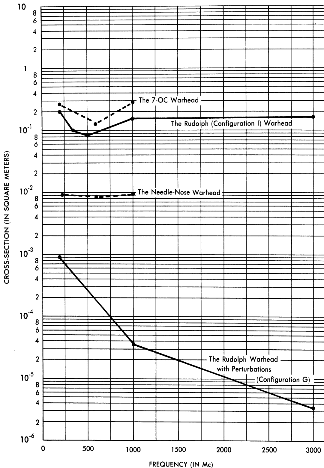
FIG. 3-2 THEORETICAL NOSE-ON CROSS-SECTIONS AS A FUNCTION OF FREQUENCY
