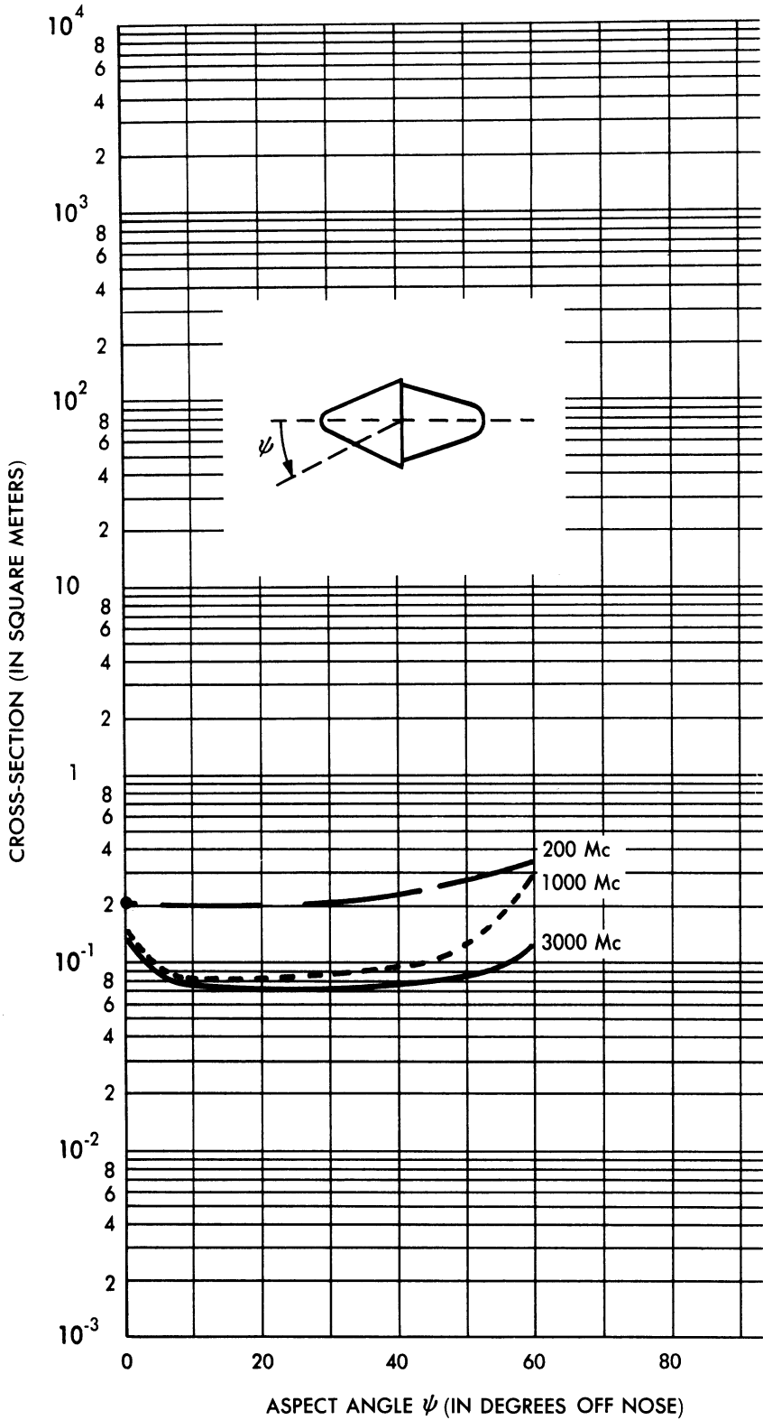
FIG. 2-3 CROSS-SECTION OF ONE OF THE PARAMETERIZATIONS FOR THE RUDOLPH WARHEAD (CONFIGURATION I) AS A FUNCTION OF ASPECT AND FREQUENCY
