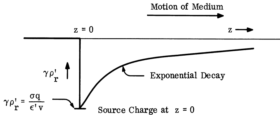
FIG. 3-2: RESPONSE CHARGE DENSITY ALONG THE z -AXIS FOR A POINT SOURCE CHARGE AT THE ORIGIN.
