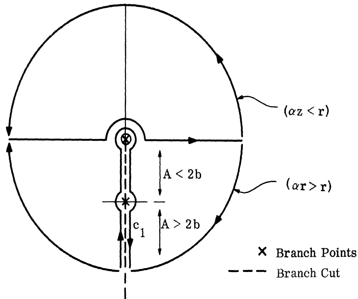
FIG. 4-3: CONTOURS IN THE h -PLANE FOR EVALUATING G(\bar{R}|0) .
