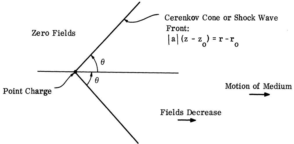
FIG. 4-4: CERENKOV CONE GEOMETRY FOR HIGH VELOCITIES.
