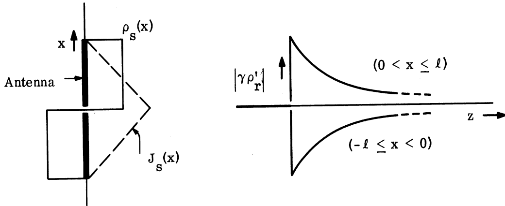
FIG. 3-3 : CHARGES AND CURRENTS FOR A THIN-WIRE ANTENNA.
