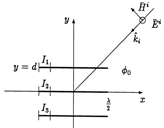
Fig. 2. Three parallel strips R_n = R_0
