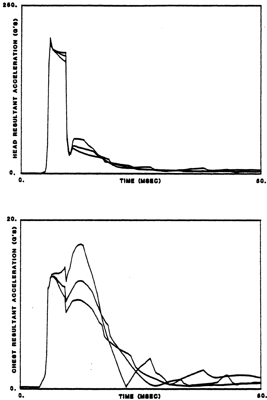
FIGURE 3-7. Comparison of Head and Chest Response for Extreme Variations in Neck Torque.
