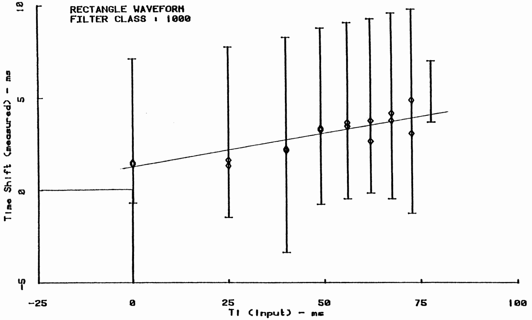
FIGURE 2-5. Representative Facility Time Accuracy Performance.
