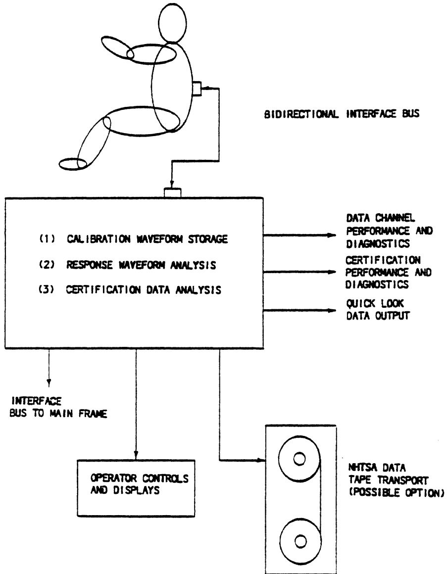
FIGURE 2-10. AATD Test Set.
