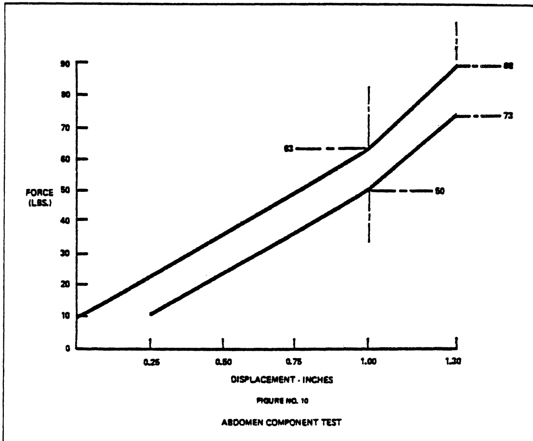
FIGURE 3-3. Abdomen Component Test Measurement Criteria.
