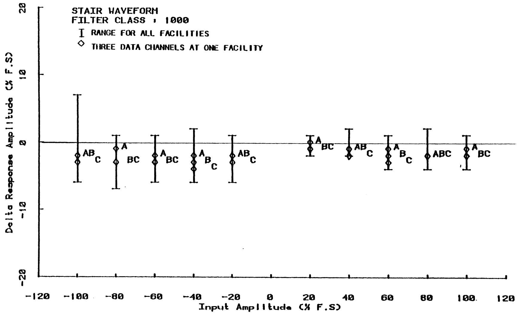
FIGURE 2-2. Facility with Representative Amplitude Error Performance.
