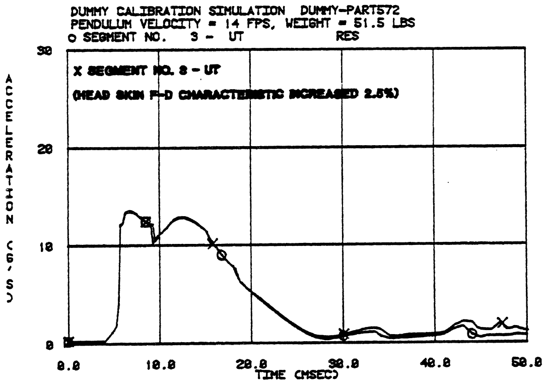
FIGURE 3-9. Comparison of Head and Chest Response for a 2.5% Change in Head-Skin F-D Characteristic.
