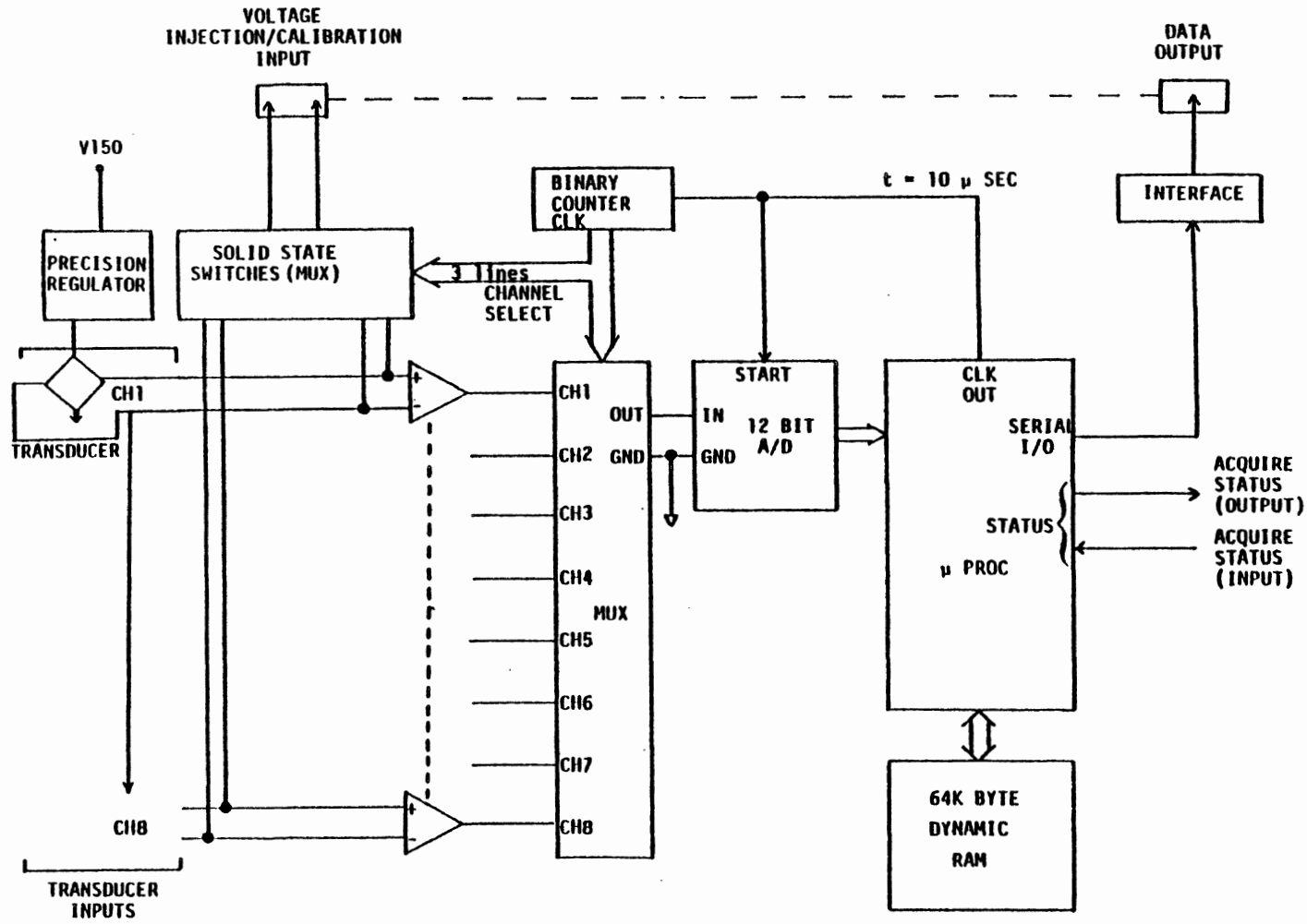
FIGURE 3-6. Data Acquisition Module Block Diagram.
