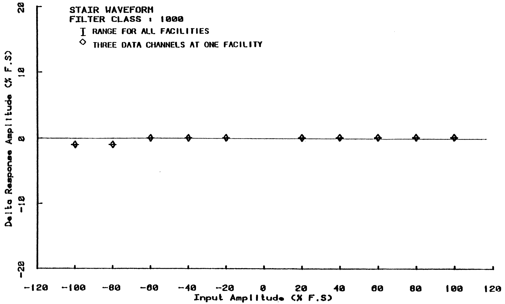
FIGURE 2-4. Amplitude Accuracy Performance for MGA Data Acquisition System.
