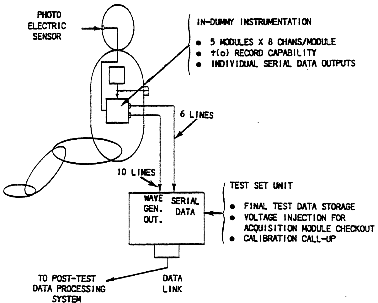
FIGURE 3-5. Full System Concept.
