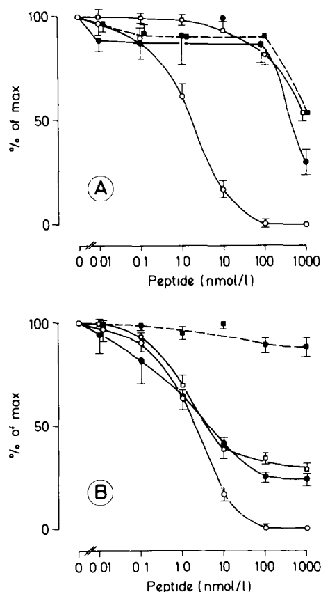
Fig. 2. Inhibition of binding of ^{125}\text{I} -labelled GLP-1(7-36)amide to lung membranes by GLP-1(7-36)amide ( \circ ) ( n = 4 ). (A) GLP-1(1-36)amide ( \bullet ) ( n = 4 ), glucagon ( \blacksquare ) ( n = 6 ) and GLP-2 ( \square ) ( n = 6 ). (B) VIP ( \bullet ) ( n = 5 ), PHI ( \square ) ( n = 6 ) and oxyntomodulin ( \blacksquare ) ( n = 6 ). Data points show means \pm SE.
