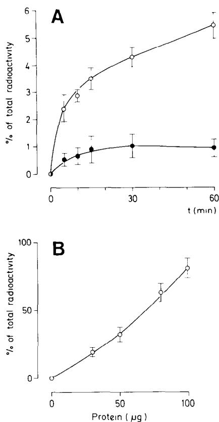
Fig. 1. (A) Specific binding of ^{125}\text{I} -labelled GLP-1(7-36)amide to lung membranes (1 mg/ml) at 37°C ( \circ ) and 10°C ( \bullet ) (means \pm SE, n = 4 ). (B) Specific binding of ^{125}\text{I} -labelled GLP-1(7-36)amide to lung membranes as a function of protein concentration (means \pm SE, n = 4 ).
