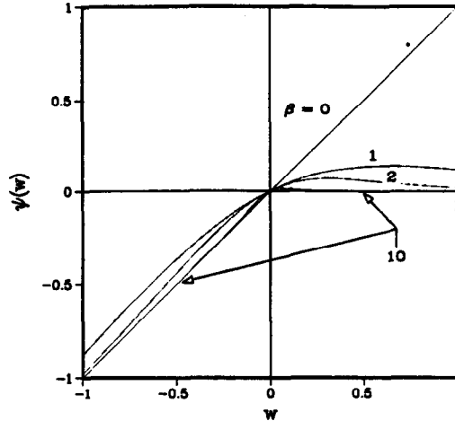
Fig. 3. Displacement function that characterizes the foundation model \Psi(w) as a function of w for different values of \beta .
