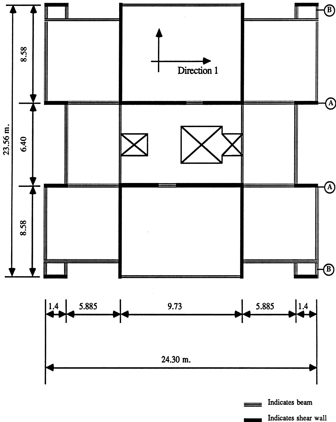
Fig 6.1(a) : Plan View of a Typical Story of Almendral Building.
