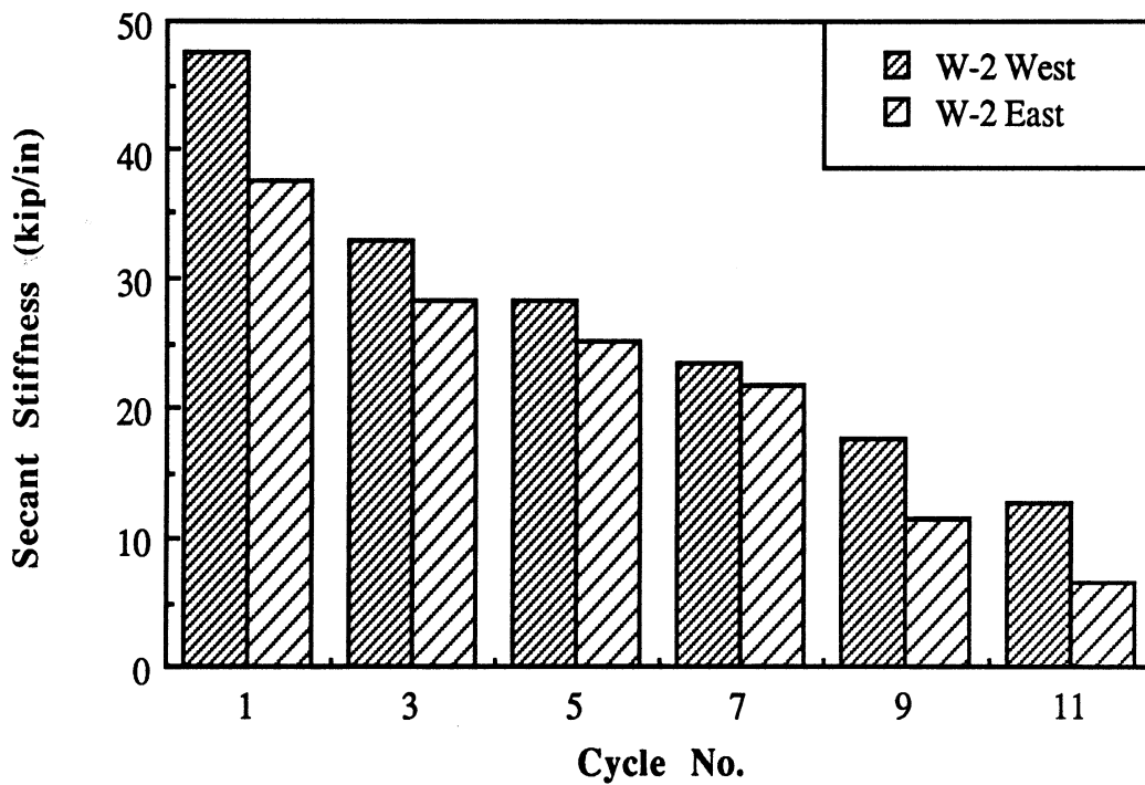
Fig. 4.41 : Comparison of Secant Stiffnesses for Wall W-2.
