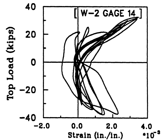
Fig. 4.70(b) : Strain Histories for Gages 8, 9, 10, 12, 13 and 14 in Wall W-2.
