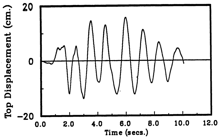
(b) Top Displacement Time History
