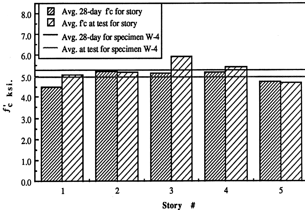
Fig. 3.17(d) : Variation of Concrete Compressive Strength for Wall W-4.
