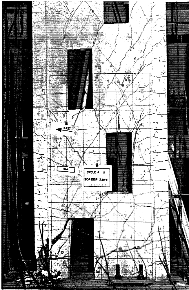
Fig. 4.38 : General Condition of Specimen W-4 during the Last Cycle.
