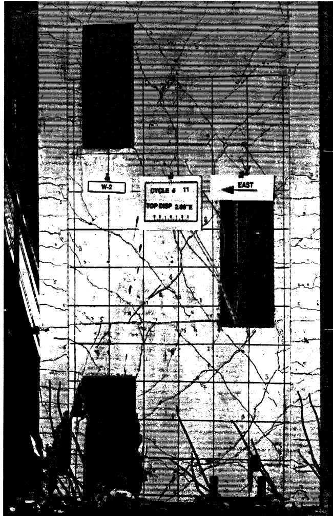
Fig. 4.17 : Crushing on the West Edge of Opening is Accompanied by Buckling of Reinforcement Bars during Cycle 11.
