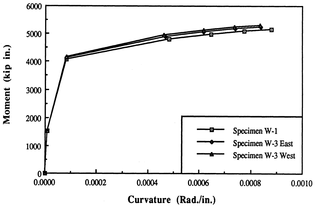
Fig. 5.2 : Comparison of Moment-Curvature Relationships for Walls W-1 and W-3.
