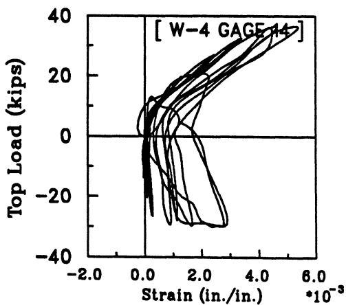
Fig. 4.73(b) : Strain Histories for Gages 8, 9, 10, 11, 12 and 14 in Wall W-4.
