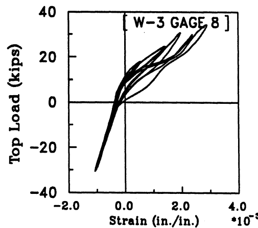
Fig. 4.72(a) : Strain Histories for Gages 1, 2, 5, 6, 7 and 8 in Wall W-3.
