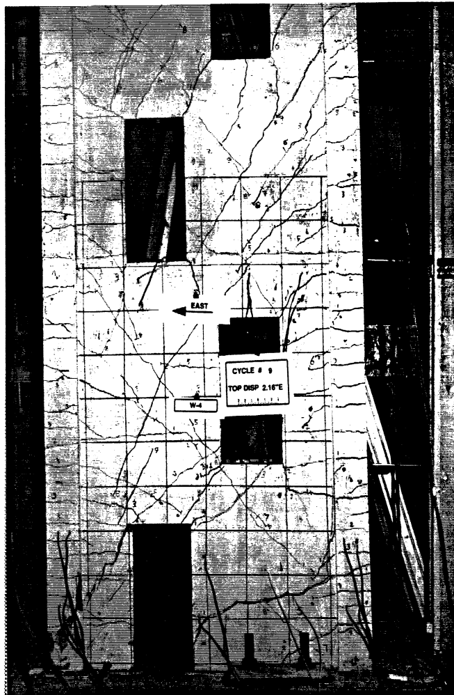
Fig. 4.35 : Shear Compression Failure of East Boundary Column in W-4 during
