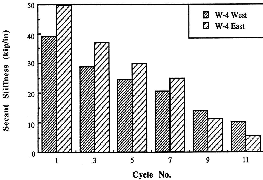
Fig. 4.44 : Comparison of Secant Stiffnesses for Wall W-4.
