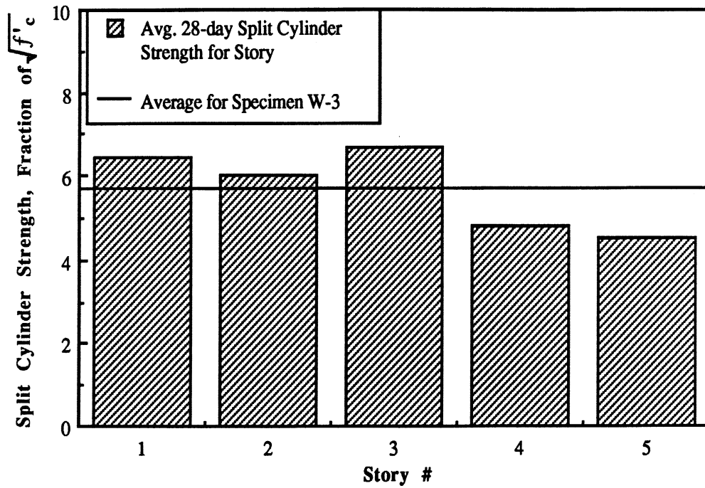
Fig. 3.18(c) : Variation of Concrete Split Cylinder Strength for Wall W-3.
