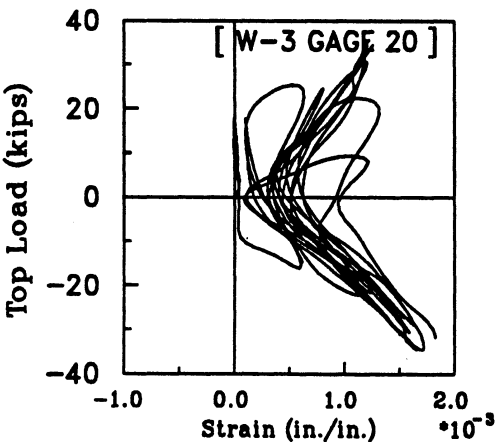
Fig. 4.72(c) : Strain Histories for Gages 16, 17, 18, 19, 20 and 21 in Wall W-3.
