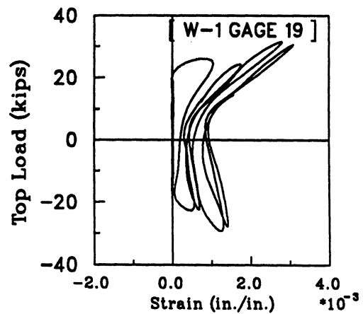
Fig. 4.70(c) : Strain Histories for Gages 14, 15, 16, 17, 18 and 19 in Wall W-1.
