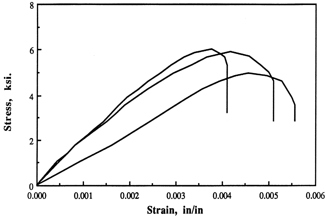
Fig. 3.20 : Stress-Strain Relationship for Concrete.
