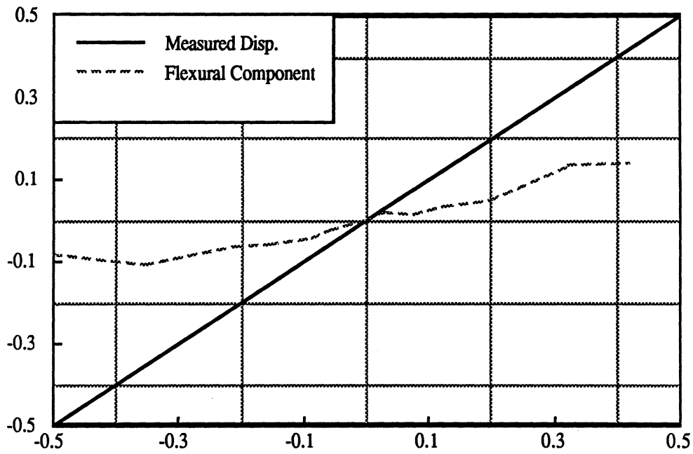
Fig. 4.61 : Flexural and Shear Components of First Story Displacement in W-4.
