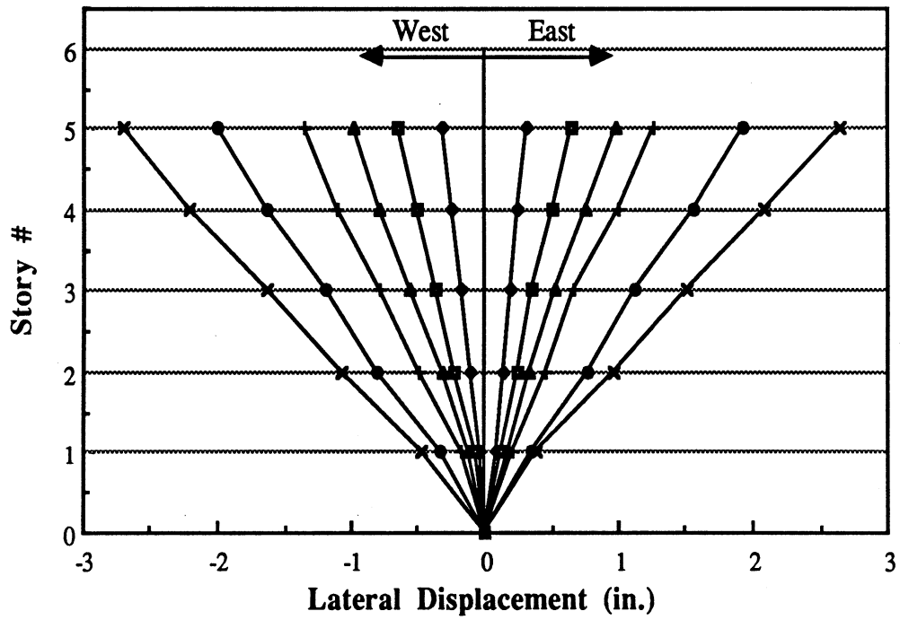
Fig. 4.54 : Displacement Profile along the Wall Height for W-2.
