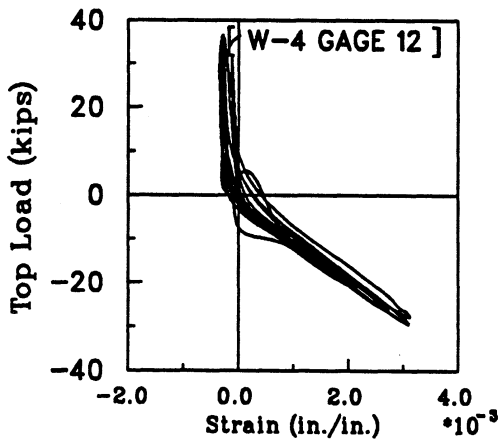
Fig. 4.73(b) : Strain Histories for Gages 8, 9, 10, 11, 12 and 14 in Wall W-4.
