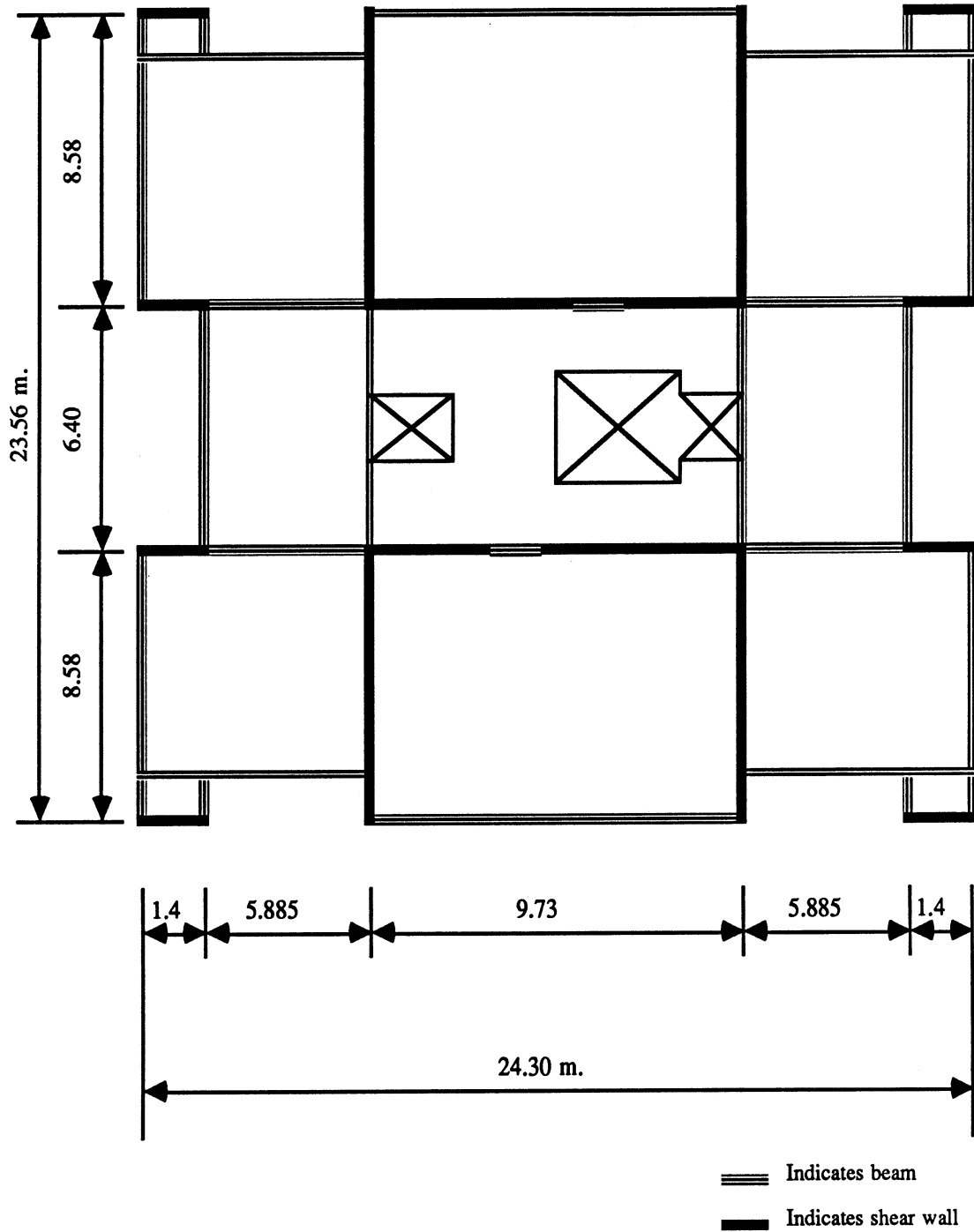
Fig 1.3(a) : Plan View of a Typical Story of Almendral Building.
