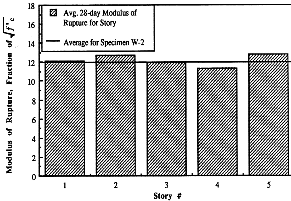
Fig. 3.19(b) : Variation of Concrete Modulus of Rupture for Wall W-2.
