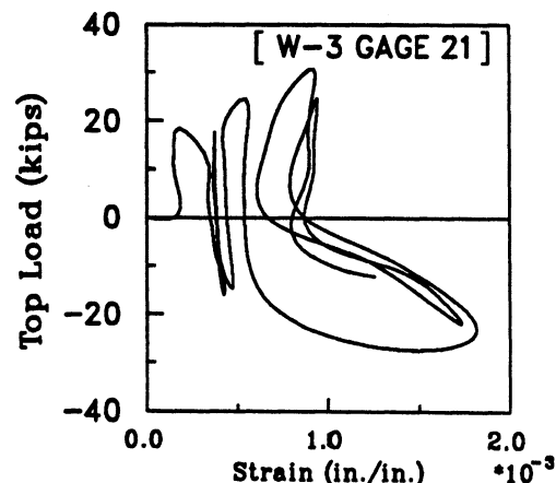
Fig. 4.72(c) : Strain Histories for Gages 16, 17, 18, 19, 20 and 21 in Wall W-3.
