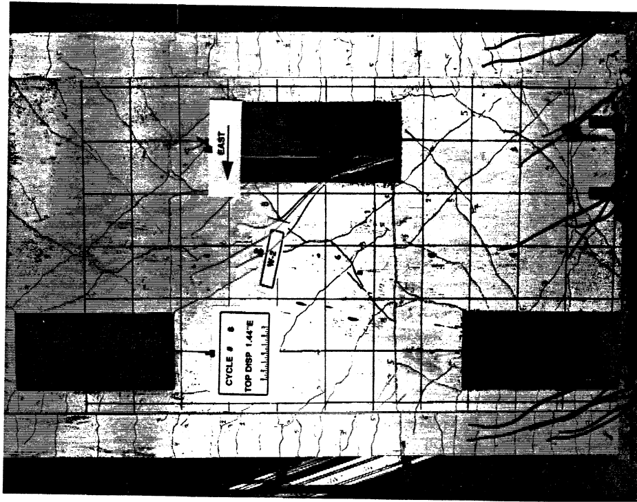
Fig. 4.13 : Compression Struts in the Lower Half of W-2 continue across the Joint during Cycle 8.
