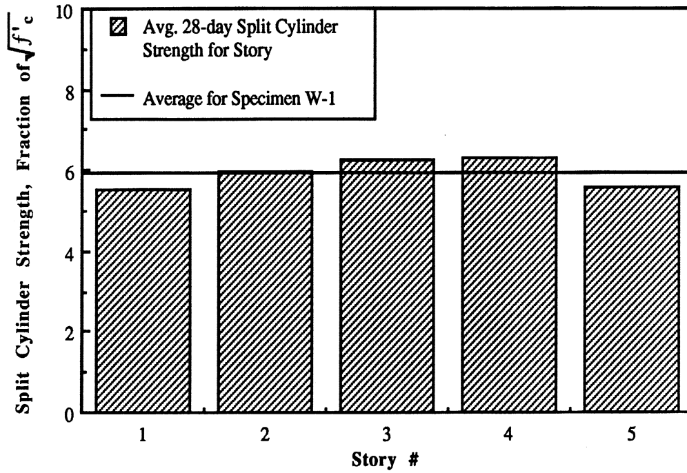
Fig. 3.18(a) : Variation of Concrete Split Cylinder Strength for Wall W-1.
