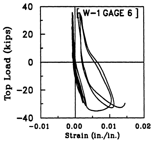
Fig. 4.70(a) : Strain Histories for Gages 1, 2, 3, 4, 6 and 7 in Wall W-1.
