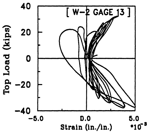
Fig. 4.70(b) : Strain Histories for Gages 8, 9, 10, 12, 13 and 14 in Wall W-2.
