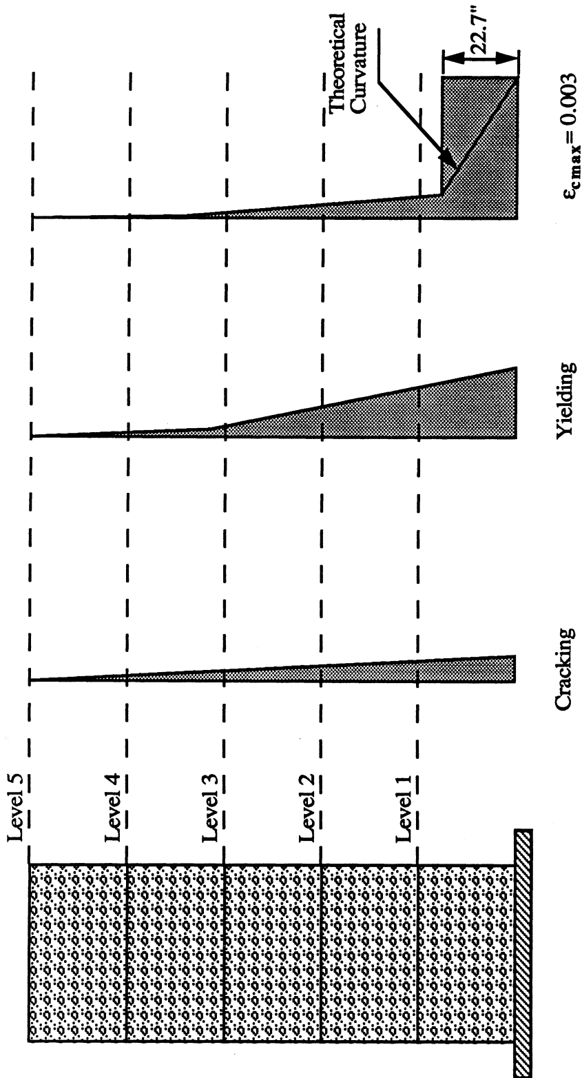
Fig. 5.5(a) : Actual and Effective Curvature Distributions for Wall Specimens at Cracking, Yielding and Nominal Strains.
