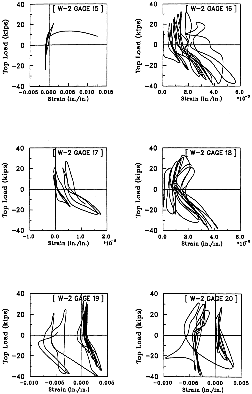
Fig. 4.71(c) : Strain Histories for Gages 15, 16, 17, 18, 19 and 20 in Wall W-2.
