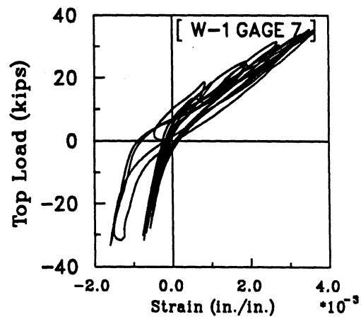
Fig. 4.70(a) : Strain Histories for Gages 1, 2, 3, 4, 6 and 7 in Wall W-1.
