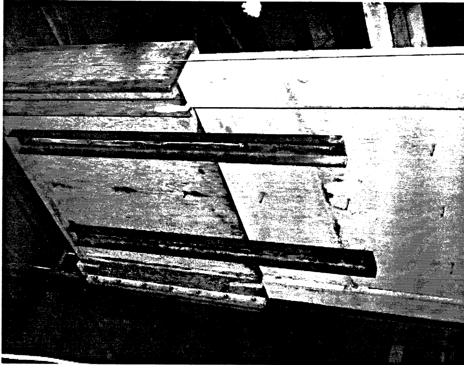
Fig. 3.9 : Wall W-1 under Construction.
