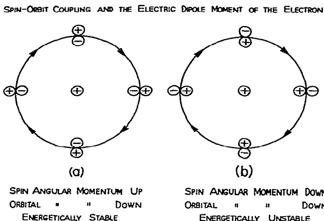
Fig 1 An illustration of spin-orbit coupling for an electron in the field of a positive charge in terms of the relativistic electric dipole moment of the electron (eqn. (11)). The positive charge is at the center of the circle and the motion is taken clockwise for (a) spin angular momentum up, electric moment pointing away from nucleus and (b) spin angular momentum down, electric moment pointing toward nucleus. The electron charge is not shown, only the dipole moment.
