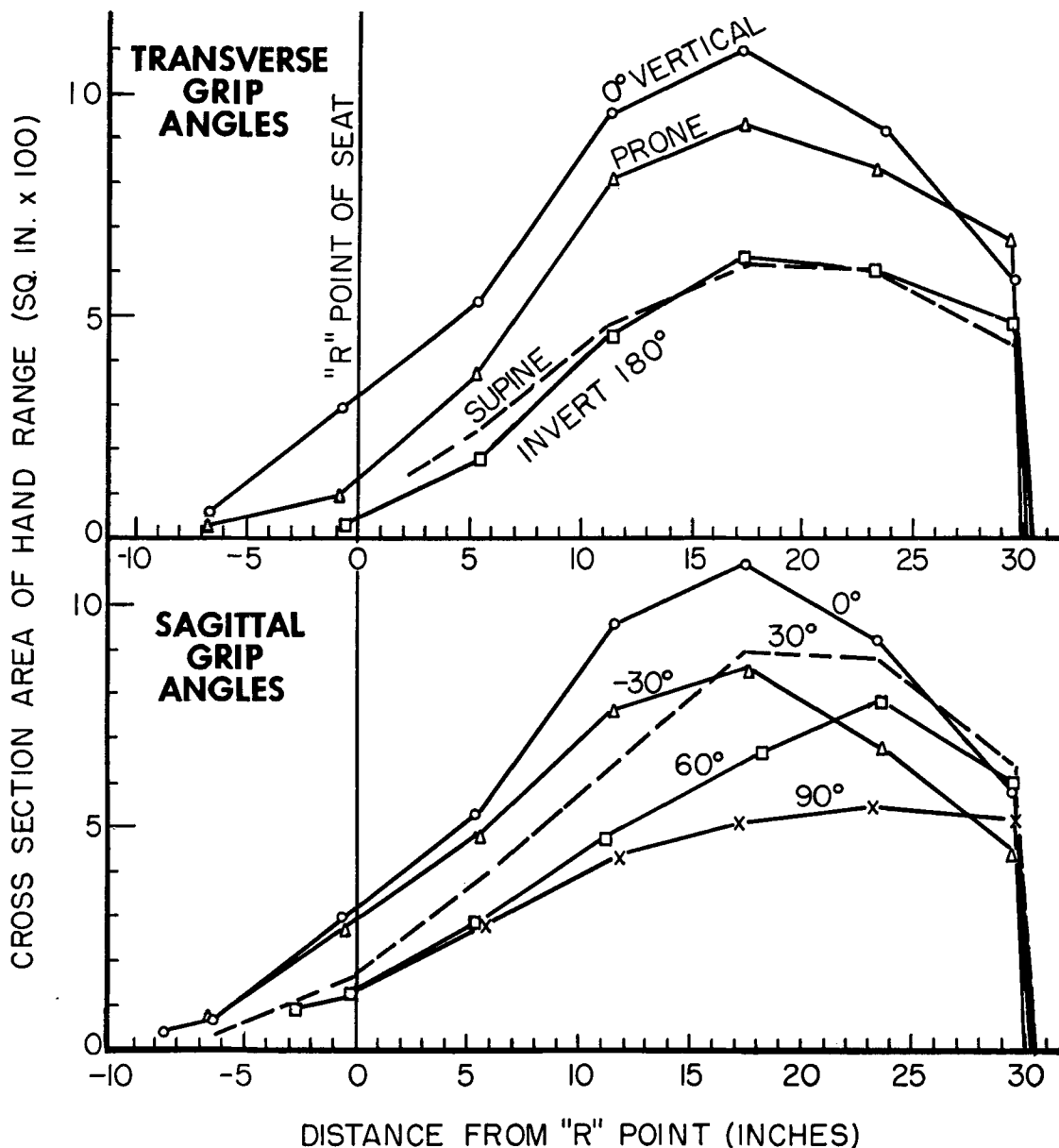
Fig. 5 Two series of plots showing the panel area available to the grip point of the left hand for transverse planes at different distances from the "R" point of the seat.
