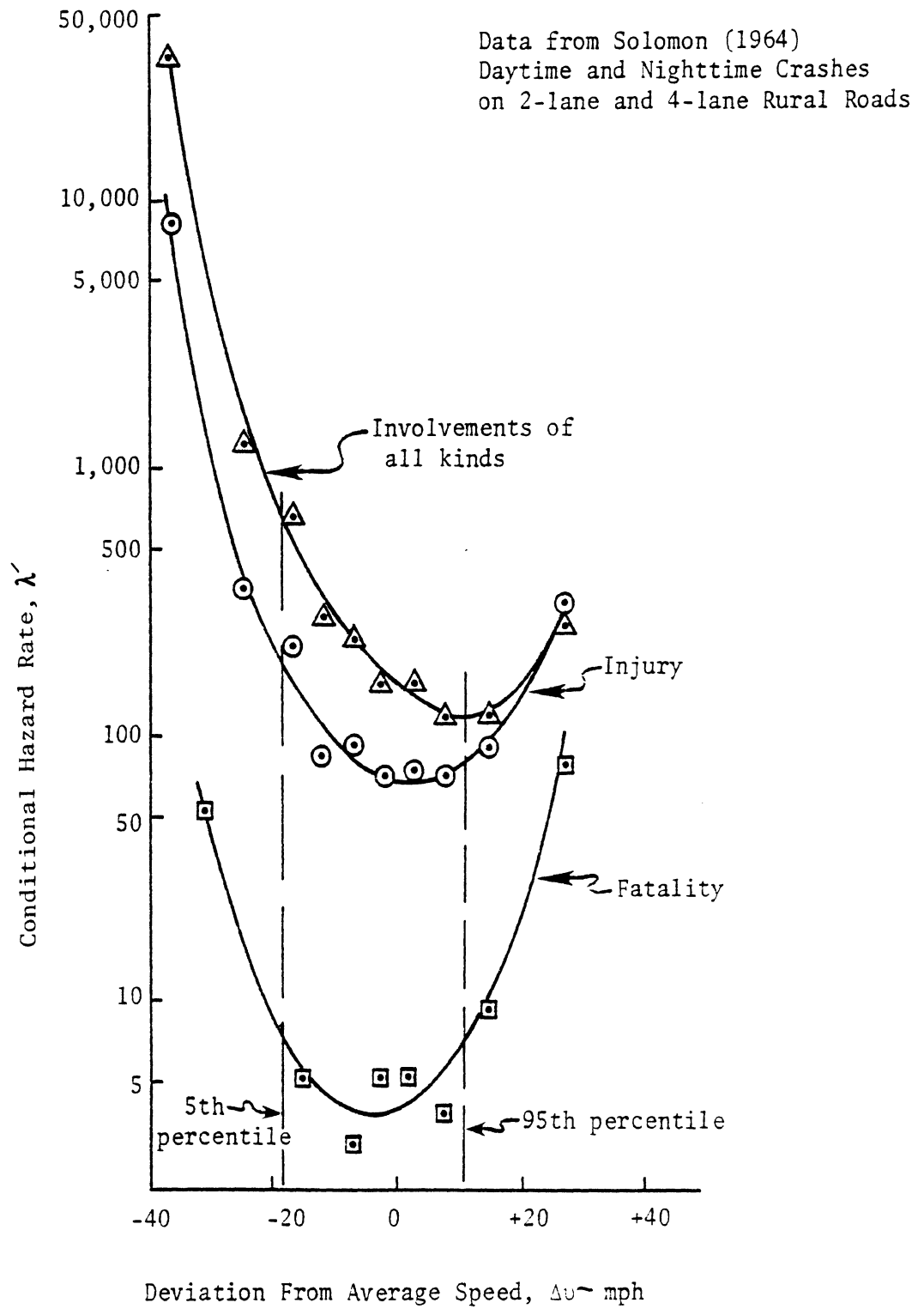
FIGURE 2-5 CONDITIONAL HAZARD RATES VERSUS SPEED DEVIATION FROM AVERAGE SPEED
