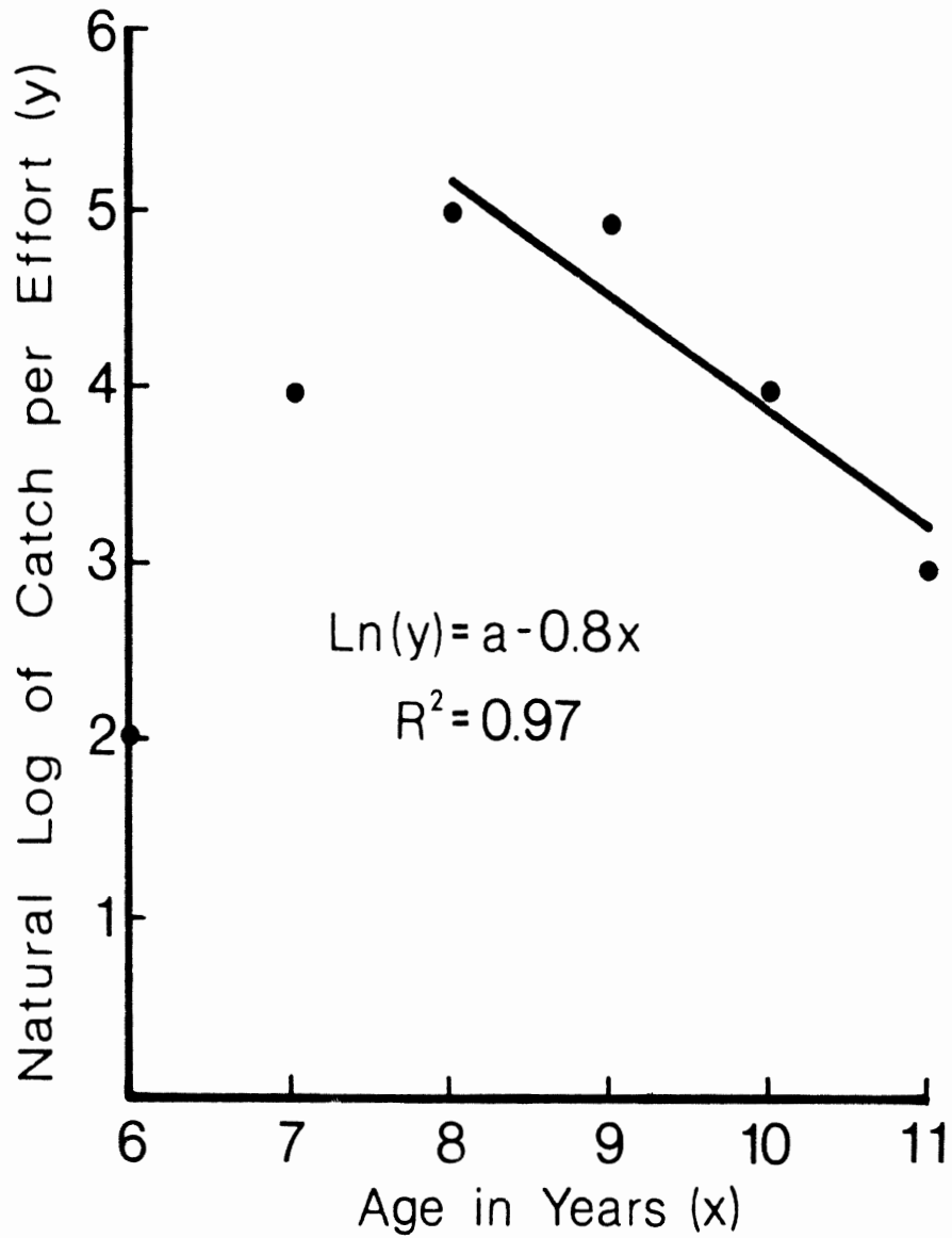
Figure 3.--Catch curve for northern Isle Royale whitefish collected with gill nets.
