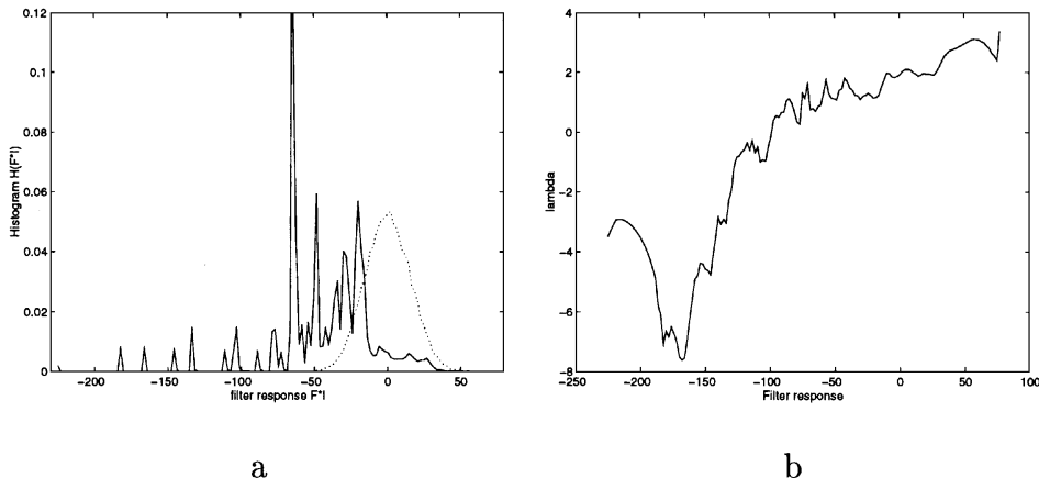
Figure 13. (a) The solid curve is the histogram of the circle image, and the dotted curve is the histogram of the noise image, and (b) the estimated \lambda(\cdot) function in the probability model for the image of circles.
