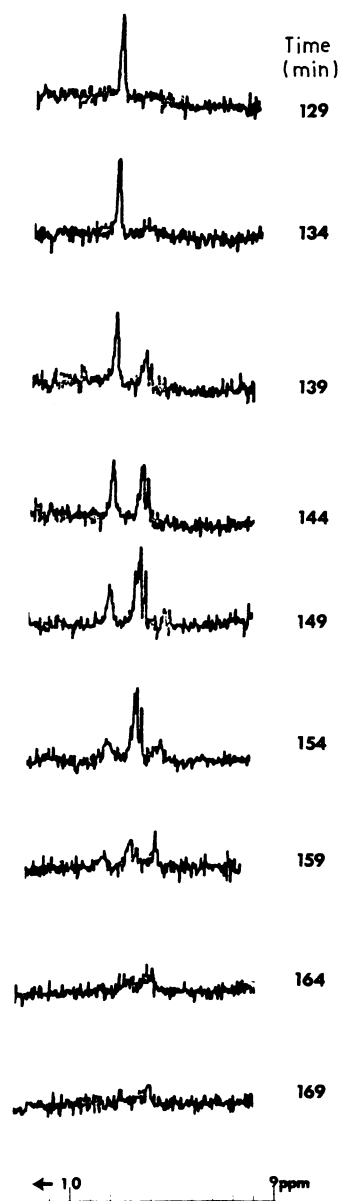
Fig. 2. FT proton NMR spectra of 4-hydroxycyclophosphamide in \text{CDCl}_3 between 9–10 ppm downfield from TMS at 15^\circ\text{C} .
