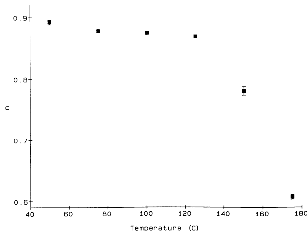
Fig. 5. The aging temperature dependence of the coupling parameter for cellulose acetate; time = 3 hr. The parameters were obtained from the fits of the converted mechanical relaxation data. (See text.) Error bars represent standard error of the mean.
