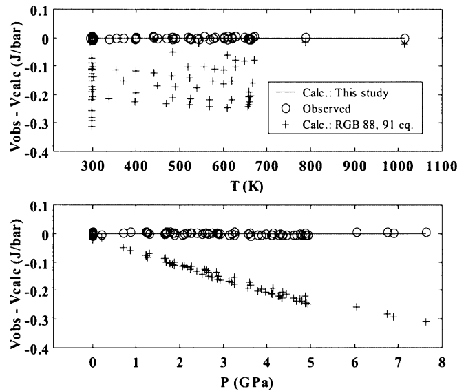
Fig. 5 ( V_{\text{obs}} - V_{\text{calc}} ) vs. T , and P plots. Use of the Holland and Powell (1990, 1998) volume equations produces similar results to the Berman (1998, 1991) equation
