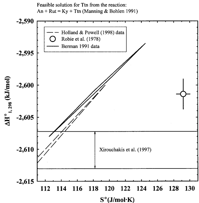
Fig. 6 Feasible solution for the reaction: anorthite + rutile = titanite + kyanite calculated using the internally consistent data bases of Berman (1991) and Holland and Powell (1998)
