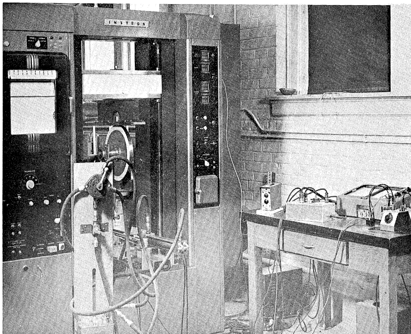
Figure 9. Test arrangement of Instron testing machine.
