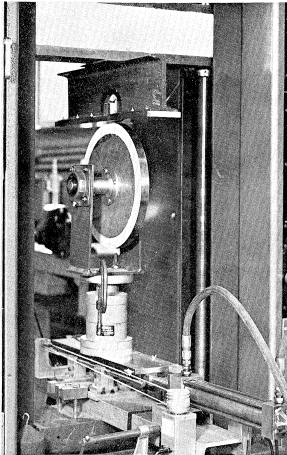
Figure 8. Test arrangement of Instron testing machine.
