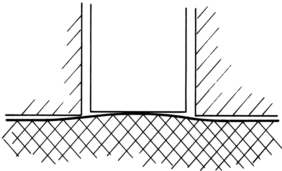
Figure 5. Detailed view of probable "bridging" action across pressure transducer.
