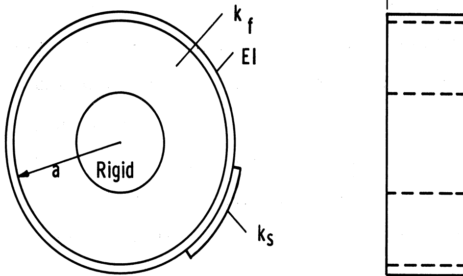
Figure 1. Shell model geometry.
