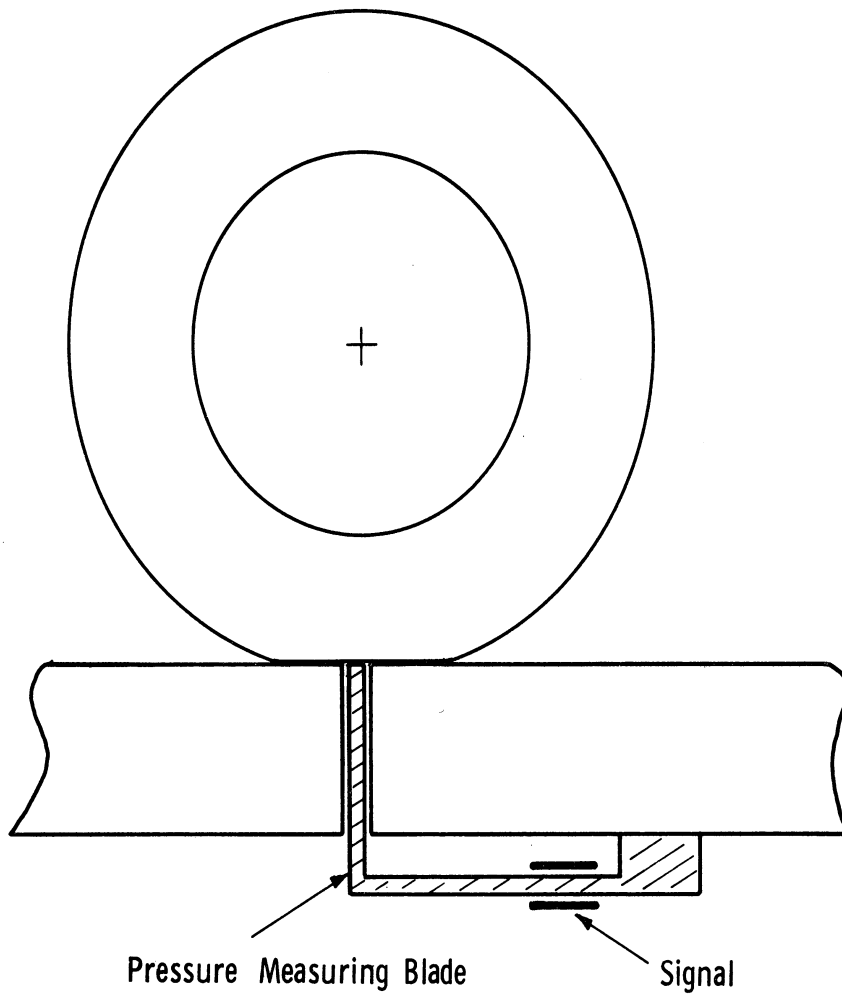
Figure 4. Cross section of pressure measuring area.
