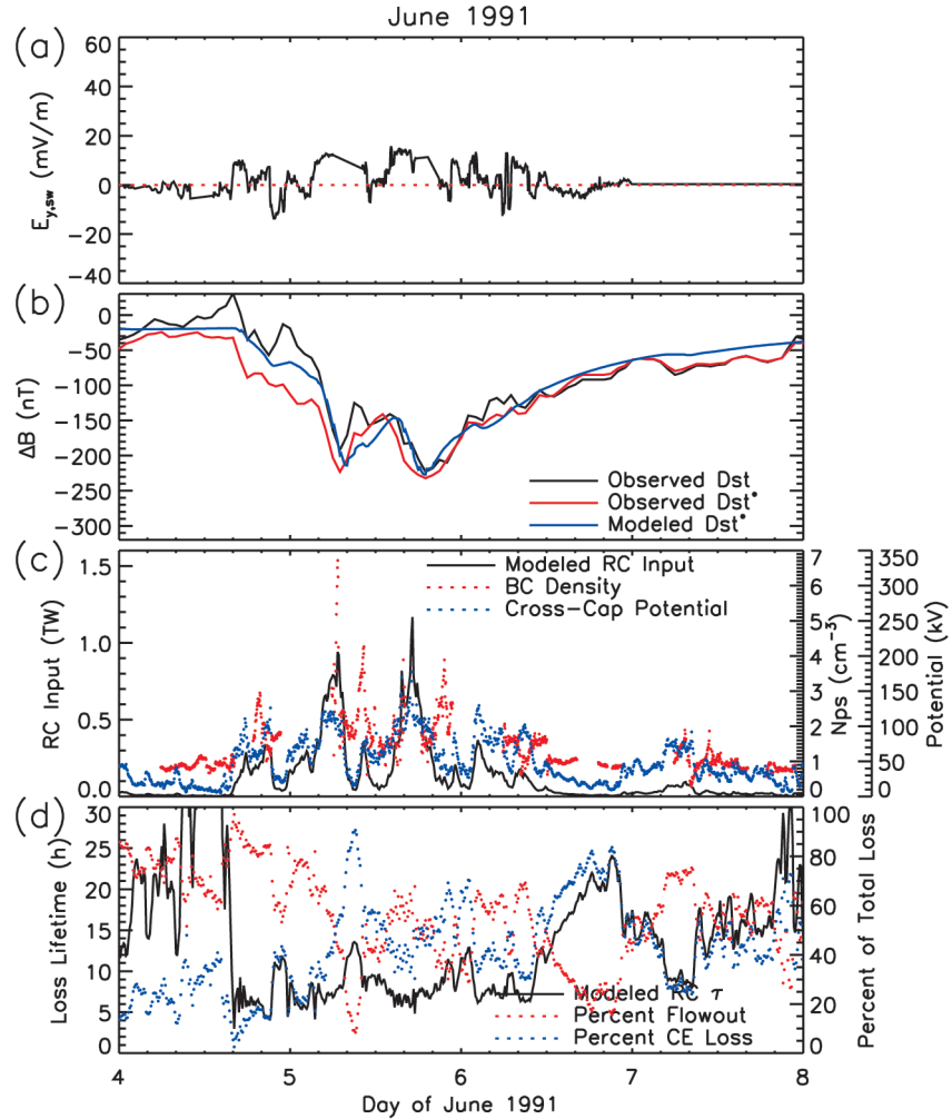
Figure 1. Simulation results for the 4–7 June 1991 magnetic storm. The solar wind E_y that triggered the storm is shown in the top panel. The modeled Dst^* (blue line) is compared to the observed Dst (black line) and observed Dst^* (red line) in the second panel. The energy input through the nightside outer boundary ( L = 6.75 ) of the model is plotted in the third panel (black line). This energy influx is constructed from observations of the plasma density at geosynchronous orbit (red dots) flowing inward with E \times B velocity which is a function of the cross polar cap potential, \Delta\Phi_{PC} (blue dots). The globally-average loss lifetime for the ring current is plotted in the bottom panel (black line) along with percentage of loss due to charge exchange (blue dots) and flow-out (red dots).
