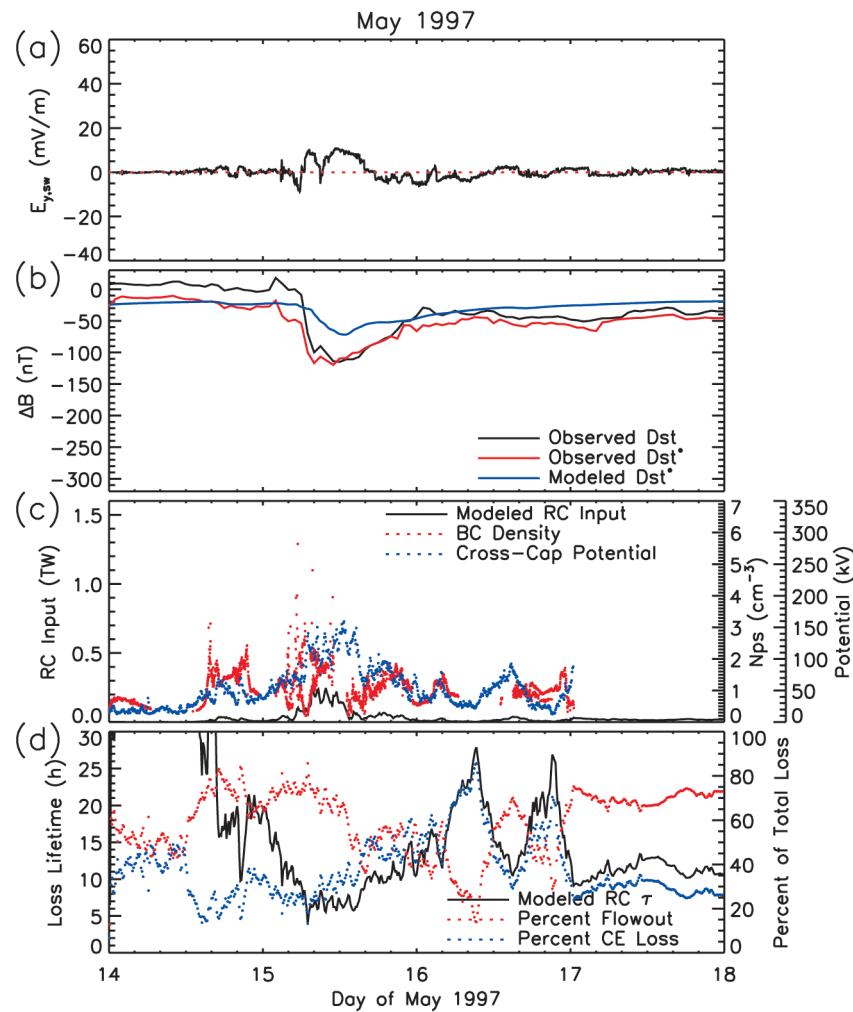
Figure 2. Simulation results for the 14–17 May 1997 magnetic storm in the same format as Figure 1.
