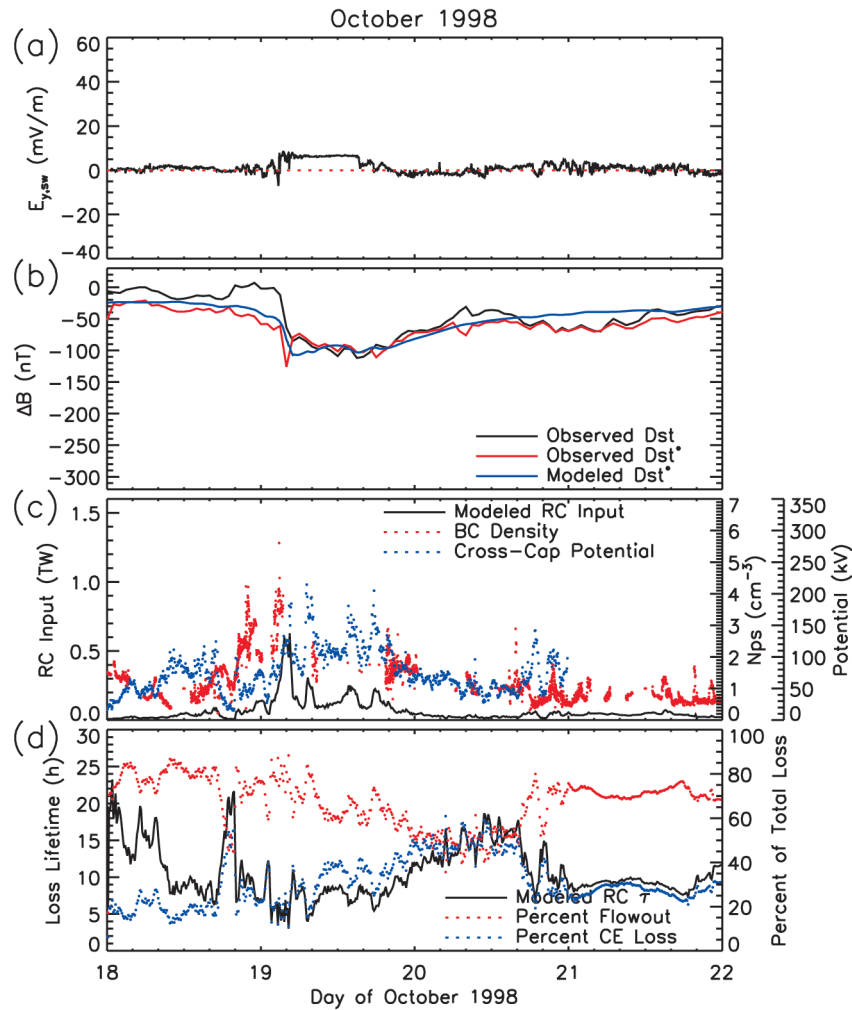
Figure 4. Simulation results for the 18–21 October 1998 magnetic storm in the same format as Figure 1.
