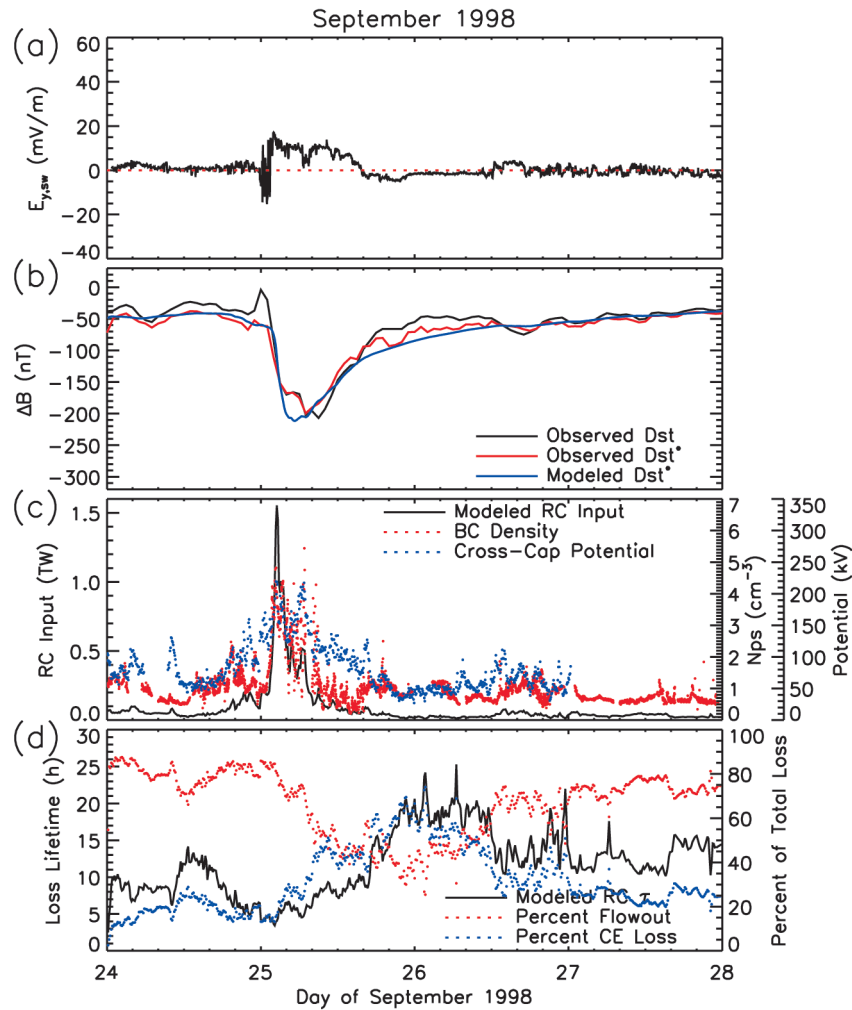
Figure 3. Simulation results for the 24–27 September 1998 magnetic storm in the same format as Figure 1.
