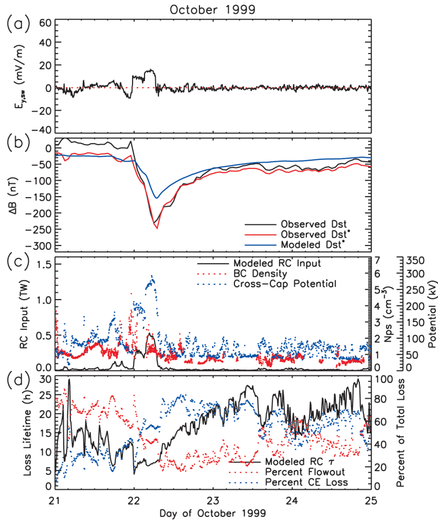
Figure 5. Simulation results for the 21–24 October 1999 magnetic storm in the same format as Figure 1.
