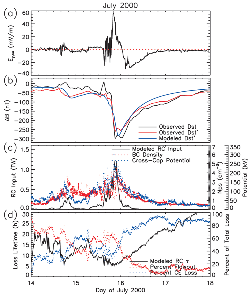
Figure 8. Simulation results for the 14–17 July 2000 magnetic storm in the same format as Figure 1.
