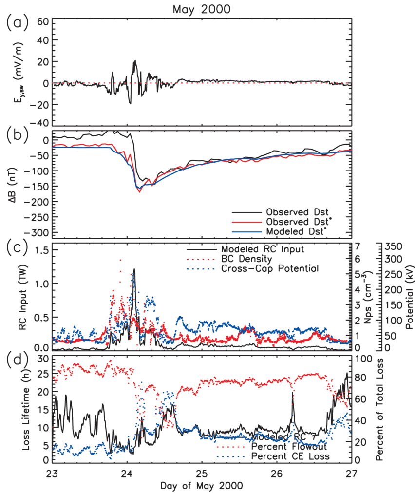
Figure 7. Simulation results for the 23–26 May 2000 magnetic storm in the same format as Figure 1.
