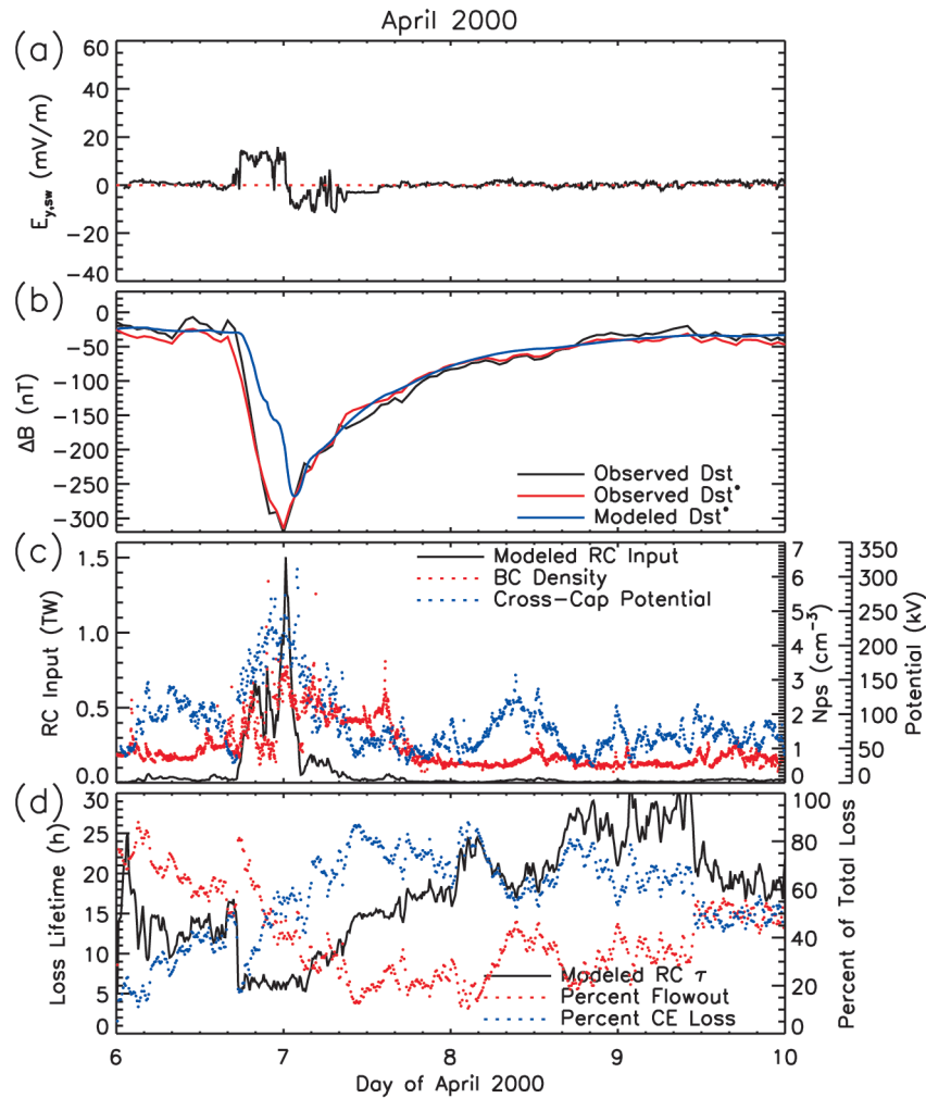
Figure 6. Simulation results for the 6–9 April 2000 magnetic storm in the same format as Figure 1.
