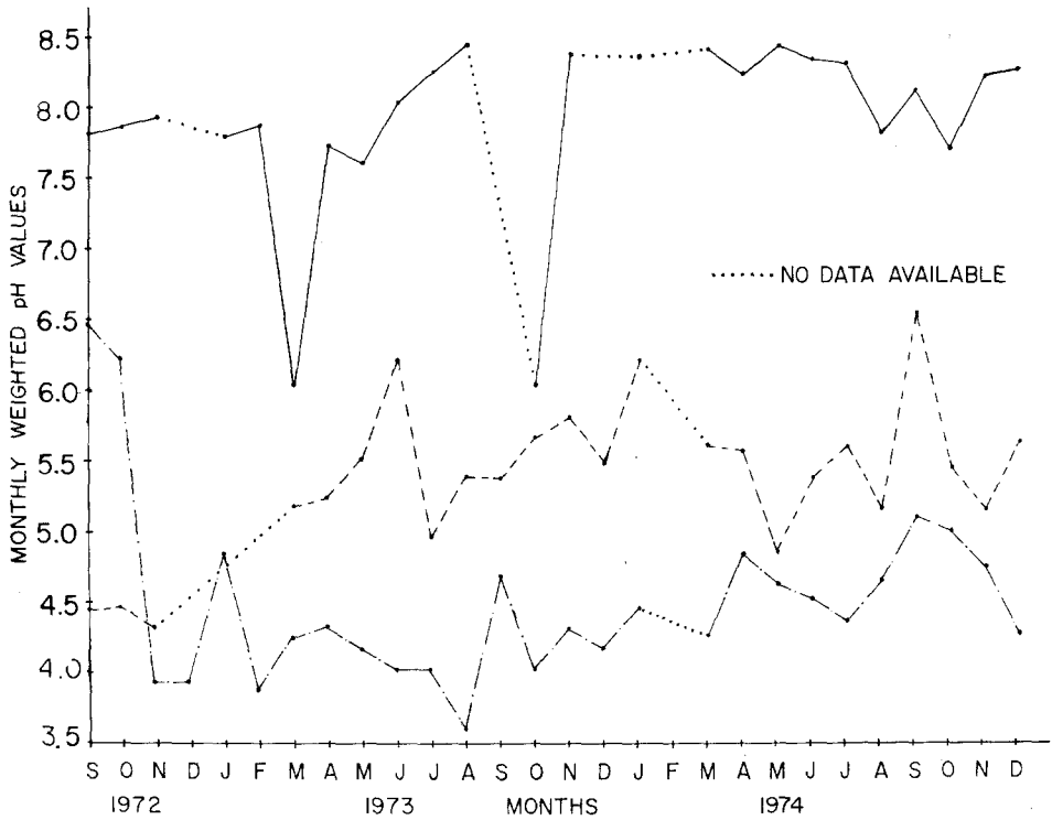
Fig. 2. Seasonal trends (1972-74) in weighted monthly pH values for three stations in Michigan (Reed City ---, Dimondale —, and Vassar —·—·—).
