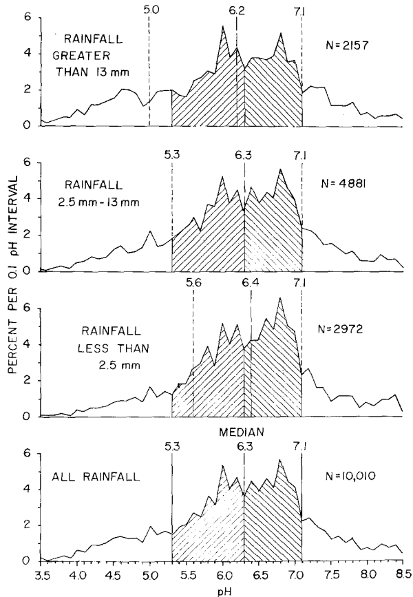
Fig. 4. Frequency distribution of pH values for three depths of rainfall. The median pH value \pm 33\% is shown for the entire state by solid lines and hatching. Dashed lines indicate median station pH values (—) and the 83.3 and 16.7 percentile (---), respectively. (Note median = 50 percentile, 50 + 33.3 = 83.3 , 50 - 33.3 = 16.7 .)
