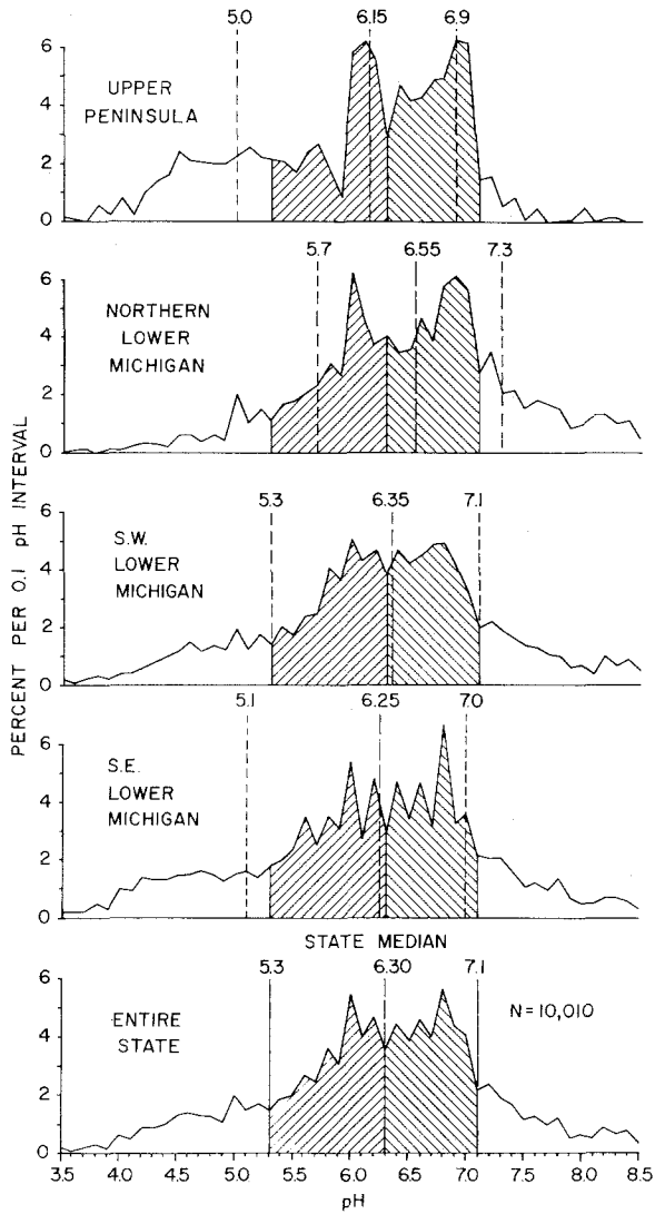
Fig. 1. Frequency distribution by region for pH values collected in Michigan (1972-74) from 60 selected stations. The median pH value ( \pm 33\% ) is shown for the entire state by solid lines and hatching. Dashed lines indicate regional pH median values (—) and 83.3 and 16.7 percentile (---), respectively. (Note median = 50 percentile, 50 + 33.3 = 83.3 , 50 - 33.3 = 16.7 .)
