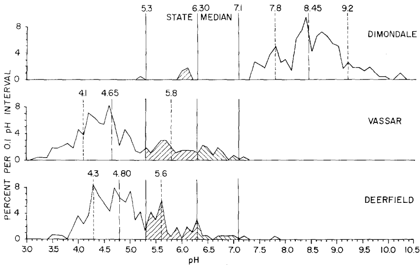
Fig. 3. Frequency distribution of pH values for selected stations in Michigan. The median pH value \pm 33% is shown for the entire state by solid lines and hatching. Dashed lines indicate median station pH values (—) and the 83.3 and 16.7 percentile (---), respectively. (Note median=50 percentile, 50 + 33.3 = 83.3 , 50 - 33.3 = 16.7 .)
