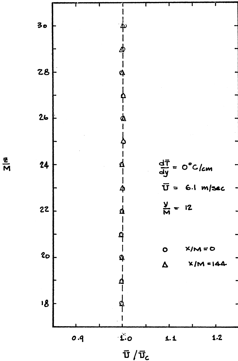
Fig. 13. Lateral (or horizontal) mean velocity distribution.
