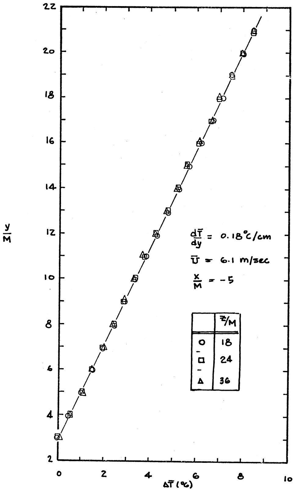
Fig. 18. Two - dimensionality of vertical mean temperature distribution
