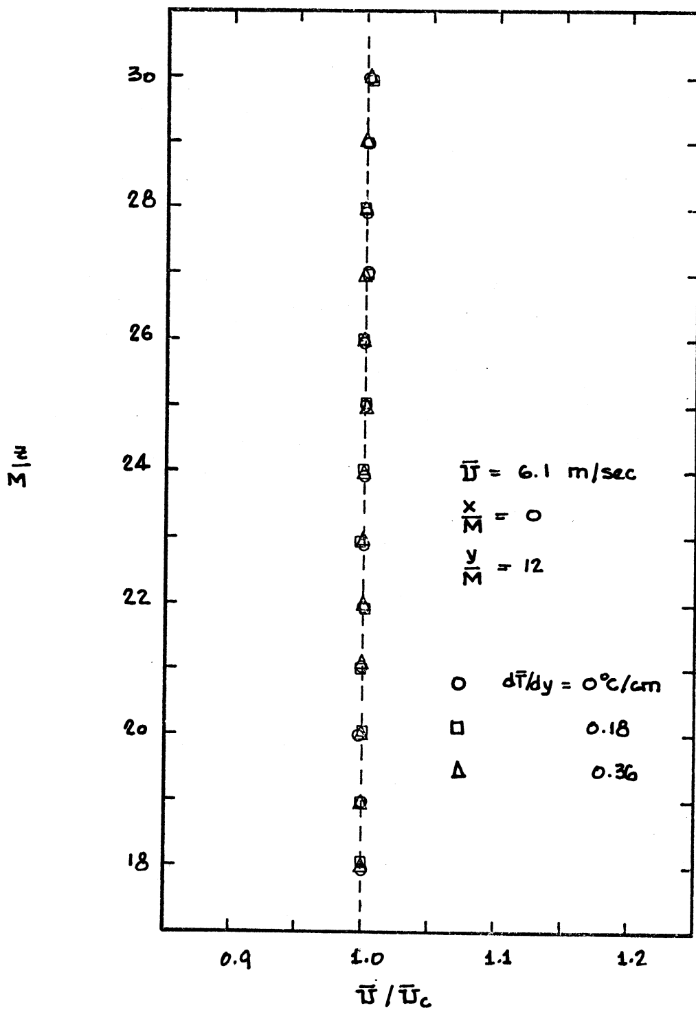
Fig. 22. Temperature effect upon lateral mean velocity distribution
