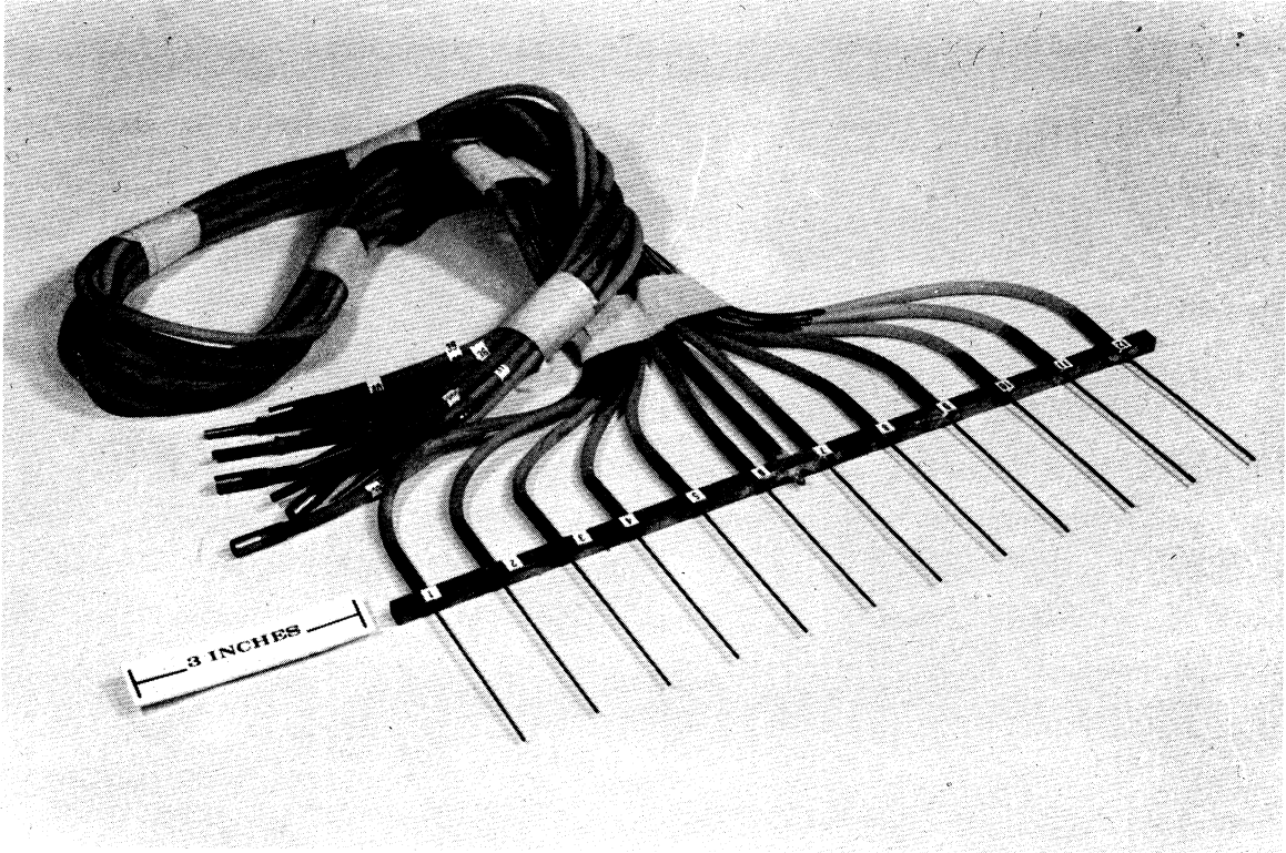
Fig. 12. Impact tube rake for measuring the free-stream velocity distribution in the wind tunnel.
