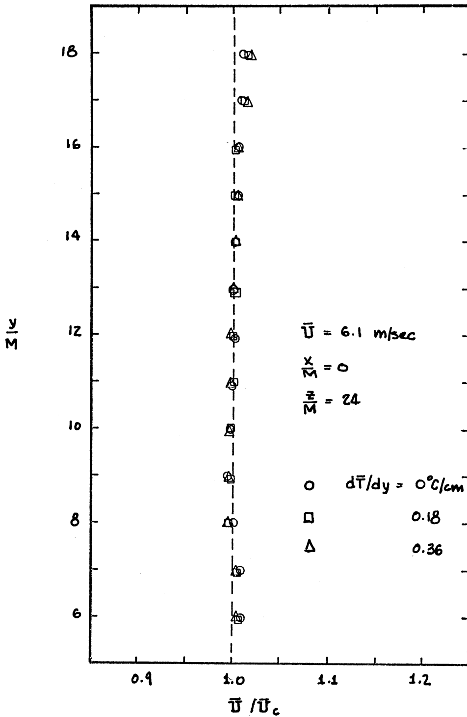
Fig. 21. Temperature effect upon mean vertical velocity distribution
