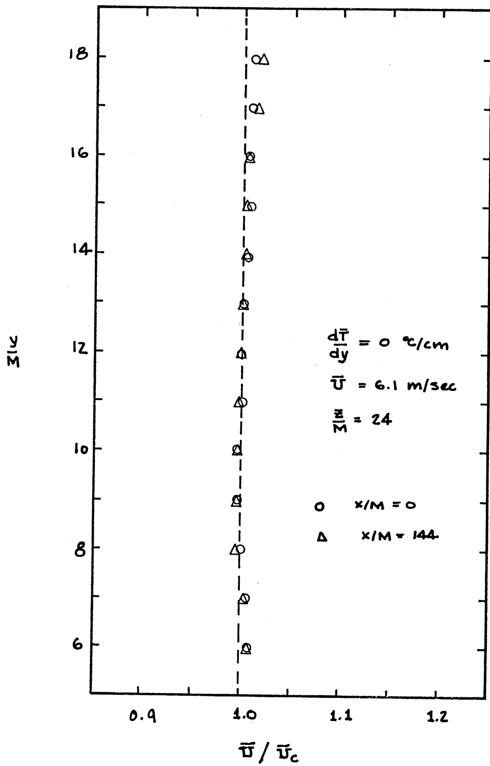
Fig. 11. Vertical mean velocity distribution.
