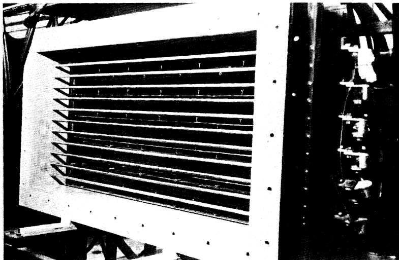
Fig. 4. Heater section showing method of support of elements by tension strips that are insulated from heating elements by glass tubing. One half inch brass rods to promote interfacial mixing can be seen.
