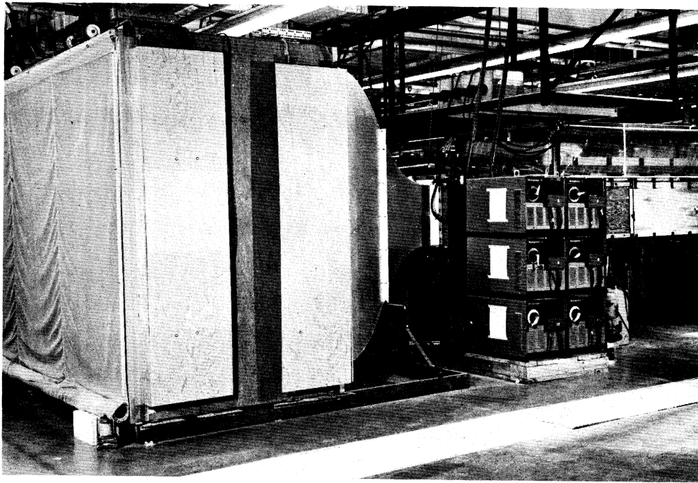
Fig. 2. Entrance, stilling and contraction sections. Six of the eleven welding transformers are also shown.
