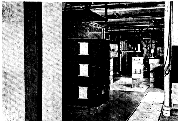
Fig. 10. View of support for temperature rake (at center of picture) showing guide channel and reference ice-bath. Cement block column supports channel in which a guide block slides. The guide block contains the thermocouple terminal strip and a guide pin to assure the position of the thermocouple rake when retracting it into the recesses in the sidewall of the wind tunnel. Covered mirror for shadowgraph visible on second, block column.
