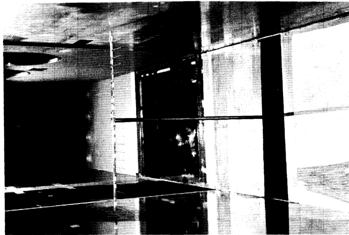
Fig. 9. Temperature rake for sensing the undisturbed temperature distribution. Rake retracts into wall. Shadowgraph window also is visible.
